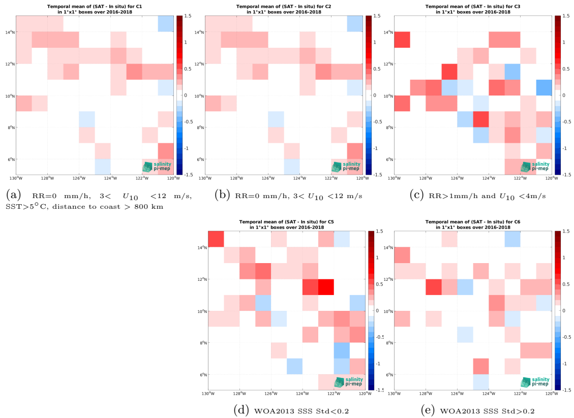
Figure 11: Temporal mean gridded over spatial boxes of size 1^\circ \times 1^\circ of \Delta\text{SSS} (CCI SSS L4 Merged-OI v3.2 - 7-day running (ESA) - Surface drifters) for 5 different subdatasets corresponding to:RR=0 mm/h, 3 < U_{10} < 12 m/s, SST >5^\circ\text{C} , distance to coast > 800 km (a), RR=0 mm/h, 3 < U_{10} < 12 m/s (b), RR >1 mm/h and U_{10} < 4 m/s (c), WOA2013 SSS Std <0.2 (d), WOA2013 SSS Std >0.2 (e).
