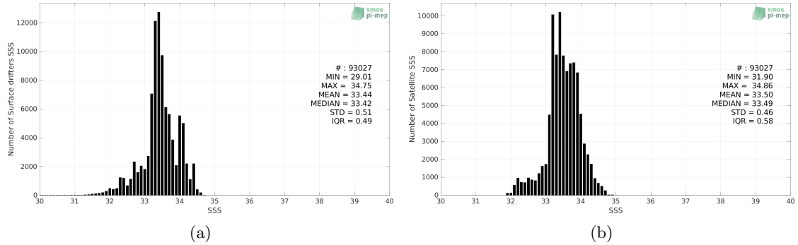
Figure 2: Histograms of SSS from Surface drifters (a) and CCI SSS L4 Merged-OI v3.2 - 7-day running (ESA) (b) considering all match-up pairs per bins of 0.1 over the SPURS 2 Pi-MEP region and for the full satellite product period.
