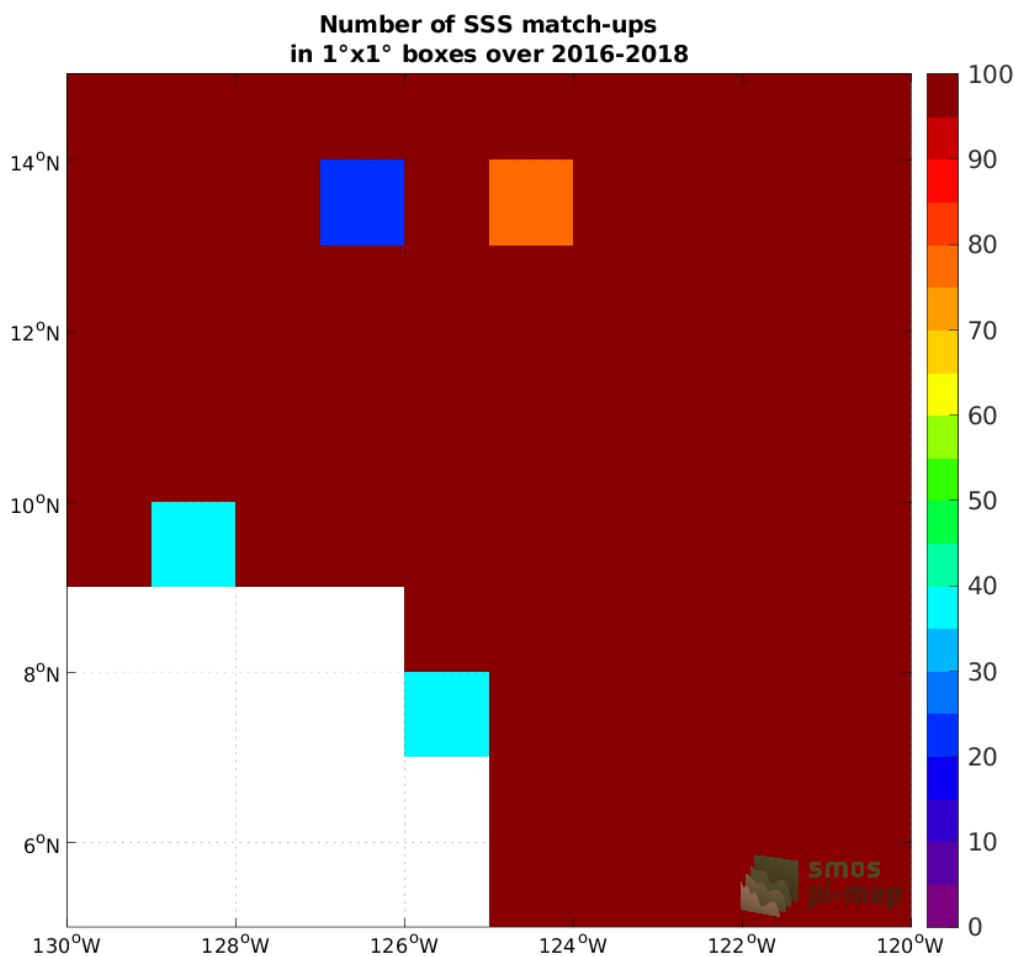
Figure 3: Number of SSS match-ups between Surface drifters SSS and the CCI SSS L4 Merged-OI v3.2 - 7-day running (ESA) SSS product for the SPURS 2 Pi-MEP region over 1°x1° boxes and for the full satellite product period.
