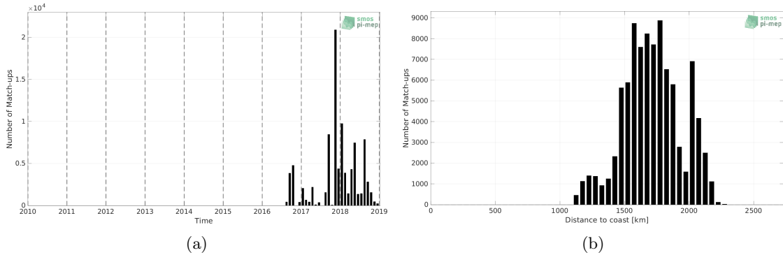
Figure 1: Number of match-ups between Surface drifters and CCI SSS L4 Merged-OI v3.2 - 7-day running (ESA) SSS as a function of time (a) and as function of the distance to coast (b) over the SPURS 2 Pi-MEP region and for the full satellite product period.
