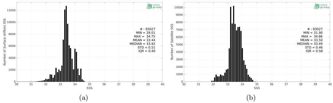
Figure 2: Histograms of SSS from Surface drifters (a) and CCI SSS L4 Merged-OI v3.2 - 7-day running (ESA) (b) considering all match-up pairs per bins of 0.1 over the SPURS 2 Pi-MEP region and for the full satellite product period.
