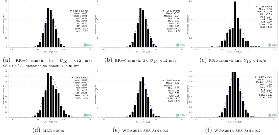
Figure 13: Normalized histogram of \Delta SSS (CCI SSS L4 Merged-OI v3.2 - 7-day running (ESA) - Argo) for 6 different subdatasets corresponding to: RR=0 mm/h, 3 < U_{10} < 12 m/s, SST>5°C, distance to coast > 800 km (a), RR=0 mm/h, 3 < U_{10} < 12 m/s (b), RR>1mm/h and U_{10} < 4 m/s (c), MLD<20m (d), WOA2013 SSS Std<0.2 (e), WOA2013 SSS Std>0.2 (f).
