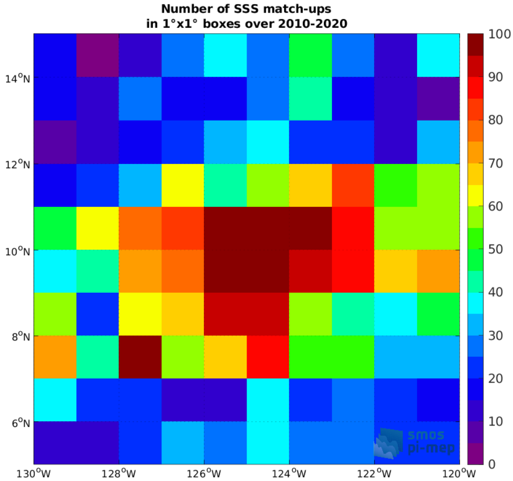
Figure 4: Number of SSS match-ups between Argo SSS and the CCI SSS L4 Merged-OI v3.2 - 7-day running (ESA) SSS product for the SPURS 2 Pi-MEP region over 1°x1° boxes and for the full satellite product period.
