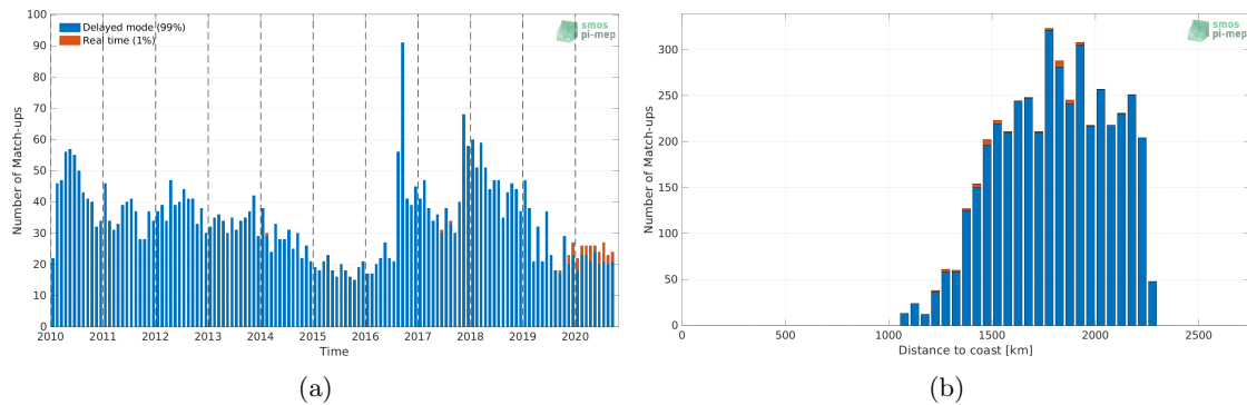
Figure 1: Number of match-ups between Argo and CCI SSS L4 Merged-OI v3.2 - 7-day running (ESA) SSS as a function of time (a) and as function of the distance to coast (b) over the SPURS 2 Pi-MEP region and for the full satellite product period.
