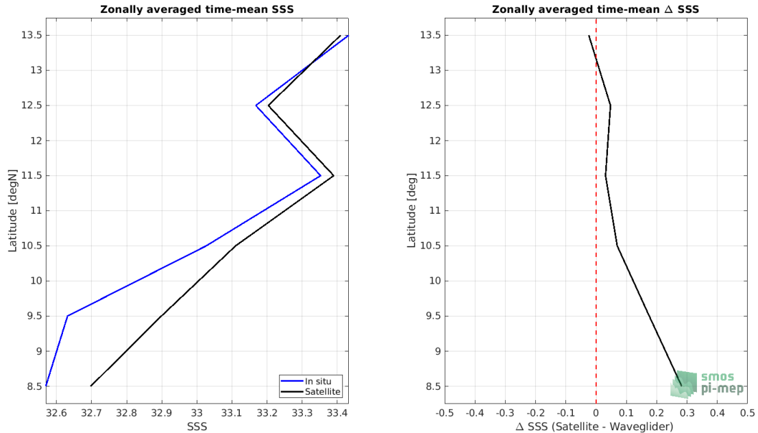
Figure 7: Left panel: Zonal mean SSS from CCI SSS L4 Merged-OI v3.2 - 30-day running (ESA) satellite product (black) and from Waveglider (blue). Right panel: Zonal mean of \Delta SSS (Satellite - Waveglider) for all the collected Pi-MEP match-up pairs estimated over the full satellite product period.
