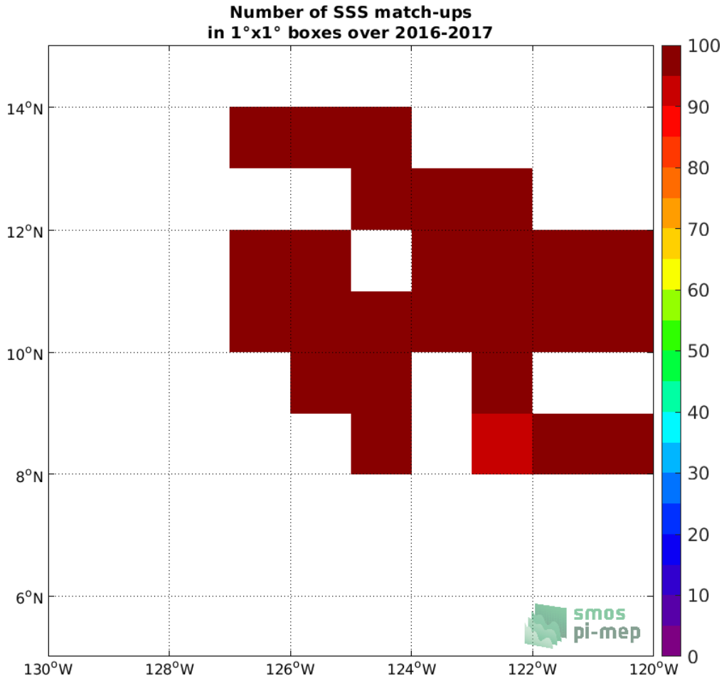
Figure 3: Number of SSS match-ups between Waveglider SSS and the CCI SSS L4 Merged-OI v3.2 - 30-day running (ESA) SSS product for the SPURS 2 Pi-MEP region over 1^\circ \times 1^\circ boxes and for the full satellite product period.
