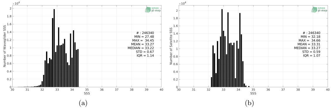
Figure 2: Histograms of SSS from Wavglider (a) and CCI SSS L4 Merged-OI v3.2 - 30-day running (ESA) (b) considering all match-up pairs per bins of 0.1 over the SPURS 2 Pi-MEP region and for the full satellite product period.
