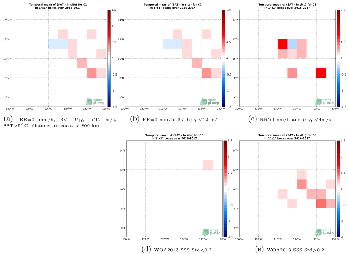
Figure 11: Temporal mean gridded over spatial boxes of size 1^\circ \times 1^\circ of \Delta SSS (CCI SSS L4 Merged-OI v3.2 - 30-day running (ESA) - Waveglider) for 5 different subdatasets corresponding to:RR=0 mm/h, 3 < U_{10} < 12 m/s, SST >5^\circ\text{C} , distance to coast > 800 km (a), RR=0 mm/h, 3 < U_{10} < 12 m/s (b), RR >1 mm/h and U_{10} < 4 m/s (c), WOA2013 SSS Std <0.2 (d), WOA2013 SSS Std >0.2 (e).
