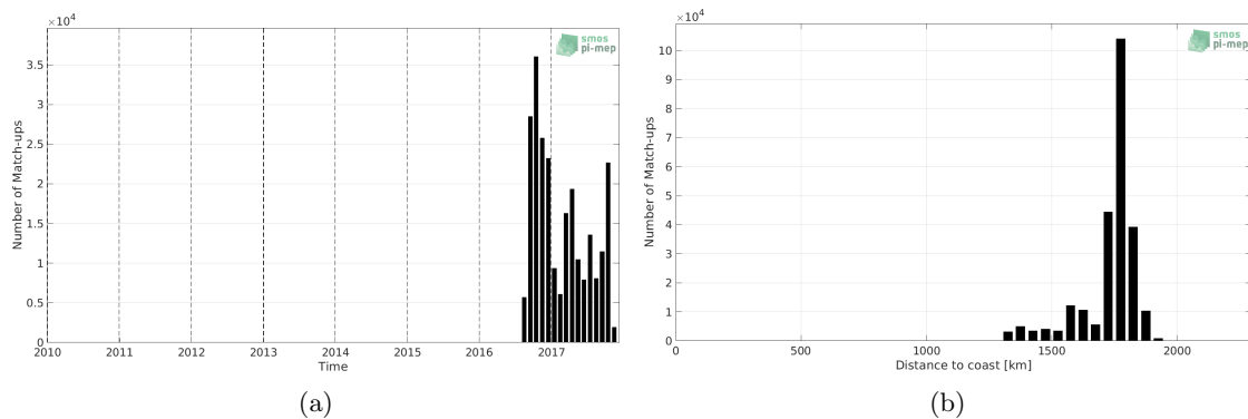
Figure 1: Number of match-ups between Waveglider and CCI SSS L4 Merged-OI v3.2 - 30-day running (ESA) SSS as a function of time (a) and as function of the distance to coast (b) over the SPURS 2 Pi-MEP region and for the full satellite product period.
