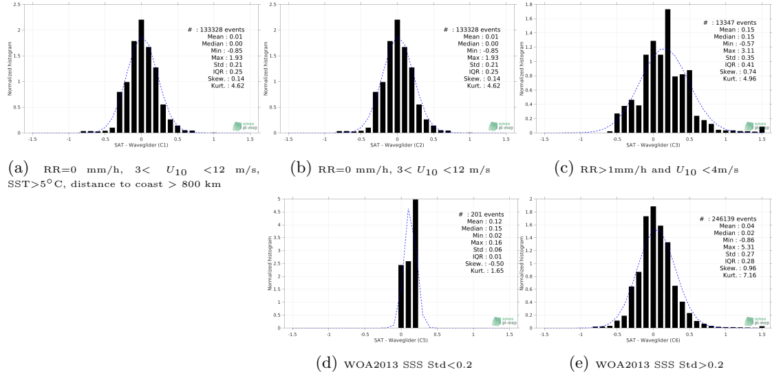
Figure 12: Normalized histogram of \Delta SSS (CCI SSS L4 Merged-OI v3.2 - 30-day running (ESA) - Waveglider) for 5 different subdatasets corresponding to: RR=0 mm/h, 3 < U_{10} < 12 m/s, SST > 5°C, distance to coast > 800 km (a), RR=0 mm/h, 3 < U_{10} < 12 m/s (b), RR > 1mm/h and U_{10} < 4 m/s (c), WOA2013 SSS Std < 0.2 (d), WOA2013 SSS Std > 0.2 (e).
