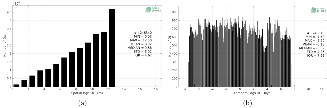
Figure 4: Histograms of the spatial (a) and temporal (b) lags between the location/time of the Waveglider measurement and the date of the corresponding CCI SSS L4 Merged-OI v3.2 - 30-day running (ESA) SSS pixel.
