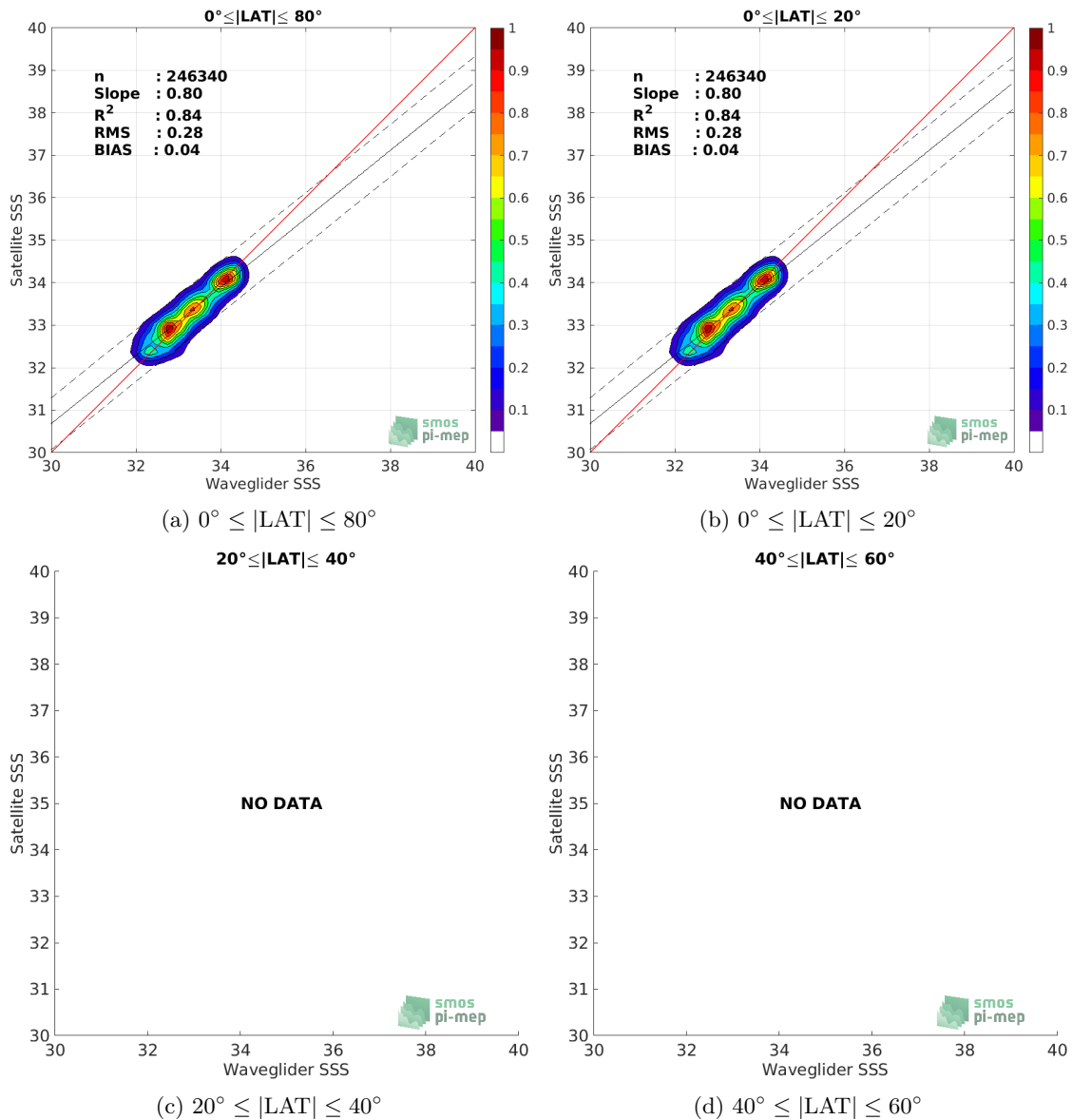
Figure 8: Contour maps of the concentration of CCI SSS L4 Merged-OI v3.2 - 30-day running (ESA) SSS (y-axis) versus Waveglider SSS (x-axis) at match-up pairs for different latitude bands. For each plot, the red line shows x=y . The black thin and dashed lines indicate a linear fit through the data cloud and the \pm 95\% confidence levels, respectively. The number match-up pairs n , the slope and R^2 coefficient of the linear fit, the root mean square (RMS) and the mean bias between satellite and in situ data are indicated for each latitude band in each plots.
