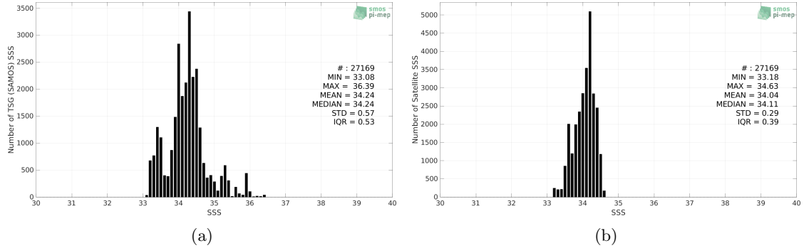
Figure 2: Histograms of SSS from TSG (SAMOS) (a) and CCI SSS L4 Merged-OI v3.2 - 30-day running (ESA) (b) considering all match-up pairs per bins of 0.1 over the SPURS 2 Pi-MEP region and for the full satellite product period.
