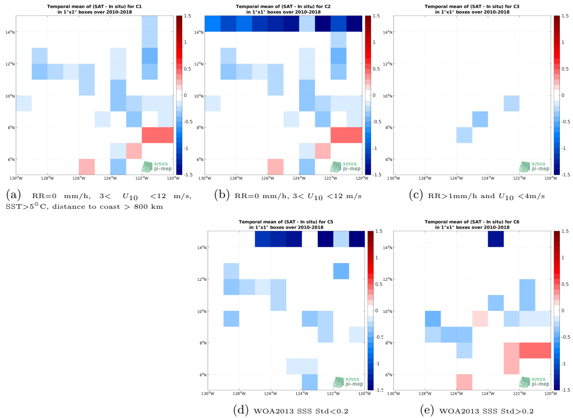
Figure 12: Temporal mean gridded over spatial boxes of size 1^\circ \times 1^\circ of \Delta\text{SSS} (CCI SSS L4 Merged-OI v3.2 - 30-day running (ESA) - TSG (SAMOS)) for 5 different subdatasets corresponding to:RR=0 mm/h, 3 < U_{10} < 12 m/s, SST >5^\circ\text{C} , distance to coast > 800 km (a), RR=0 mm/h, 3 < U_{10} < 12 m/s (b), RR >1 mm/h and U_{10} < 4 m/s (c), WOA2013 SSS Std <0.2 (d), WOA2013 SSS Std >0.2 (e).
