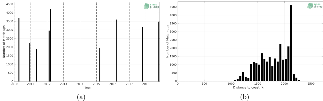
Figure 1: Number of match-ups between TSG (SAMOS) and CCI SSS L4 Merged-OI v3.2 - 30-day running (ESA) SSS as a function of time (a) and as function of the distance to coast (b) over the SPURS 2 Pi-MEP region and for the full satellite product period.
