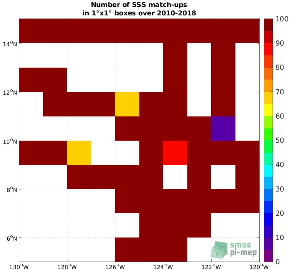
Figure 4: Number of SSS match-ups between TSG (SAMOS) SSS and the CCI SSS L4 Merged-OI v3.2 - 30-day running (ESA) SSS product for the SPURS 2 Pi-MEP region over 1^\circ \times 1^\circ boxes and for the full satellite product period.
