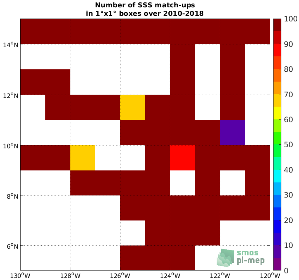
Figure 4: Number of SSS match-ups between TSG (SAMOS) SSS and the CCI SSS L4 Merged-OI v3.2 - 30-day running (ESA) SSS product for the SPURS 2 Pi-MEP region over 1°x1° boxes and for the full satellite product period.
