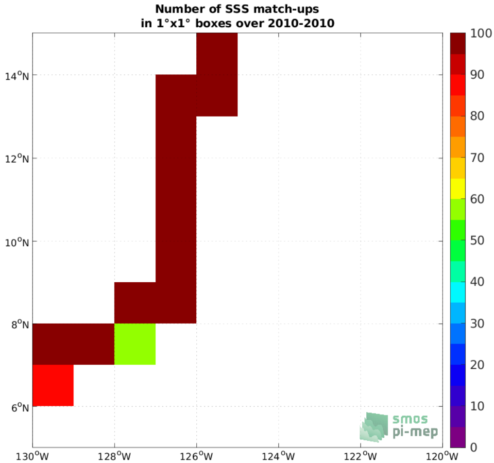
Figure 4: Number of SSS match-ups between TSG (GOSUD-Sailing-ship) SSS and the CCI SSS L4 Merged-OI v3.2 - 30-day running (ESA) SSS product for the SPURS 2 Pi-MEP region over 1^\circ \times 1^\circ boxes and for the full satellite product period.
