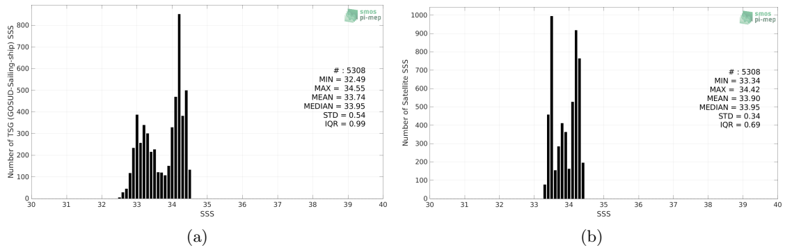
Figure 2: Histograms of SSS from TSG (GOSUD-Sailing-ship) (a) and CCI SSS L4 Merged-OI v3.2 - 30-day running (ESA) (b) considering all match-up pairs per bins of 0.1 over the SPURS 2 Pi-MEP region and for the full satellite product period.
