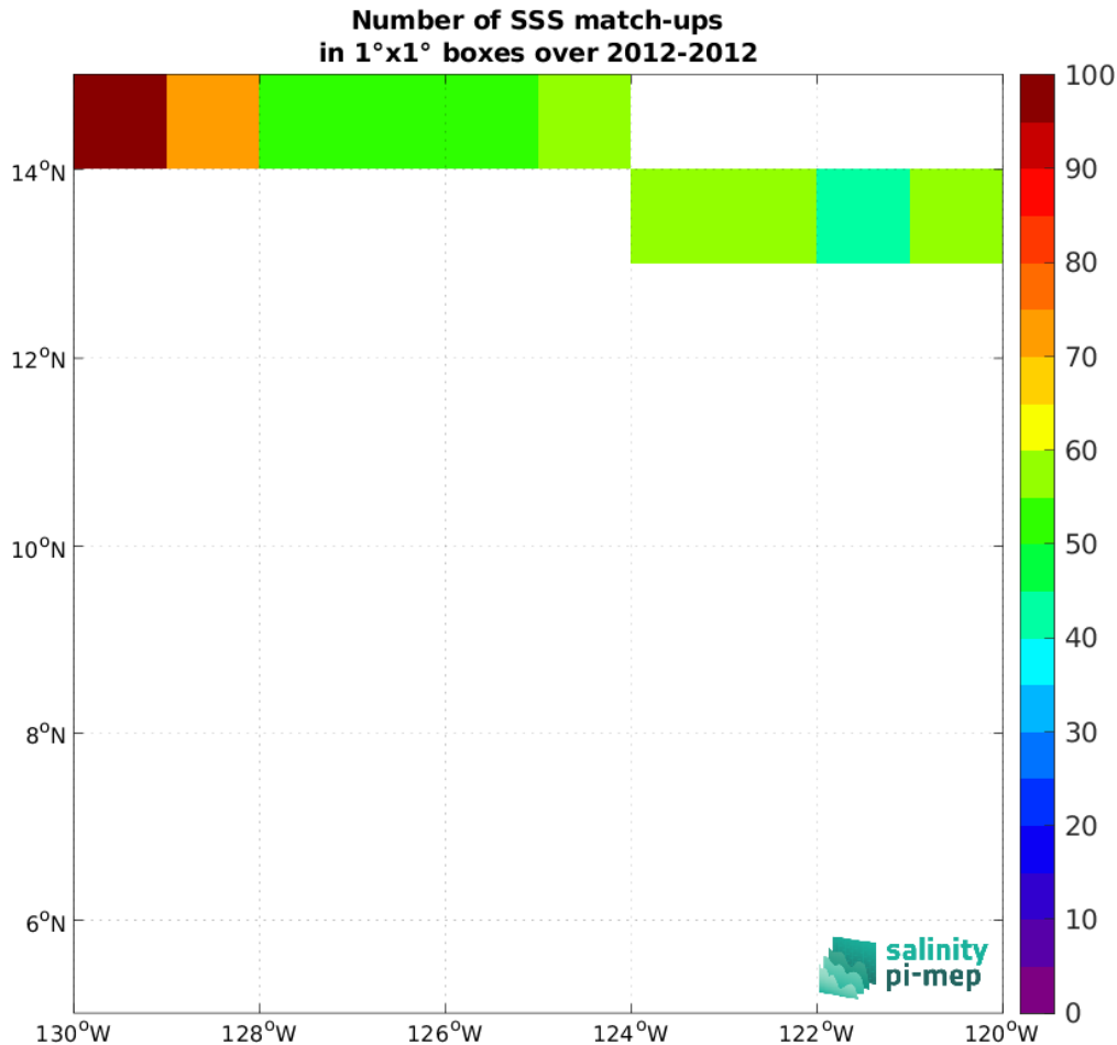
Figure 4: Number of SSS match-ups between TSG (GOSUD-Research-vessel) SSS and the CCI SSS L4 Merged-OI v3.2 - 30-day running (ESA) SSS product for the SPURS 2 Pi-MEP region over 1^\circ \times 1^\circ boxes and for the full satellite product period.
