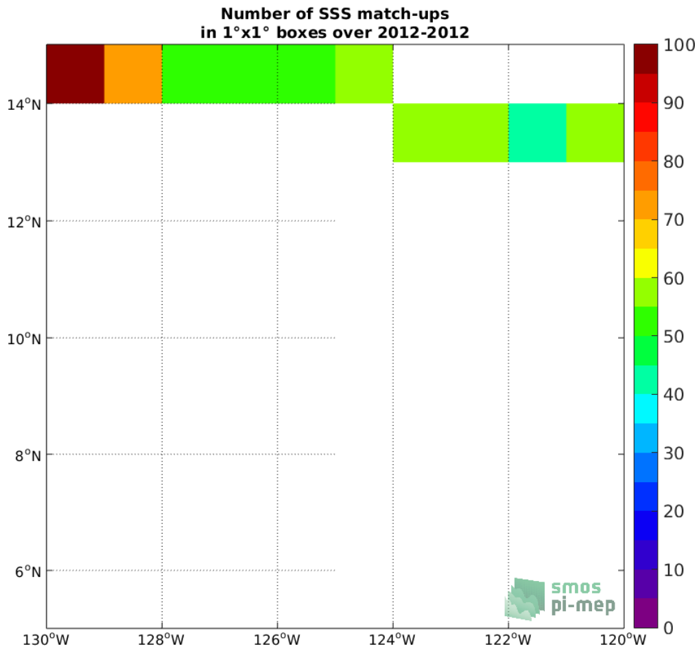
Figure 4: Number of SSS match-ups between TSG (GOSUD-Research-vessel) SSS and the CCI SSS L4 Merged-OI v3.2 - 30-day running (ESA) SSS product for the SPURS 2 Pi-MEP region over 1°x1° boxes and for the full satellite product period.
