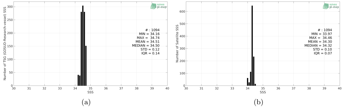
Figure 2: Histograms of SSS from TSG (GOSUD-Research-vessel) (a) and CCI SSS L4 Merged-OI v3.2 - 30-day running (ESA) (b) considering all match-up pairs per bins of 0.1 over the SPURS 2 Pi-MEP region and for the full satellite product period.
