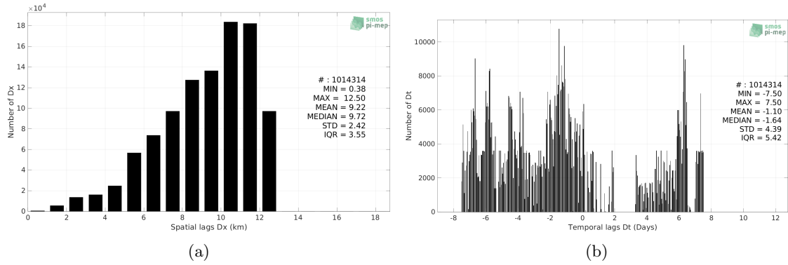
Figure 5: Histograms of the spatial (a) and temporal (b) lags between the location/time of the Salinity Snake (SPURS 2) measurement and the date of the corresponding CCI SSS L4 Merged-OI v3.2 - 30-day running (ESA) SSS pixel.
