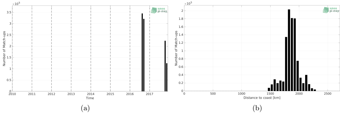
Figure 1: Number of match-ups between Salinity Snake (SPURS 2) and CCI SSS L4 Merged-OI v3.2 - 30-day running (ESA) SSS as a function of time (a) and as function of the distance to coast (b) over the SPURS 2 Pi-MEP region and for the full satellite product period.
