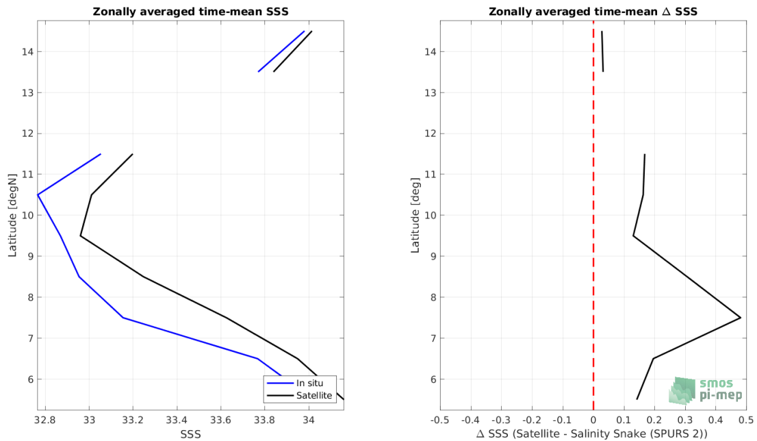
Figure 8: Left panel: Zonal mean SSS from CCI SSS L4 Merged-OI v3.2 - 30-day running (ESA) satellite product (black) and from Salinity Snake (SPURS 2) (blue). Right panel: Zonal mean of \Delta SSS (Satellite - Salinity Snake (SPURS 2)) for all the collected Pi-MEP match-up pairs estimated over the full satellite product period.
