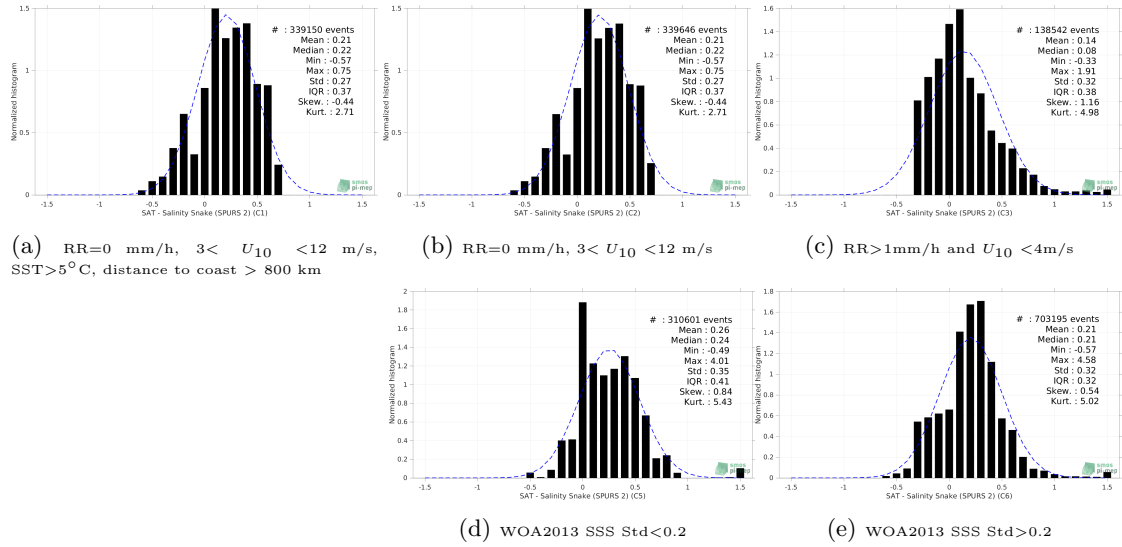
Figure 13: Normalized histogram of \Delta SSS (CCI SSS L4 Merged-OI v3.2 - 30-day running (ESA) - Salinity Snake (SPURS 2)) for 5 different subdatasets corresponding to: RR=0 mm/h, 3 < U_{10} < 12 m/s, SST > 5°C, distance to coast > 800 km (a), RR=0 mm/h, 3 < U_{10} < 12 m/s (b), RR > 1mm/h and U_{10} < 4 m/s (c), WOA2013 SSS Std < 0.2 (d), WOA2013 SSS Std > 0.2 (e).
