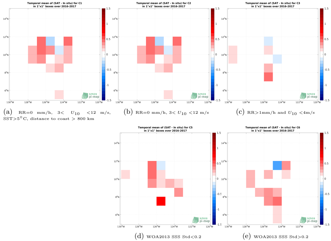
Figure 12: Temporal mean gridded over spatial boxes of size 1^\circ \times 1^\circ of \Delta SSS (CCI SSS L4 Merged-OI v3.2 - 30-day running (ESA) - Salinity Snake (SPURS 2)) for 5 different subdatasets corresponding to:RR=0 mm/h, 3 < U_{10} < 12 m/s, SST>5°C, distance to coast > 800 km (a), RR=0 mm/h, 3 < U_{10} < 12 m/s (b), RR>1mm/h and U_{10} < 4 m/s (c), WOA2013 SSS Std<0.2 (d), WOA2013 SSS Std>0.2 (e).
