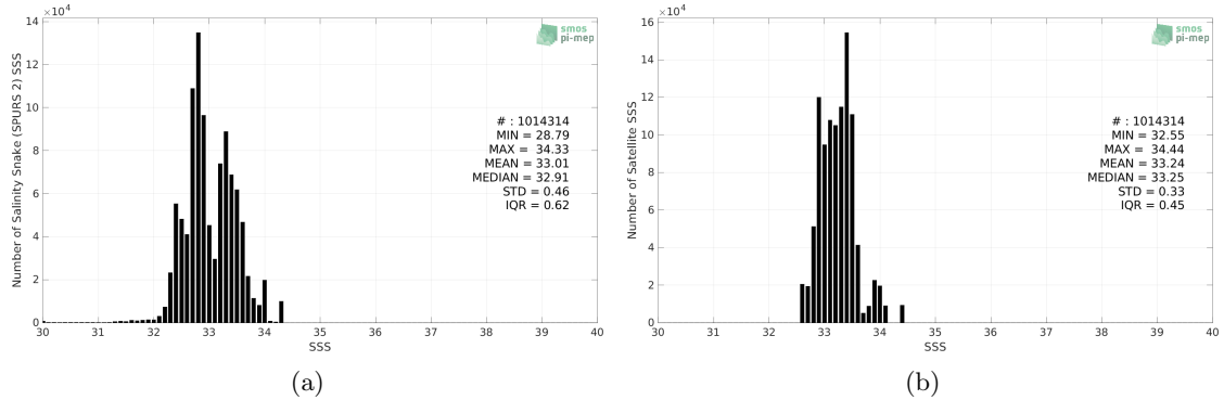
Figure 2: Histograms of SSS from Salinity Snake (SPURS 2) (a) and CCI SSS L4 Merged-OI v3.2 - 30-day running (ESA) (b) considering all match-up pairs per bins of 0.1 over the SPURS 2 Pi-MEP region and for the full satellite product period.
