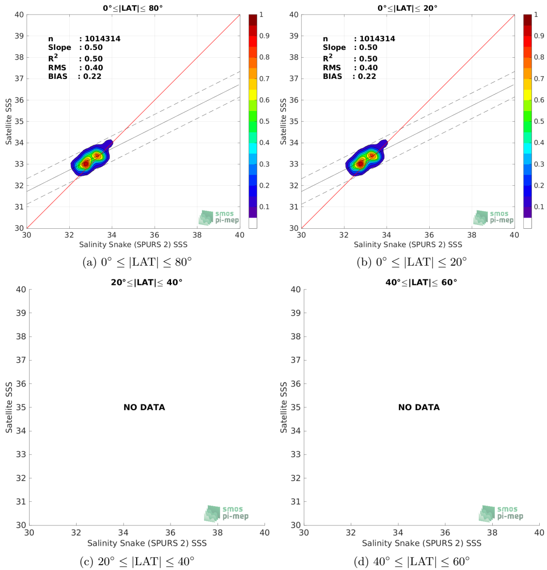
Figure 9: Contour maps of the concentration of CCI SSS L4 Merged-OI v3.2 - 30-day running (ESA) SSS (y-axis) versus Salinity Snake (SPURS 2) SSS (x-axis) at match-up pairs for different latitude bands. For each plot, the red line shows x=y . The black thin and dashed lines indicate a linear fit through the data cloud and the \pm 95\% confidence levels, respectively. The number match-up pairs n , the slope and R^2 coefficient of the linear fit, the root mean square (RMS) and the mean bias between satellite and in situ data are indicated for each latitude band in each plots.
