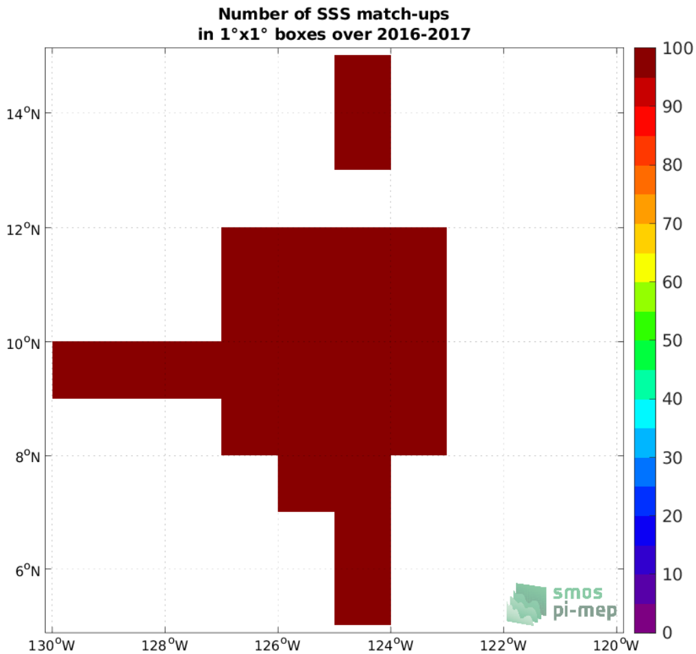
Figure 4: Number of SSS match-ups between Salinity Snake (SPURS 2) SSS and the CCI SSS L4 Merged-OI v3.2 - 30-day running (ESA) SSS product for the SPURS 2 Pi-MEP region over 1^\circ \times 1^\circ boxes and for the full satellite product period.
