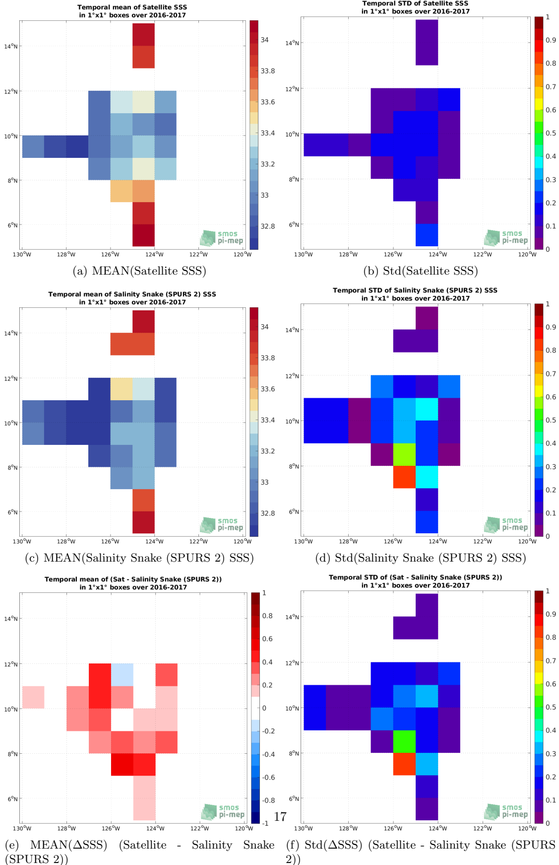
Figure 6: Temporal mean (left) and Std (right) of SSS from CCI SSS L4 Merged-OI v3.2 - 30-day running (ESA) (top), Salinity Snake (SPURS 2) (middle), and of \Delta SSS (Satellite - Salinity Snake (SPURS 2)). Only match-up pairs are used to generate these maps.
