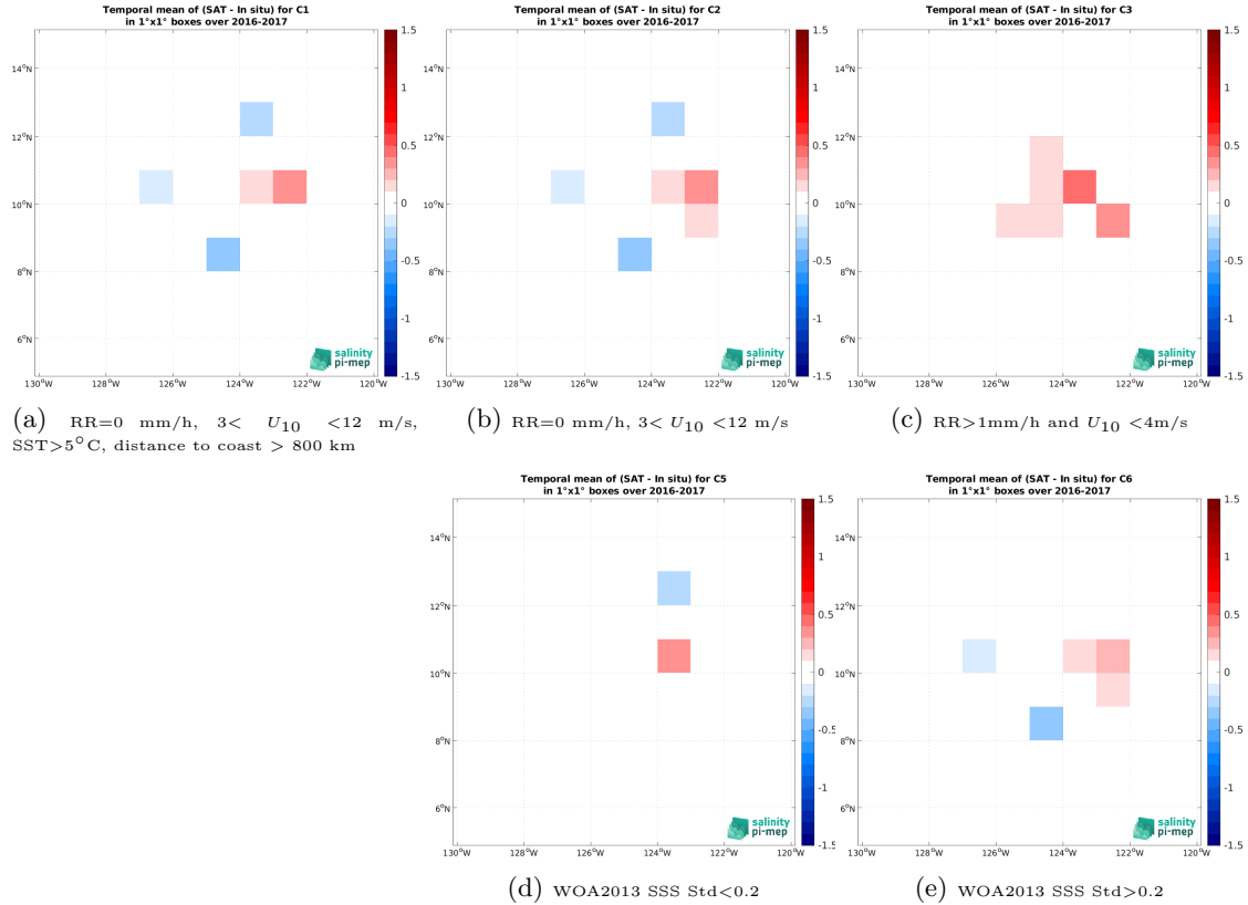
Figure 12: Temporal mean gridded over spatial boxes of size 1^{\circ}\times 1^{\circ} of \Delta\text{SSS} (CCI SSS L4 Merged-OI v3.2 - 30-day running (ESA) - Seaglider (SPURS 2)) for 5 different subdatasets corresponding to:RR=0 mm/h, 3 < U_{10} < 12 m/s, SST >5^{\circ}\text{C} , distance to coast > 800 km (a), RR=0 mm/h, 3 < U_{10} < 12 m/s (b), RR >1 mm/h and U_{10} < 4 m/s (c), WOA2013 SSS Std <0.2 (d), WOA2013 SSS Std >0.2 (e).
