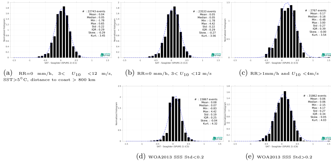
Figure 13: Normalized histogram of \Delta SSS (CCI SSS L4 Merged-OI v3.2 - 30-day running (ESA) - Seaglider (SPURS 2)) for 5 different subdatasets corresponding to: RR=0 mm/h, 3 < U_{10} < 12 m/s, SST>5°C, distance to coast > 800 km (a), RR=0 mm/h, 3 < U_{10} < 12 m/s (b), RR>1mm/h and U_{10} < 4 m/s (c), WOA2013 SSS Std<0.2 (d), WOA2013 SSS Std>0.2 (e).
