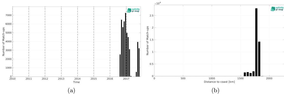
Figure 1: Number of match-ups between Seaglider (SPURS 2) and CCI SSS L4 Merged-OI v3.2 - 30-day running (ESA) SSS as a function of time (a) and as function of the distance to coast (b) over the SPURS 2 Pi-MEP region and for the full satellite product period.
