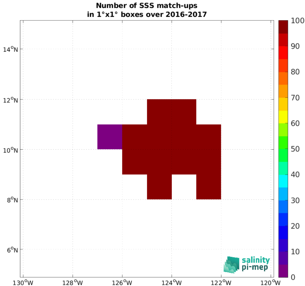
Figure 4: Number of SSS match-ups between Seaglider (SPURS 2) SSS and the CCI SSS L4 Merged-OI v3.2 - 30-day running (ESA) SSS product for the SPURS 2 Pi-MEP region over 1^\circ \times 1^\circ boxes and for the full satellite product period.
