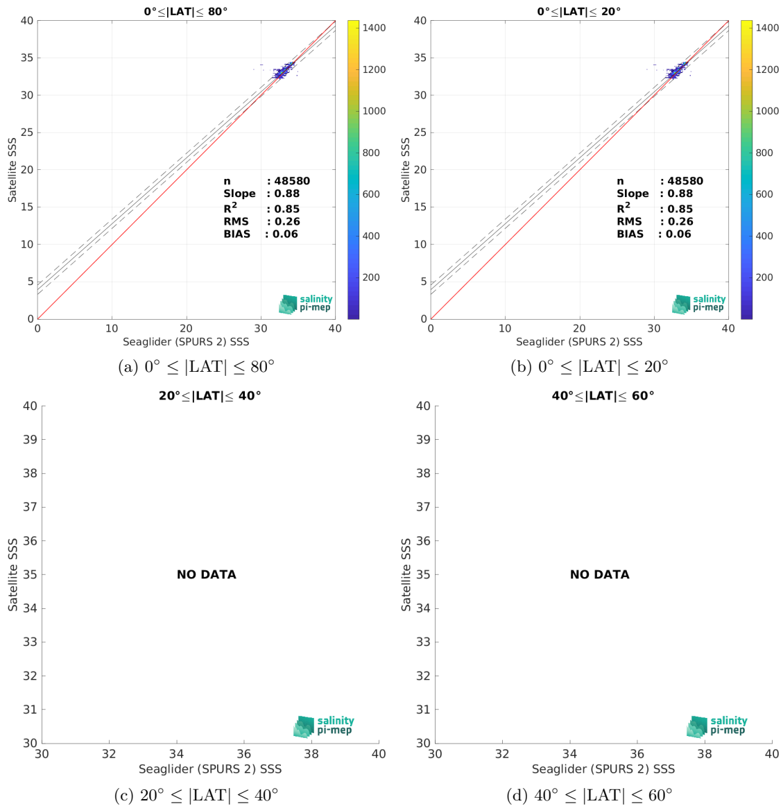
Figure 9: Contour maps of the concentration of CCI SSS L4 Merged-OI v3.2 - 30-day running (ESA) SSS (y-axis) versus Seaglider (SPURS 2) SSS (x-axis) at match-up pairs for different latitude bands. For each plot, the red line shows x=y . The black thin and dashed lines indicate a linear fit through the data cloud and the \pm 95\% confidence levels, respectively. The number match-up pairs n , the slope and R^2 coefficient of the linear fit, the root mean square (RMS) and the mean bias between satellite and in situ data are indicated for each latitude band in each plots.
