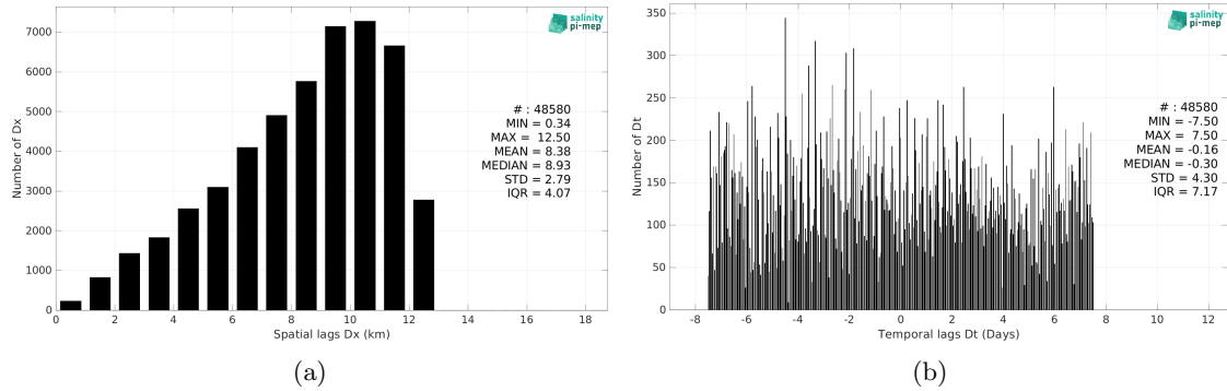
Figure 5: Histograms of the spatial (a) and temporal (b) lags between the location/time of the Seaglider (SPURS 2) measurement and the date of the corresponding CCI SSS L4 Merged-OI v3.2 - 30-day running (ESA) SSS pixel.
