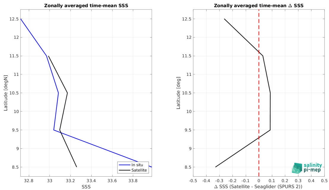
Figure 8: Left panel: Zonal mean SSS from CCI SSS L4 Merged-OI v3.2 - 30-day running (ESA) satellite product (black) and from Seaglider (SPURS 2) (blue). Right panel: Zonal mean of \Delta SSS (Satellite - Seaglider (SPURS 2)) for all the collected Pi-MEP match-up pairs estimated over the full satellite product period.
