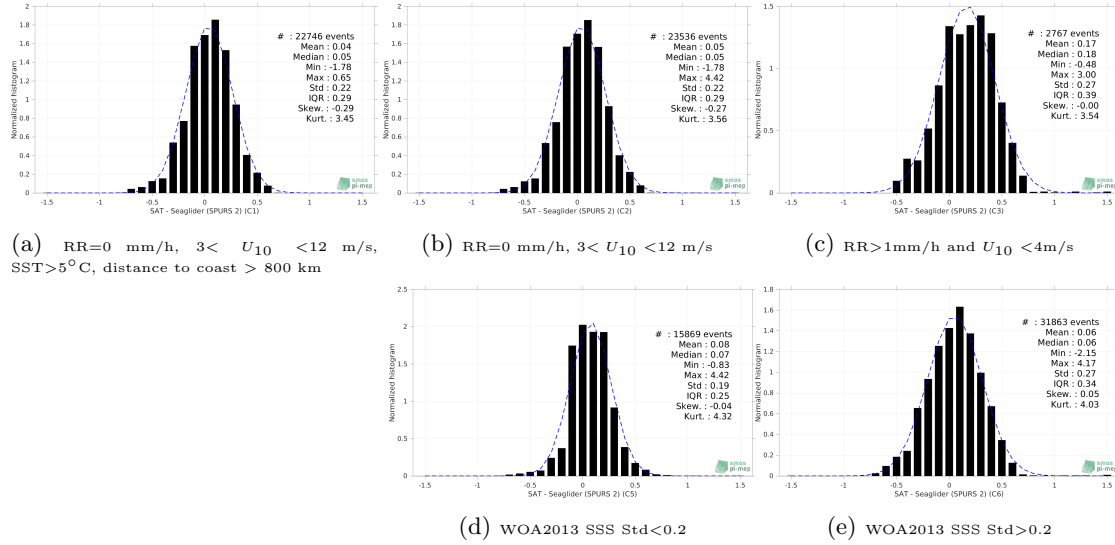
Figure 13: Normalized histogram of \Delta\text{SSS} (CCI SSS L4 Merged-OI v3.2 - 30-day running (ESA) - Seaglider (SPURS 2)) for 5 different subdatasets corresponding to: RR=0 mm/h, 3 < U_{10} < 12 m/s, SST >5^{\circ}\text{C} , distance to coast > 800 km (a), RR=0 mm/h, 3 < U_{10} < 12 m/s (b), RR >1 mm/h and U_{10} < 4 m/s (c), WOA2013 SSS Std <0.2 (d), WOA2013 SSS Std >0.2 (e).
