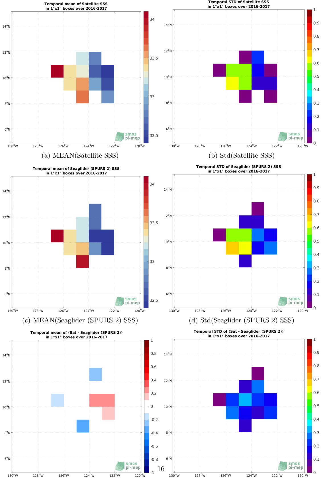
Figure 6: Temporal mean (left) and Std (right) of SSS from CCI SSS L4 Merged-OI v3.2 - 30-day running (ESA) (top), Seaglider (SPURS 2) (middle), and of \Delta SSS (Satellite - Seaglider (SPURS 2)). Only match-up pairs are used to generate these maps.
