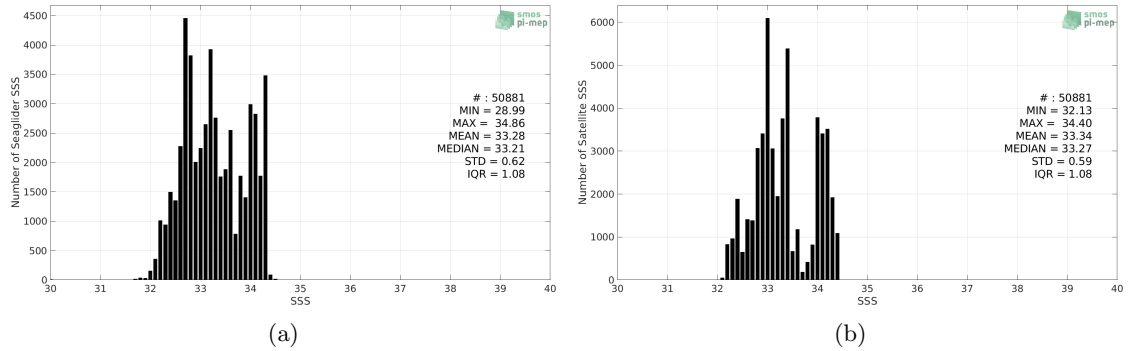
Figure 2: Histograms of SSS from Seaglider (a) and CCI SSS L4 Merged-OI v3.2 - 30-day running (ESA) (b) considering all match-up pairs per bins of 0.1 over the SPURS 2 Pi-MEP region and for the full satellite product period.
