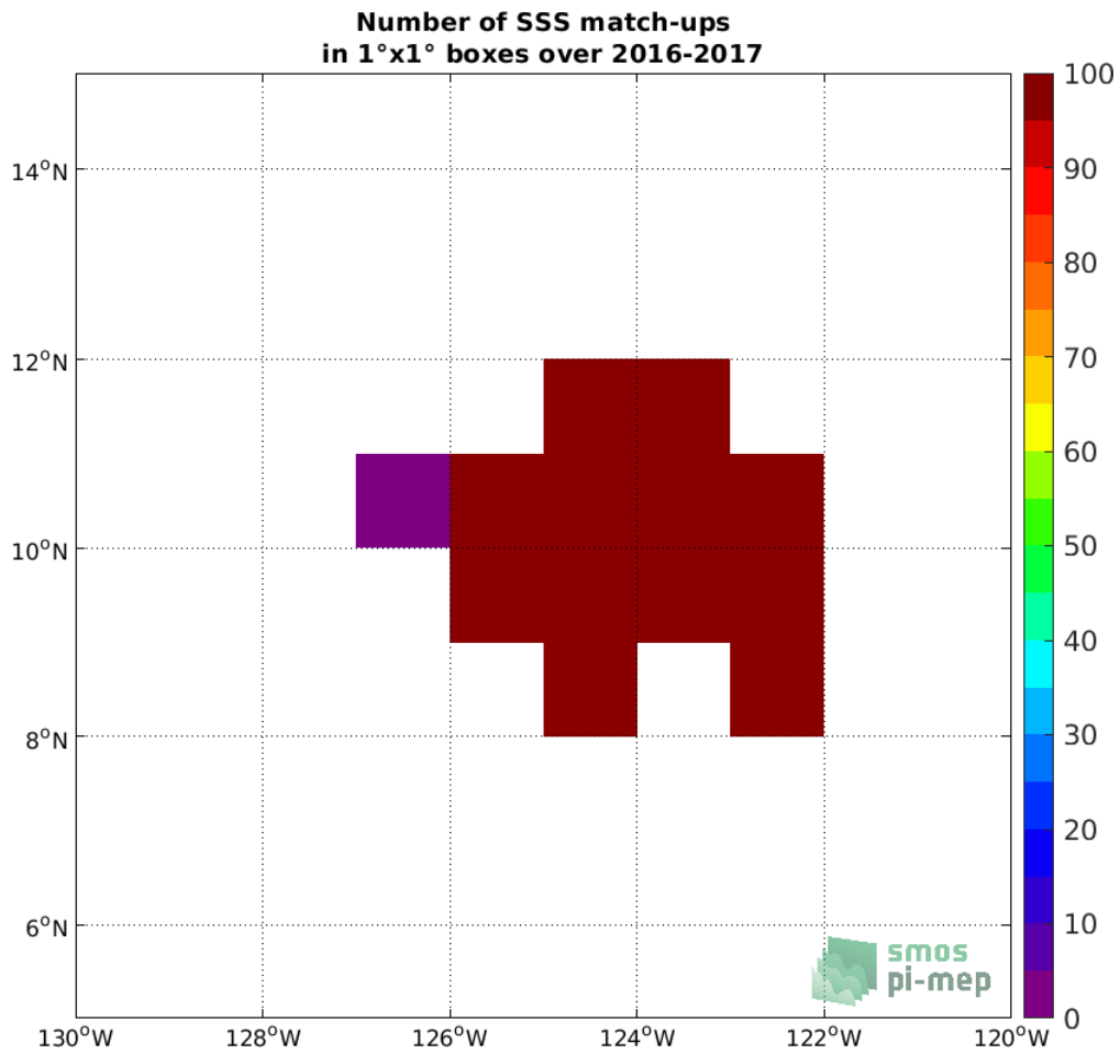
Figure 3: Number of SSS match-ups between Seaglider SSS and the CCI SSS L4 Merged-OI v3.2 - 30-day running (ESA) SSS product for the SPURS 2 Pi-MEP region over 1°×1° boxes and for the full satellite product period.
