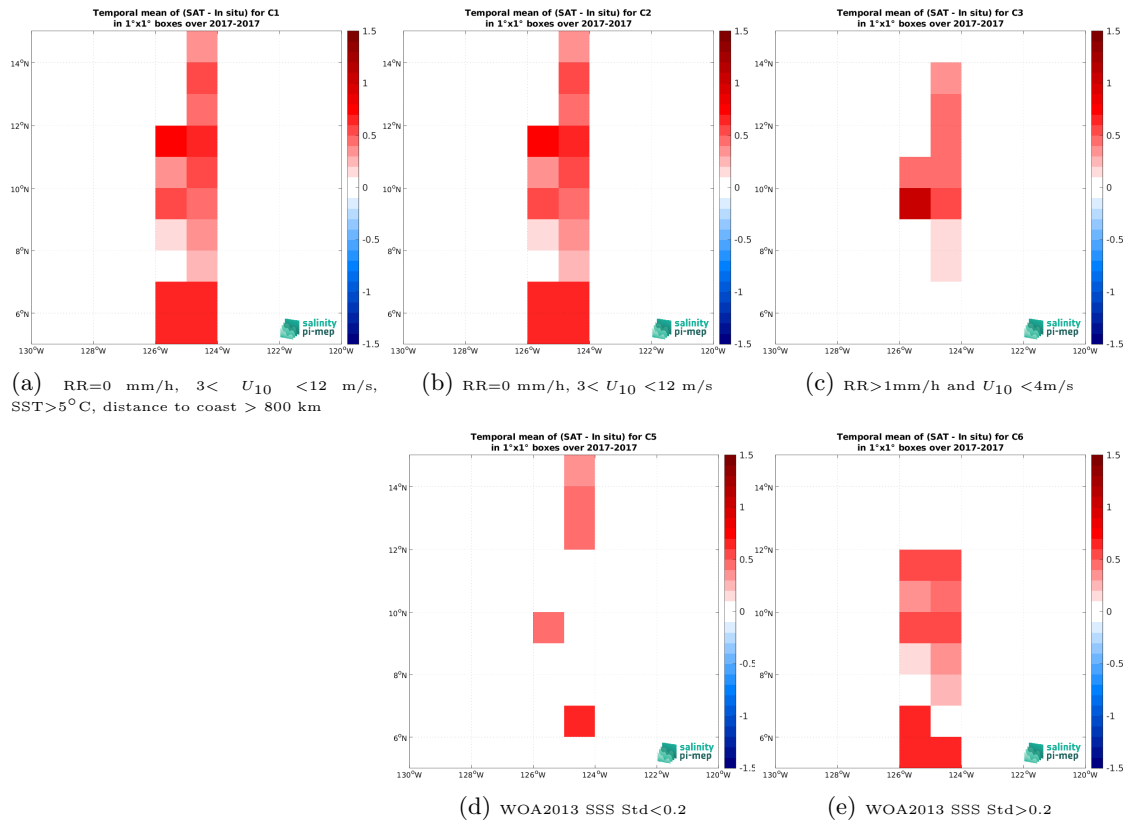
Figure 12: Temporal mean gridded over spatial boxes of size 1^\circ \times 1^\circ of \Delta SSS (CCI SSS L4 Merged-OI v3.2 - 30-day running (ESA) - Saildrone) for 5 different subdatasets corresponding to:RR=0 mm/h, 3 < U_{10} < 12 m/s, SST >5^\circ\text{C} , distance to coast > 800 km (a), RR=0 mm/h, 3 < U_{10} < 12 m/s (b), RR >1 mm/h and U_{10} < 4 m/s (c), WOA2013 SSS Std <0.2 (d), WOA2013 SSS Std >0.2 (e).
