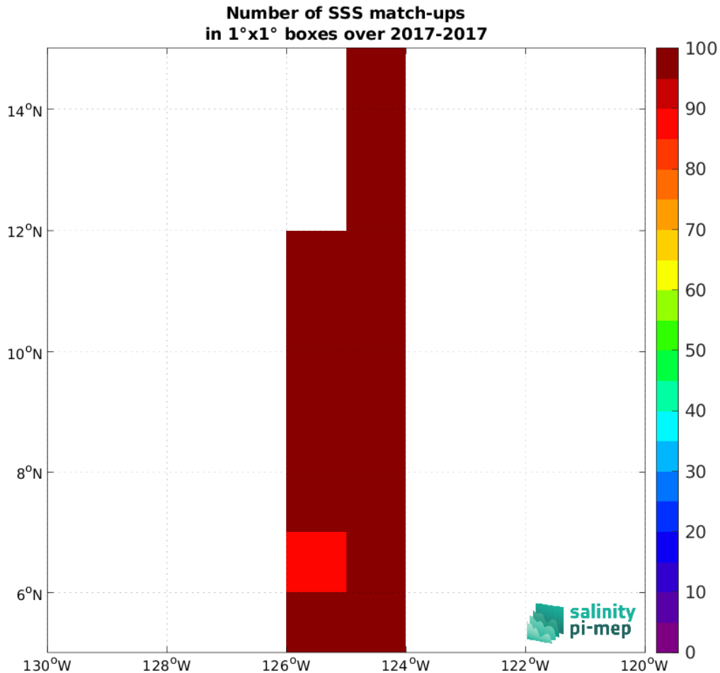
Figure 4: Number of SSS match-ups between Saildrone SSS and the CCI SSS L4 Merged-OI v3.2 - 30-day running (ESA) SSS product for the SPURS 2 Pi-MEP region over 1^\circ \times 1^\circ boxes and for the full satellite product period.
