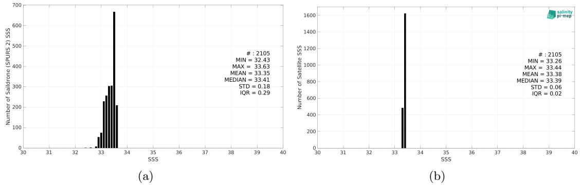
Figure 2: Histograms of SSS from Sairdronne (SPURS 2) (a) and CCI SSS L4 Merged-OI v3.2 - 30-day running (ESA) (b) considering all match-up pairs per bins of 0.1 over the SPURS 2 Pi-MEP region and for the full satellite product period.
