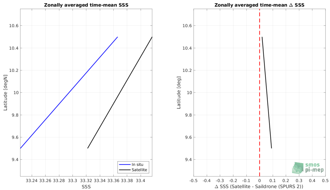
Figure 8: Left panel: Zonal mean SSS from CCI SSS L4 Merged-OI v3.2 - 30-day running (ESA) satellite product (black) and from Sairdron (SPURS 2) (blue). Right panel: Zonal mean of \Delta SSS (Satellite - Sairdron (SPURS 2)) for all the collected Pi-MEP match-up pairs estimated over the full satellite product period.
