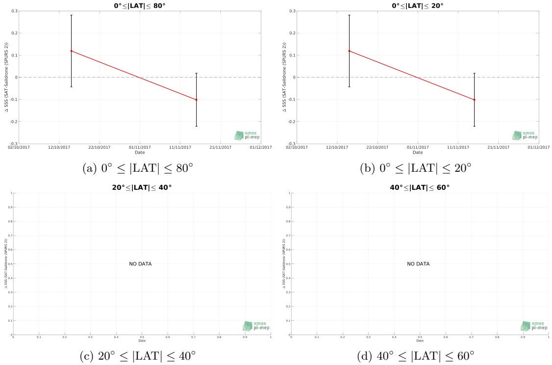
Figure 10: Monthly median (red curves) of \Delta SSS (Satellite - Sairdrome (SPURS 2)) and \pm 1 Std (black vertical thick bars) as function of time for all the collected Pi-MEP match-up pairs estimated over the SPURS 2 Pi-MEP region and for the full satellite product period are shown for different latitude bands: (a) 80°S-80°N, (b) 20°S-20°N, (c) 40°S-20°S and 20°N-40°N and (d) 60°S-40°S and 40°N-60°N.
