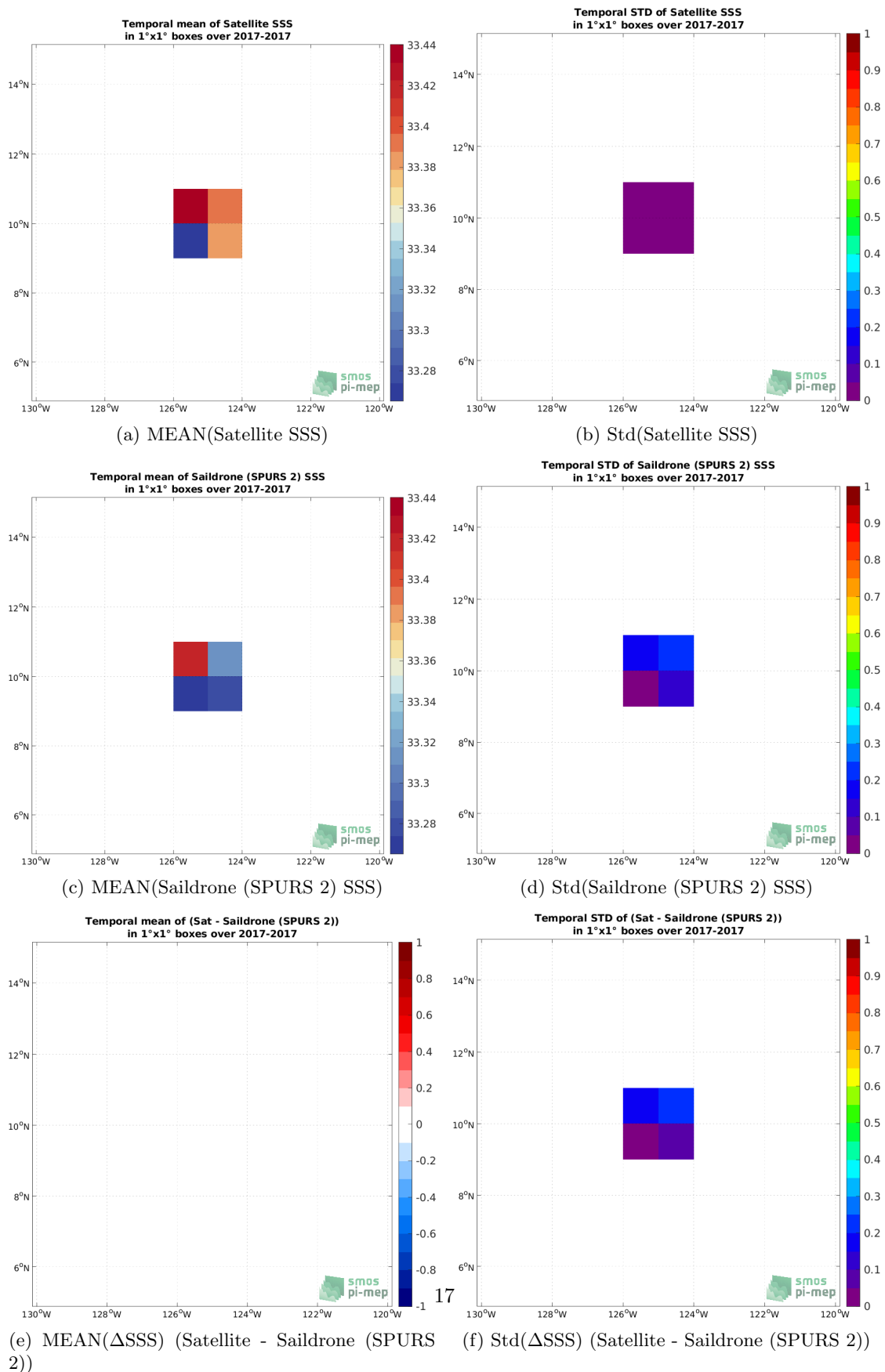
Figure 6: Temporal mean (left) and Std (right) of SSS from CCI SSS L4 Merged-OI v3.2 - 30-day running (ESA) (top), Saildrone (SPURS 2) (middle), and of \Delta SSS (Satellite - Saildrone (SPURS 2)). Only match-up pairs are used to generate these maps.
