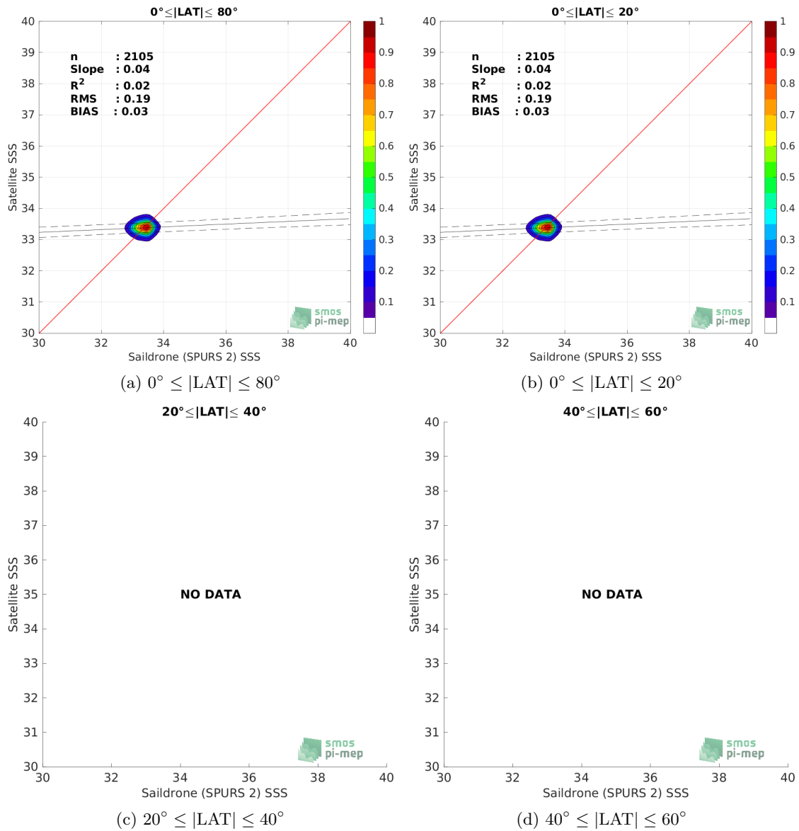
Figure 9: Contour maps of the concentration of CCI SSS L4 Merged-OI v3.2 - 30-day running (ESA) SSS (y-axis) versus Saildrone (SPURS 2) SSS (x-axis) at match-up pairs for different latitude bands. For each plot, the red line shows x=y . The black thin and dashed lines indicate a linear fit through the data cloud and the \pm 95\% confidence levels, respectively. The number match-up pairs n , the slope and R^2 coefficient of the linear fit, the root mean square (RMS) and the mean bias between satellite and in situ data are indicated for each latitude band in each plots.
