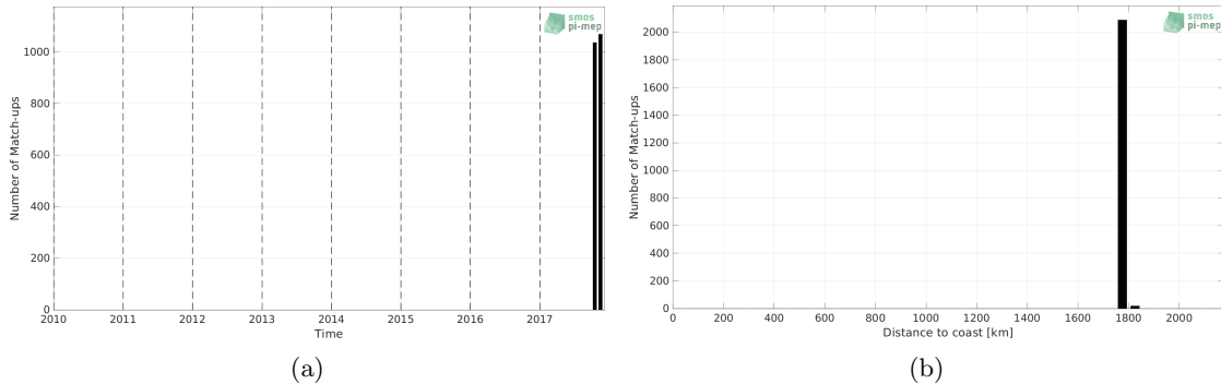
Figure 1: Number of match-ups between Saildrone (SPURS 2) and CCI SSS L4 Merged-OI v3.2 - 30-day running (ESA) SSS as a function of time (a) and as function of the distance to coast (b) over the SPURS 2 Pi-MEP region and for the full satellite product period.
