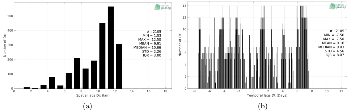
Figure 5: Histograms of the spatial (a) and temporal (b) lags between the location/time of the Saildrone (SPURS 2) measurement and the date of the corresponding CCI SSS L4 Merged-OI v3.2 - 30-day running (ESA) SSS pixel.
