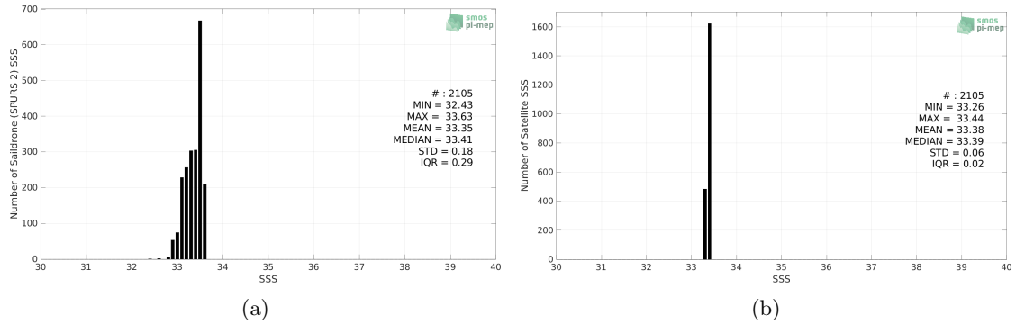
Figure 2: Histograms of SSS from Sairdrone (SPURS 2) (a) and CCI SSS L4 Merged-OI v3.2 - 30-day running (ESA) (b) considering all match-up pairs per bins of 0.1 over the SPURS 2 Pi-MEP region and for the full satellite product period.
