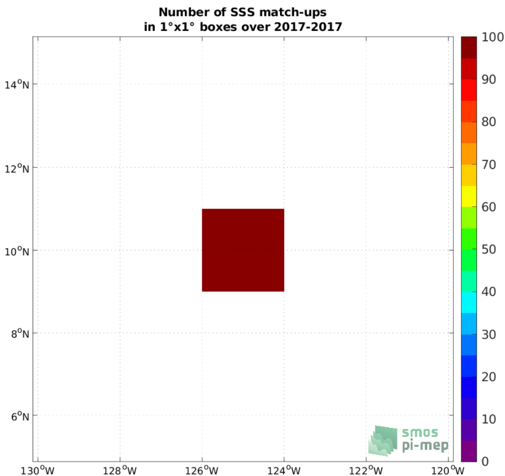
Figure 4: Number of SSS match-ups between Saildrone (SPURS 2) SSS and the CCI SSS L4 Merged-OI v3.2 - 30-day running (ESA) SSS product for the SPURS 2 Pi-MEP region over 1^\circ \times 1^\circ boxes and for the full satellite product period.
