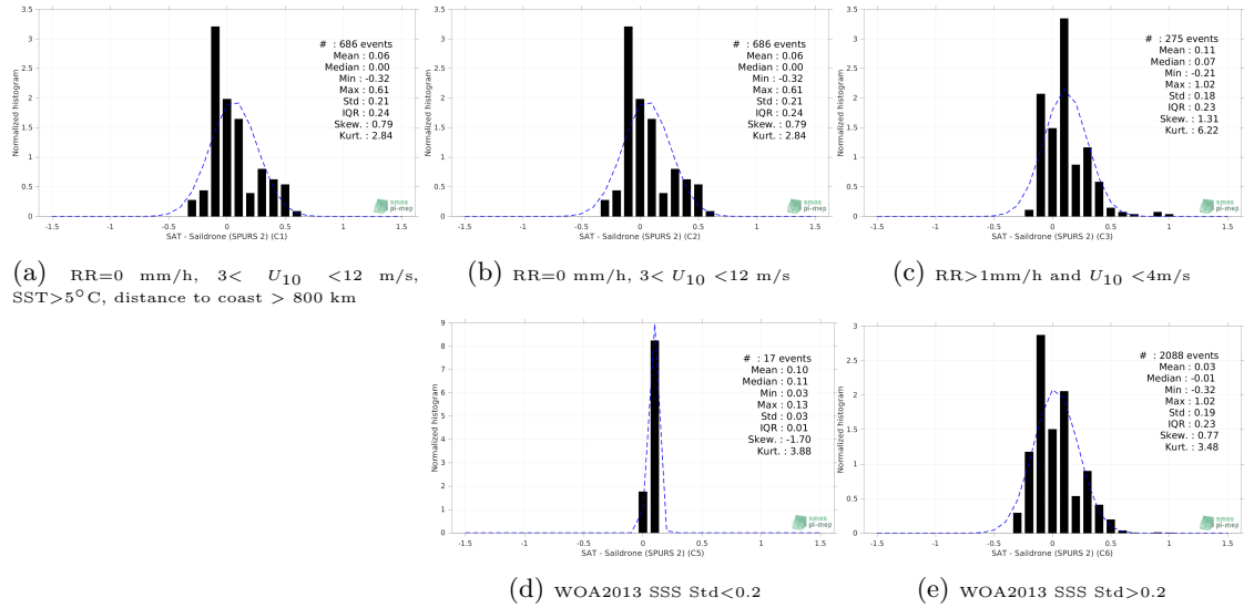
Figure 13: Normalized histogram of \Delta SSS (CCI SSS L4 Merged-OI v3.2 - 30-day running (ESA) - Saldrone (SPURS 2)) for 5 different subdatasets corresponding to: RR=0 mm/h, 3 < U_{10} < 12 m/s, SST > 5°C, distance to coast > 800 km (a), RR=0 mm/h, 3 < U_{10} < 12 m/s (b), RR > 1mm/h and U_{10} < 4 m/s (c), WOA2013 SSS Std < 0.2 (d), WOA2013 SSS Std > 0.2 (e).
