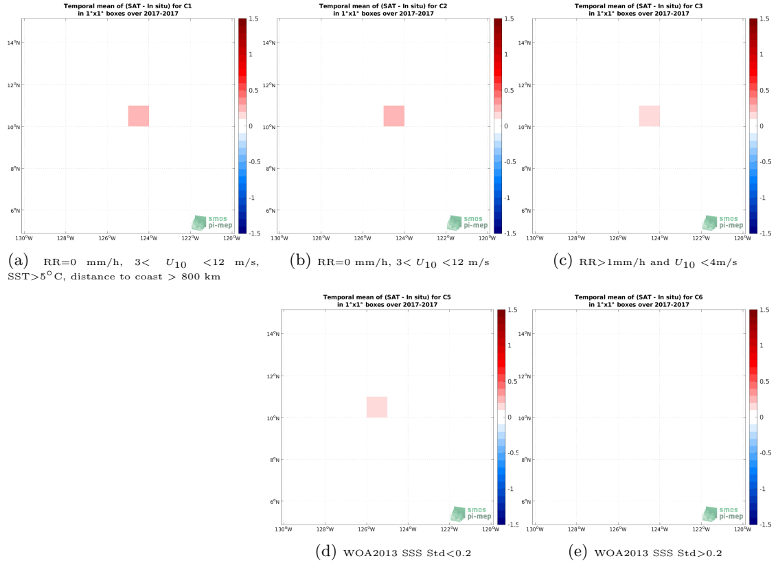
Figure 12: Temporal mean gridded over spatial boxes of size 1^{\circ}\times 1^{\circ} of \Delta\text{SSS} (CCI SSS L4 Merged-OI v3.2 - 30-day running (ESA) - Saildrone (SPURS 2)) for 5 different subdatasets corresponding to:RR=0 mm/h, 3 < U_{10} < 12 m/s, SST >5^{\circ}\text{C} , distance to coast > 800 km (a), RR=0 mm/h, 3 < U_{10} < 12 m/s (b), RR >1 mm/h and U_{10} < 4 m/s (c), WOA2013 SSS Std <0.2 (d), WOA2013 SSS Std >0.2 (e).
