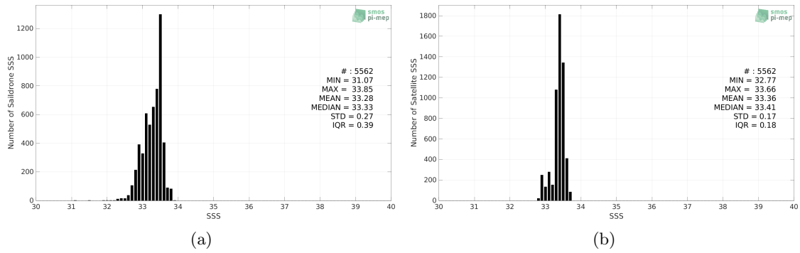
Figure 2: Histograms of SSS from Sairdrone (a) and CCI SSS L4 Merged-OI v3.2 - 30-day running (ESA) (b) considering all match-up pairs per bins of 0.1 over the SPURS 2 Pi-MEP region and for the full satellite product period.
