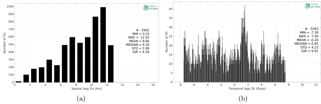
Figure 4: Histograms of the spatial (a) and temporal (b) lags between the location/time of the Saildrone measurement and the date of the corresponding CCI SSS L4 Merged-OI v3.2 - 30-day running (ESA) SSS pixel.
