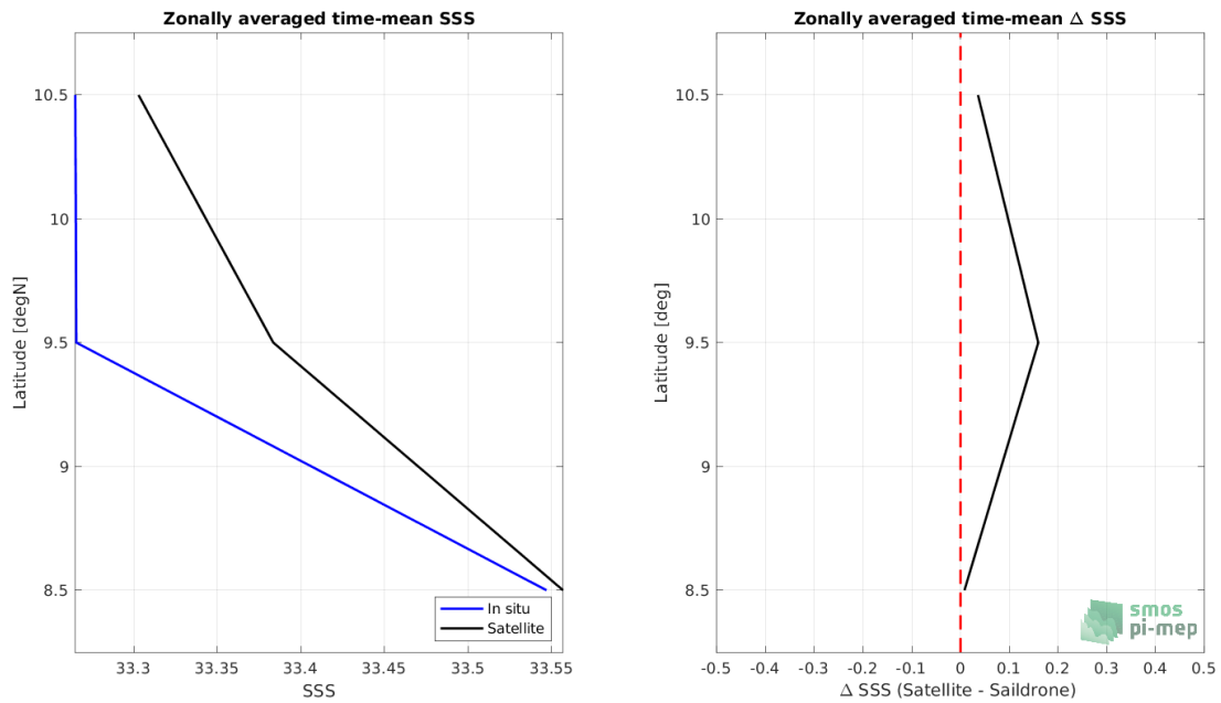
Figure 7: Left panel: Zonal mean SSS from CCI SSS L4 Merged-OI v3.2 - 30-day running (ESA) satellite product (black) and from Sairdron (blue). Right panel: Zonal mean of \Delta SSS (Satellite - Sairdron) for all the collected Pi-MEP match-up pairs estimated over the full satellite product period.
