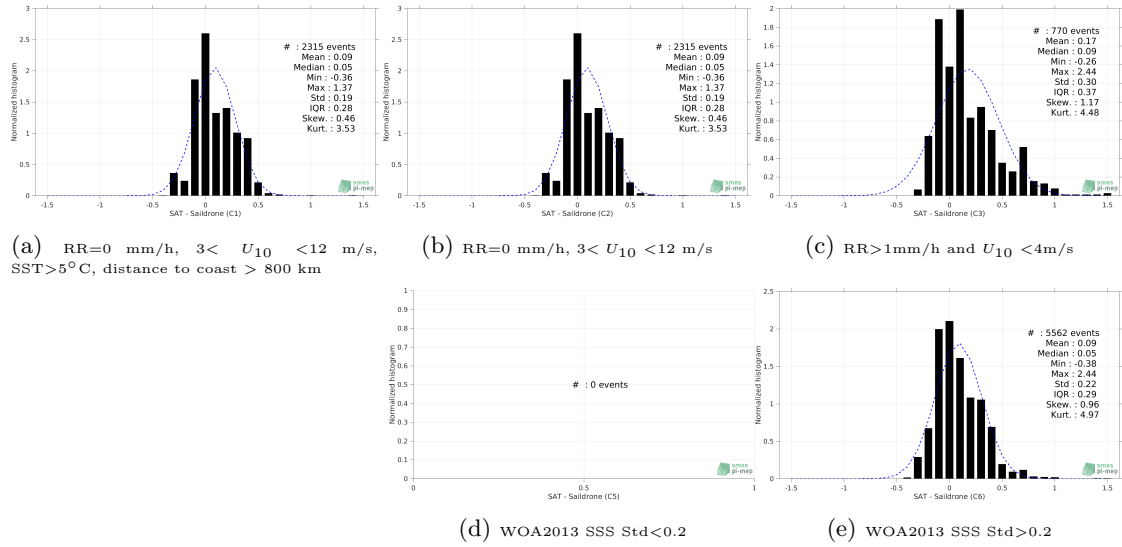
Figure 12: Normalized histogram of \Delta SSS (CCI SSS L4 Merged-OI v3.2 - 30-day running (ESA) - Saildrone) for 5 different subdatasets corresponding to: RR=0 mm/h, 3 < U_{10} < 12 m/s, SST > 5°C, distance to coast > 800 km (a), RR=0 mm/h, 3 < U_{10} < 12 m/s (b), RR > 1mm/h and U_{10} < 4 m/s (c), WOA2013 SSS Std < 0.2 (d), WOA2013 SSS Std > 0.2 (e).
