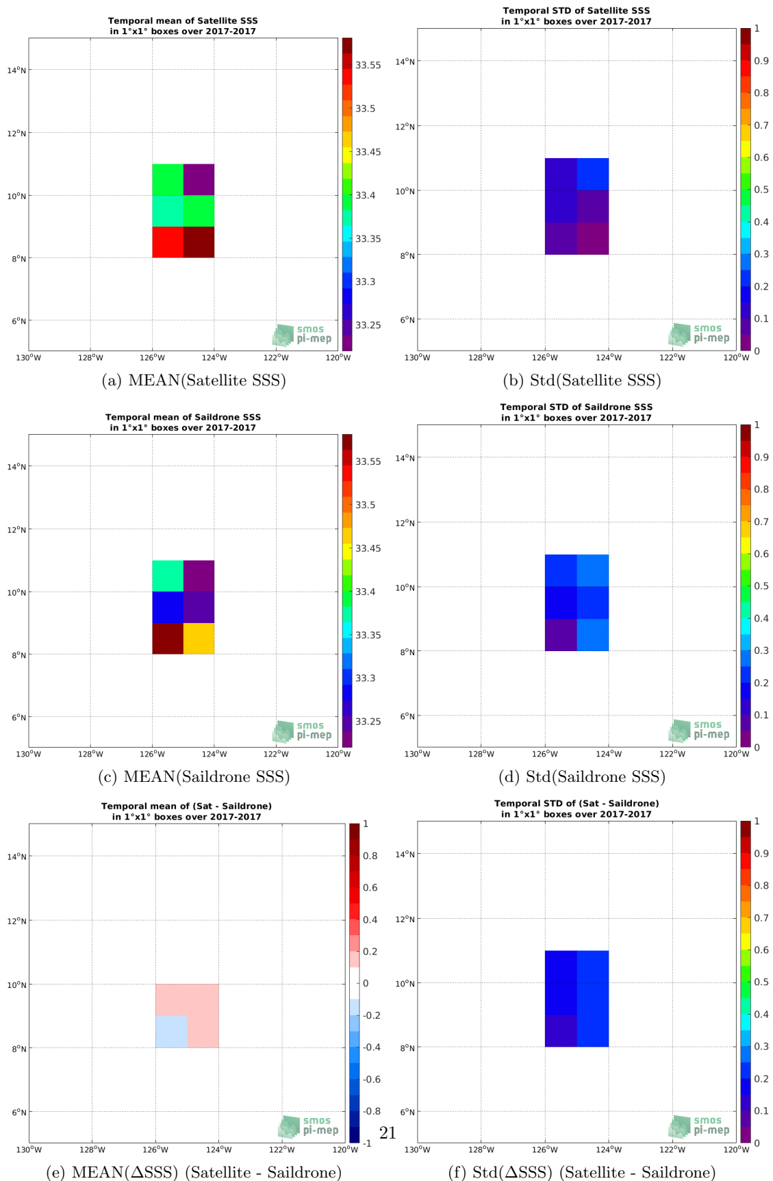
Figure 5: Temporal mean (left) and Std (right) of SSS from CCI SSS L4 Merged-OI v3.2 - 30-day running (ESA) (top), Saildrone (middle), and of \Delta SSS (Satellite - Saildrone). Only match-up pairs are used to generate these maps.
