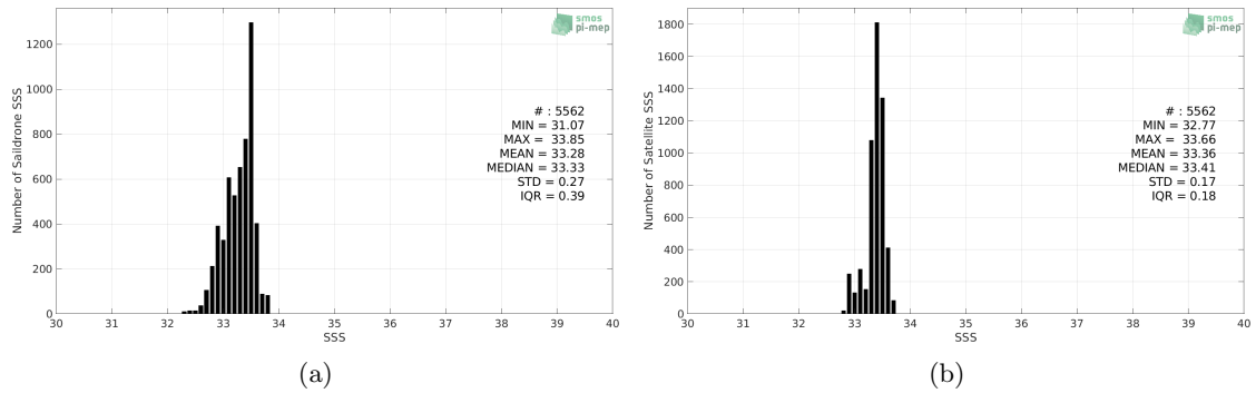
Figure 2: Histograms of SSS from Saildrone (a) and CCI SSS L4 Merged-OI v3.2 - 30-day running (ESA) (b) considering all match-up pairs per bins of 0.1 over the SPURS 2 Pi-MEP region and for the full satellite product period.
