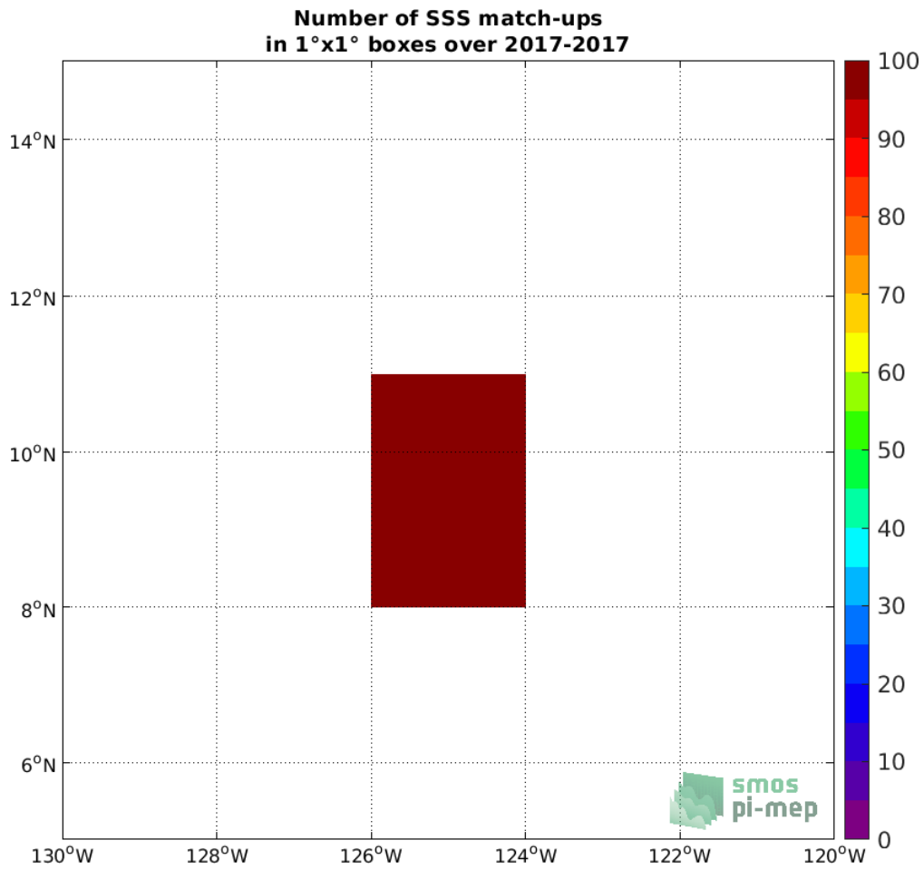
Figure 3: Number of SSS match-ups between Sairdrone SSS and the CCI SSS L4 Merged-OI v3.2 - 30-day running (ESA) SSS product for the SPURS 2 Pi-MEP region over 1°×1° boxes and for the full satellite product period.
