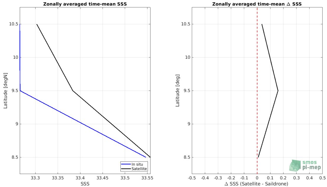
Figure 7: Left panel: Zonal mean SSS from CCI SSS L4 Merged-OI v3.2 - 30-day running (ESA) satellite product (black) and from Sairdrone (blue). Right panel: Zonal mean of \Delta SSS (Satellite - Sairdrone) for all the collected Pi-MEP match-up pairs estimated over the full satellite product period.
