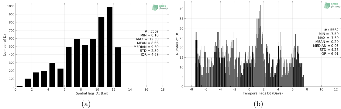
Figure 4: Histograms of the spatial (a) and temporal (b) lags between the location/time of the Sairdrone measurement and the date of the corresponding CCI SSS L4 Merged-OI v3.2 - 30-day running (ESA) SSS pixel.
