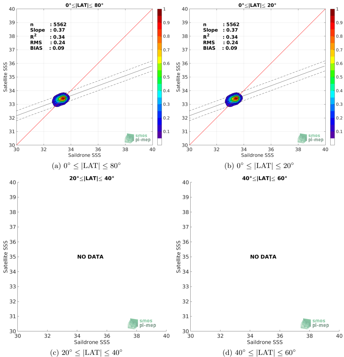
Figure 8: Contour maps of the concentration of CCI SSS L4 Merged-OI v3.2 - 30-day running (ESA) SSS (y-axis) versus Saildrone SSS (x-axis) at match-up pairs for different latitude bands. For each plot, the red line shows x=y . The black thin and dashed lines indicate a linear fit through the data cloud and the \pm 95\% confidence levels, respectively. The number match-up pairs n , the slope and R^2 coefficient of the linear fit, the root mean square (RMS) and the mean bias between satellite and in situ data are indicated for each latitude band in each plots.
