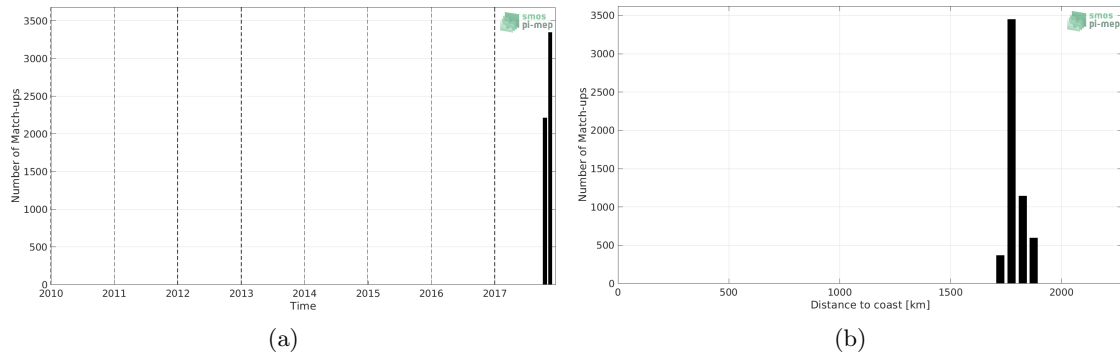
Figure 1: Number of match-ups between Saildrone and CCI SSS L4 Merged-OI v3.2 - 30-day running (ESA) SSS as a function of time (a) and as function of the distance to coast (b) over the SPURS 2 Pi-MEP region and for the full satellite product period.
