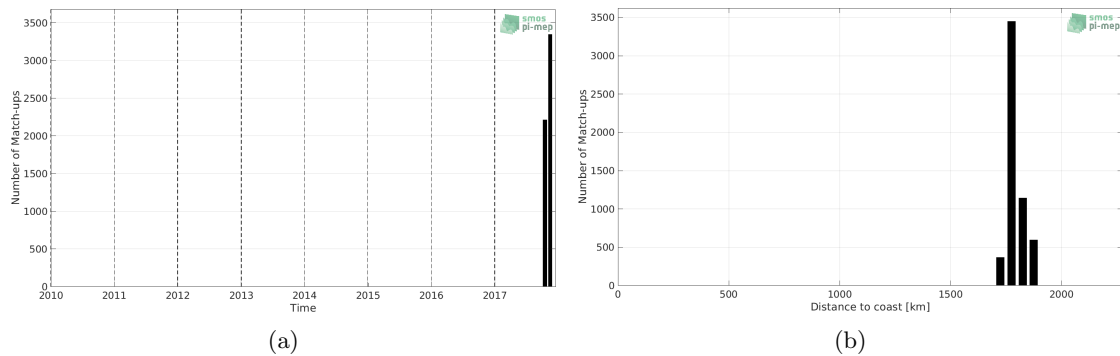
Figure 1: Number of match-ups between Sailldrone and CCI SSS L4 Merged-OI v3.2 - 30-day running (ESA) SSS as a function of time (a) and as function of the distance to coast (b) over the SPURS 2 Pi-MEP region and for the full satellite product period.
