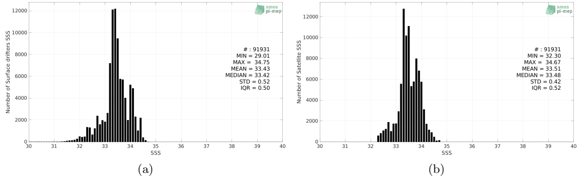
Figure 2: Histograms of SSS from Surface drifters (a) and CCI SSS L4 Merged-OI v3.2 - 30-day running (ESA) (b) considering all match-up pairs per bins of 0.1 over the SPURS 2 Pi-MEP region and for the full satellite product period.
