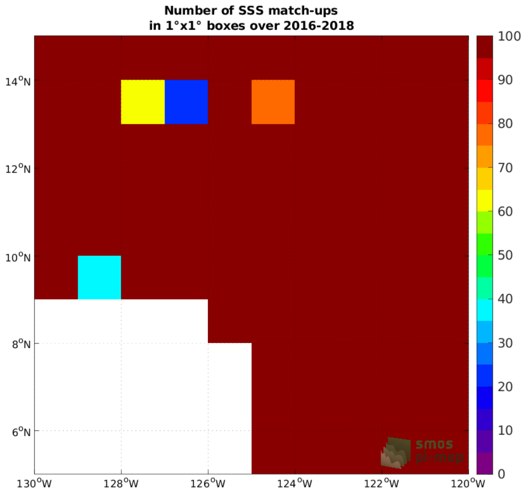
Figure 3: Number of SSS match-ups between Surface drifters SSS and the CCI SSS L4 Merged-OI v3.2 - 30-day running (ESA) SSS product for the SPURS 2 Pi-MEP region over 1°x1° boxes and for the full satellite product period.
