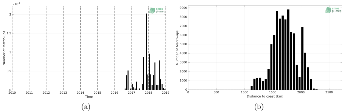
Figure 1: Number of match-ups between Surface drifters and CCI SSS L4 Merged-OI v3.2 - 30-day running (ESA) SSS as a function of time (a) and as function of the distance to coast (b) over the SPURS 2 Pi-MEP region and for the full satellite product period.
