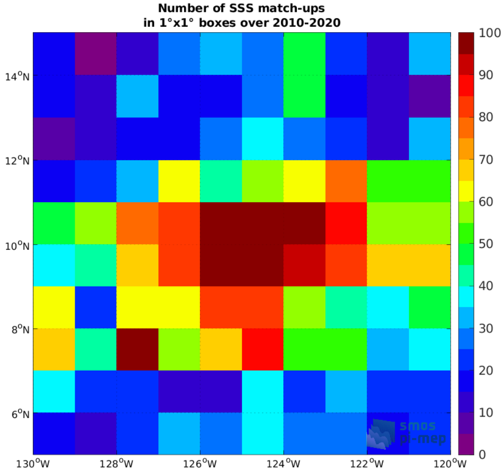
Figure 4: Number of SSS match-ups between Argo SSS and the CCI SSS L4 Merged-OI v3.2 - 30-day running (ESA) SSS product for the SPURS 2 Pi-MEP region over 1^\circ \times 1^\circ boxes and for the full satellite product period.
