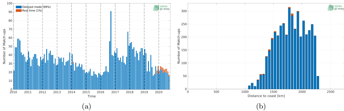
Figure 1: Number of match-ups between Argo and CCI SSS L4 Merged-OI v3.2 - 30-day running (ESA) SSS as a function of time (a) and as function of the distance to coast (b) over the SPURS 2 Pi-MEP region and for the full satellite product period.
