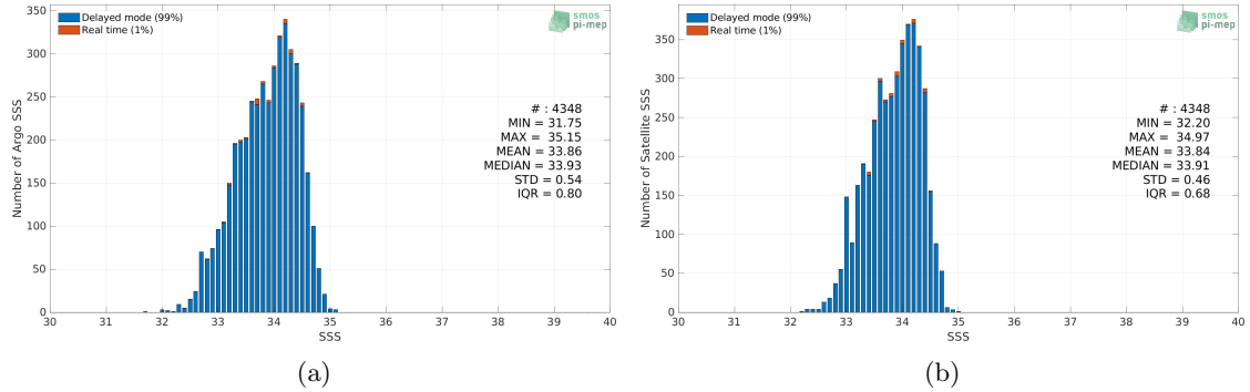
Figure 2: Histograms of SSS from Argo (a) and CCI SSS L4 Merged-OI v3.2 - 30-day running (ESA) (b) considering all match-up pairs per bins of 0.1 over the SPURS 2 Pi-MEP region and for the full satellite product period.
