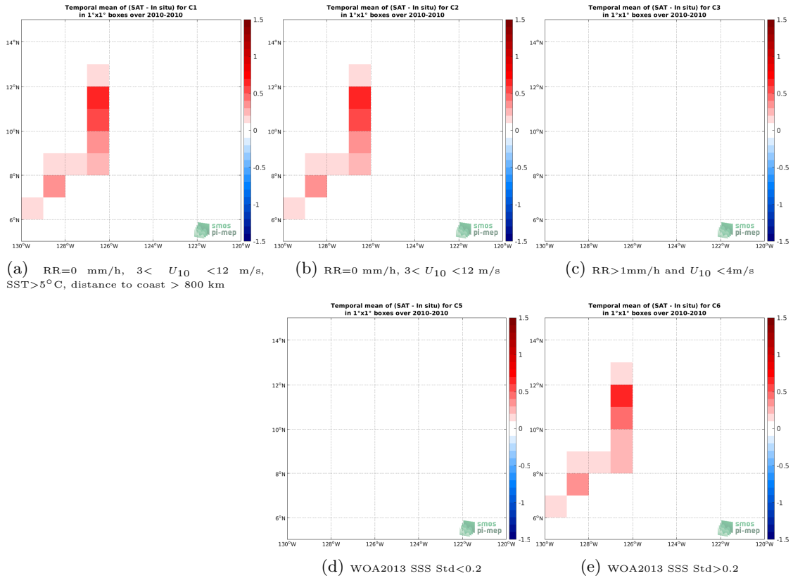
Figure 12: Temporal mean gridded over spatial boxes of size 1°x1° of \Delta SSS (CCI SSS L4 Merged-OI v2.31 - 7-day running (ESA) - TSG (GOSUD-Sailing-ship)) for 5 different subdatasets corresponding to:RR=0 mm/h, 3 < U_{10} < 12 m/s, SST>5°C, distance to coast > 800 km (a), RR=0 mm/h, 3 < U_{10} < 12 m/s (b), RR>1mm/h and U_{10} < 4 m/s (c), WOA2013 SSS Std<0.2 (d), WOA2013 SSS Std>0.2 (e).
