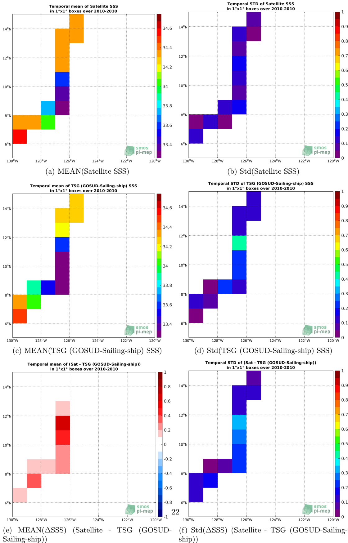
Figure 6: Temporal mean (left) and Std (right) of SSS from CCI SSS L4 Merged-OI v2.31 - 7-day running (ESA) (top), TSG (GOSUD-Sailing-ship) (middle), and of \Delta SSS (Satellite - TSG (GOSUD-Sailing-ship)). Only match-up pairs are used to generate these maps.
