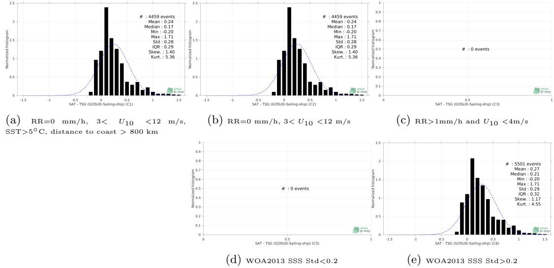
Figure 13: Normalized histogram of \Delta SSS (CCI SSS L4 Merged-OI v2.31 - 7-day running (ESA) - TSG (GOSUD-Sailing-ship)) for 5 different subdatasets corresponding to: RR=0 mm/h, 3 < U_{10} < 12 m/s, SST > 5°C, distance to coast > 800 km (a), RR=0 mm/h, 3 < U_{10} < 12 m/s (b), RR > 1mm/h and U_{10} < 4 m/s (c), WOA2013 SSS Std < 0.2 (d), WOA2013 SSS Std > 0.2 (e).
