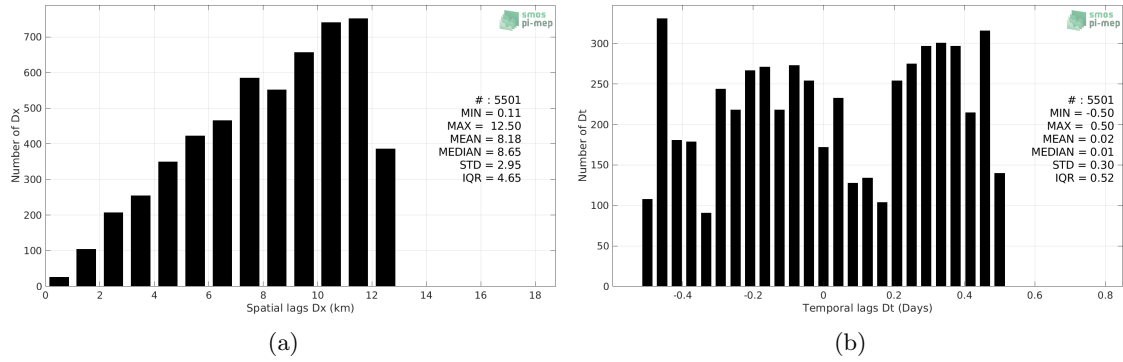
Figure 5: Histograms of the spatial (a) and temporal (b) lags between the location/time of the TSG (GOSUD-Sailing-ship) measurement and the date of the corresponding CCI SSS L4 Merged-OI v2.31 - 7-day running (ESA) SSS pixel.
