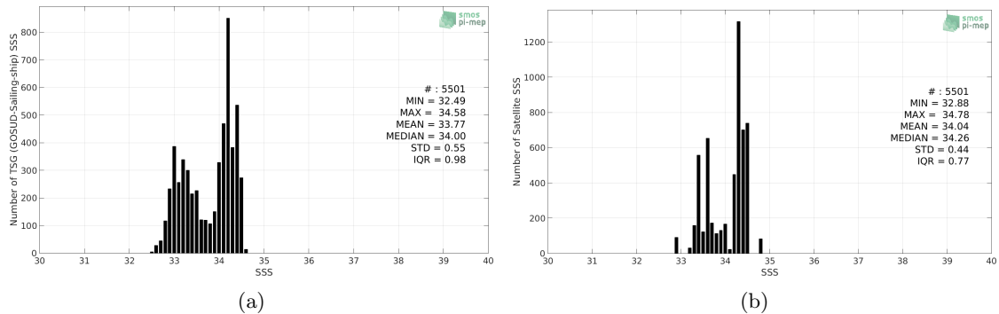
Figure 2: Histograms of SSS from TSG (GOSUD-Sailing-ship) (a) and CCI L4 Merged-OI v2.31 - 7-day running (ESA) (b) considering all match-up pairs per bins of 0.1 over the SPURS 2 Pi-MEP region and for the full satellite product period.
