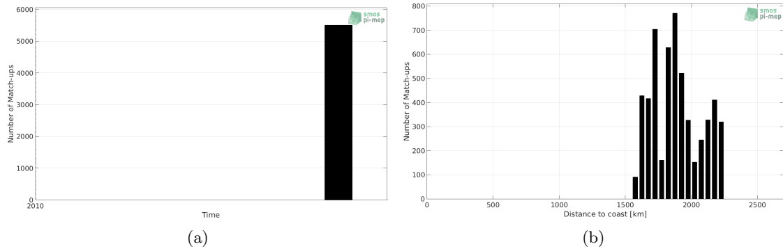
Figure 1: Number of match-ups between TSG (GOSUD-Sailing-ship) and CCI L4 Merged-OI v2.31 - 7-day running (ESA) SSS as a function of time (a) and as function of the distance to coast (b) over the SPURS 2 Pi-MEP region and for the full satellite product period.
