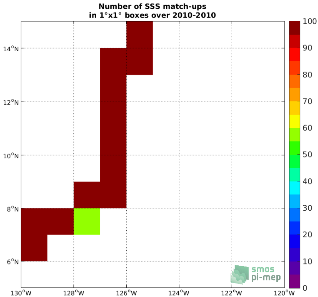
Figure 4: Number of SSS match-ups between TSG (GOSUD-Sailing-ship) SSS and the CCI L4 Merged-OI v2.31 - 7-day running (ESA) SSS product for the SPURS 2 Pi-MEP region over 1°x1° boxes and for the full satellite product period.
