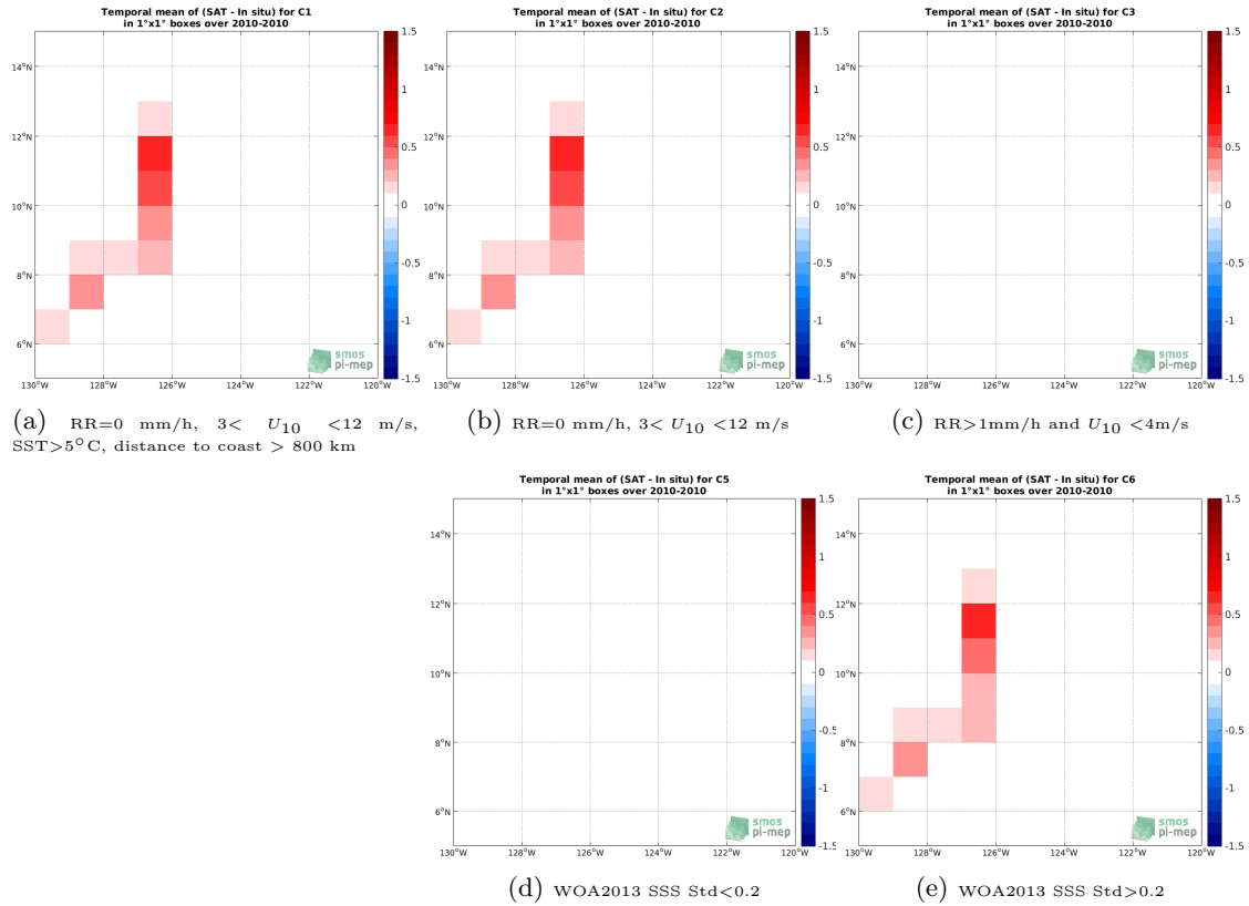
Figure 12: Temporal mean gridded over spatial boxes of size 1^\circ \times 1^\circ of \Delta SSS (CCI L4 Merged-OI v2.31 - 7-day running (ESA) - TSG (GOSUD-Sailing-ship)) for 5 different subdatasets corresponding to:RR=0 mm/h, 3 < U_{10} < 12 m/s, SST>5°C, distance to coast > 800 km (a), RR=0 mm/h, 3 < U_{10} < 12 m/s (b), RR>1mm/h and U_{10} < 4 m/s (c), WOA2013 SSS Std<0.2 (d), WOA2013 SSS Std>0.2 (e).
