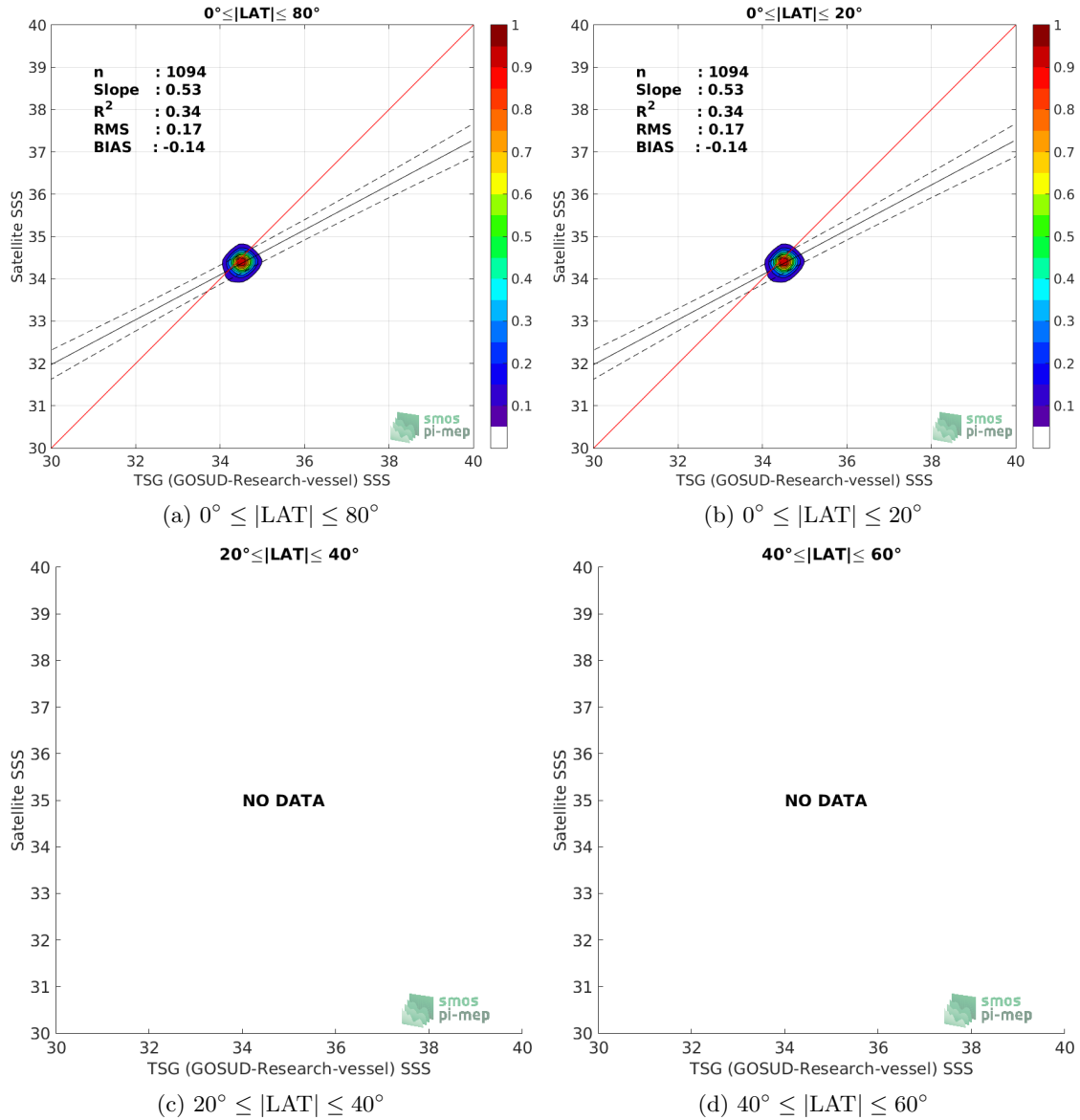
Figure 9: Contour maps of the concentration of CCI SSS L4 Merged-OI v2.31 - 7-day running (ESA) SSS ( y -axis) versus TSG (GOSUD-Research-vessel) SSS ( x -axis) at match-up pairs for different latitude bands. For each plot, the red line shows x=y . The black thin and dashed lines indicate a linear fit through the data cloud and the \pm 95\% confidence levels, respectively. The number match-up pairs n , the slope and R^2 coefficient of the linear fit, the root mean square (RMS) and the mean bias between satellite and in situ data are indicated for each latitude band in each plots.
