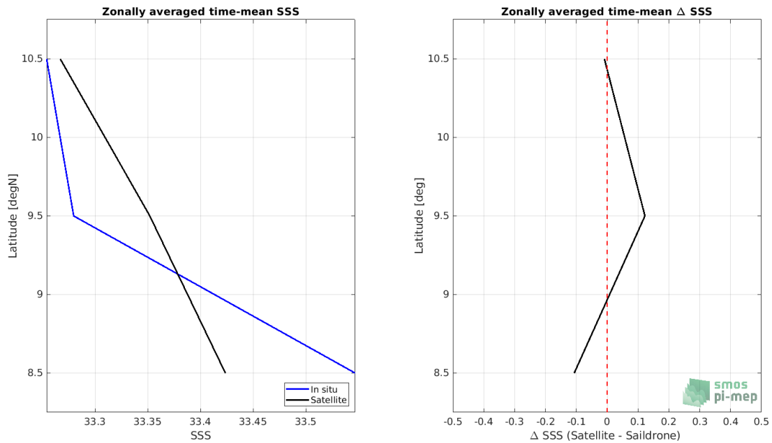
Figure 7: Left panel: Zonal mean SSS from CCI SSS L4 Merged-OI v2.31 - 7-day running (ESA) satellite product (black) and from Sairdron (blue). Right panel: Zonal mean of \Delta SSS (Satellite - Sairdron) for all the collected Pi-MEP match-up pairs estimated over the full satellite product period.
