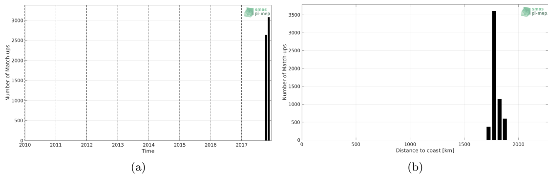
Figure 1: Number of match-ups between Saildrone and CCI SSS L4 Merged-OI v2.31 - 7-day running (ESA) SSS as a function of time (a) and as function of the distance to coast (b) over the SPURS 2 Pi-MEP region and for the full satellite product period.
