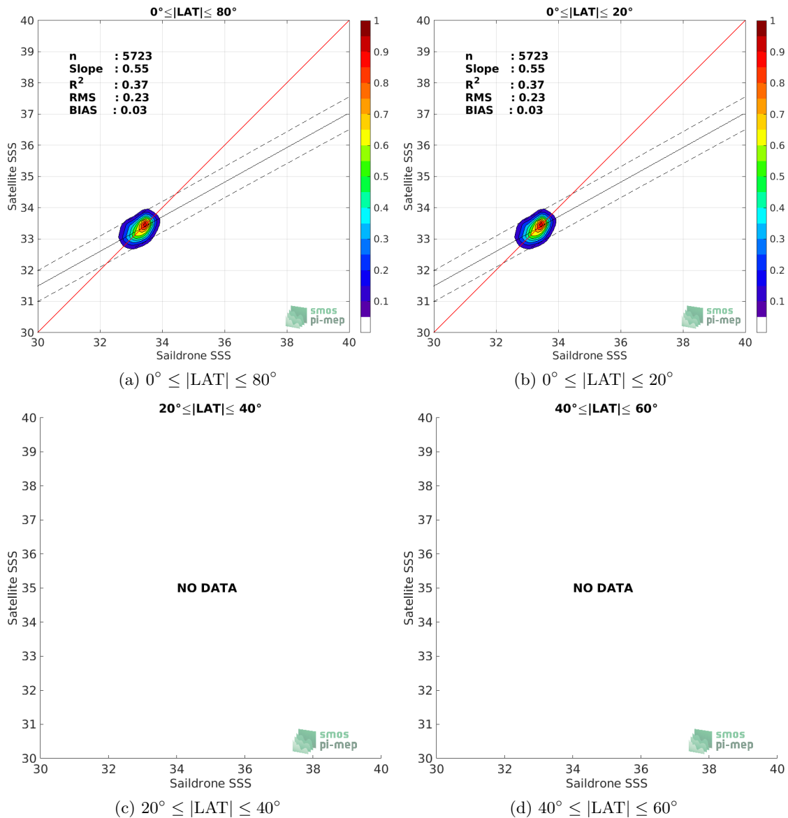
Figure 8: Contour maps of the concentration of CCI SSS L4 Merged-OI v2.31 - 7-day running (ESA) SSS (y-axis) versus Saildrone SSS (x-axis) at match-up pairs for different latitude bands. For each plot, the red line shows x=y . The black thin and dashed lines indicate a linear fit through the data cloud and the \pm 95\% confidence levels, respectively. The number match-up pairs n , the slope and R^2 coefficient of the linear fit, the root mean square (RMS) and the mean bias between satellite and in situ data are indicated for each latitude band in each plots.
