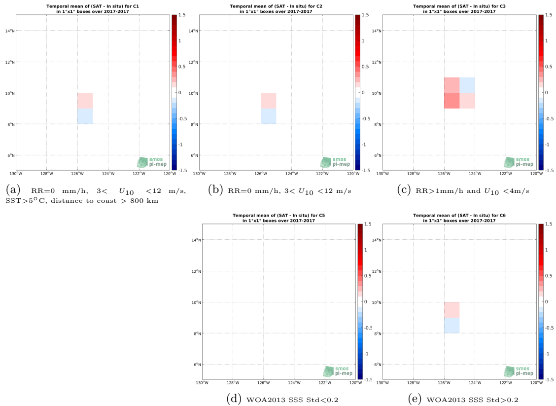
Figure 11: Temporal mean gridded over spatial boxes of size 1^\circ \times 1^\circ of \Delta SSS (CCI SSS L4 Merged-OI v2.31 - 7-day running (ESA) - Saildrone) for 5 different subdatasets corresponding to:RR=0 mm/h, 3 < U_{10} < 12 m/s, SST >5^\circ\text{C} , distance to coast > 800 km (a), RR=0 mm/h, 3 < U_{10} < 12 m/s (b), RR >1 mm/h and U_{10} < 4 m/s (c), WOA2013 SSS Std <0.2 (d), WOA2013 SSS Std >0.2 (e).
