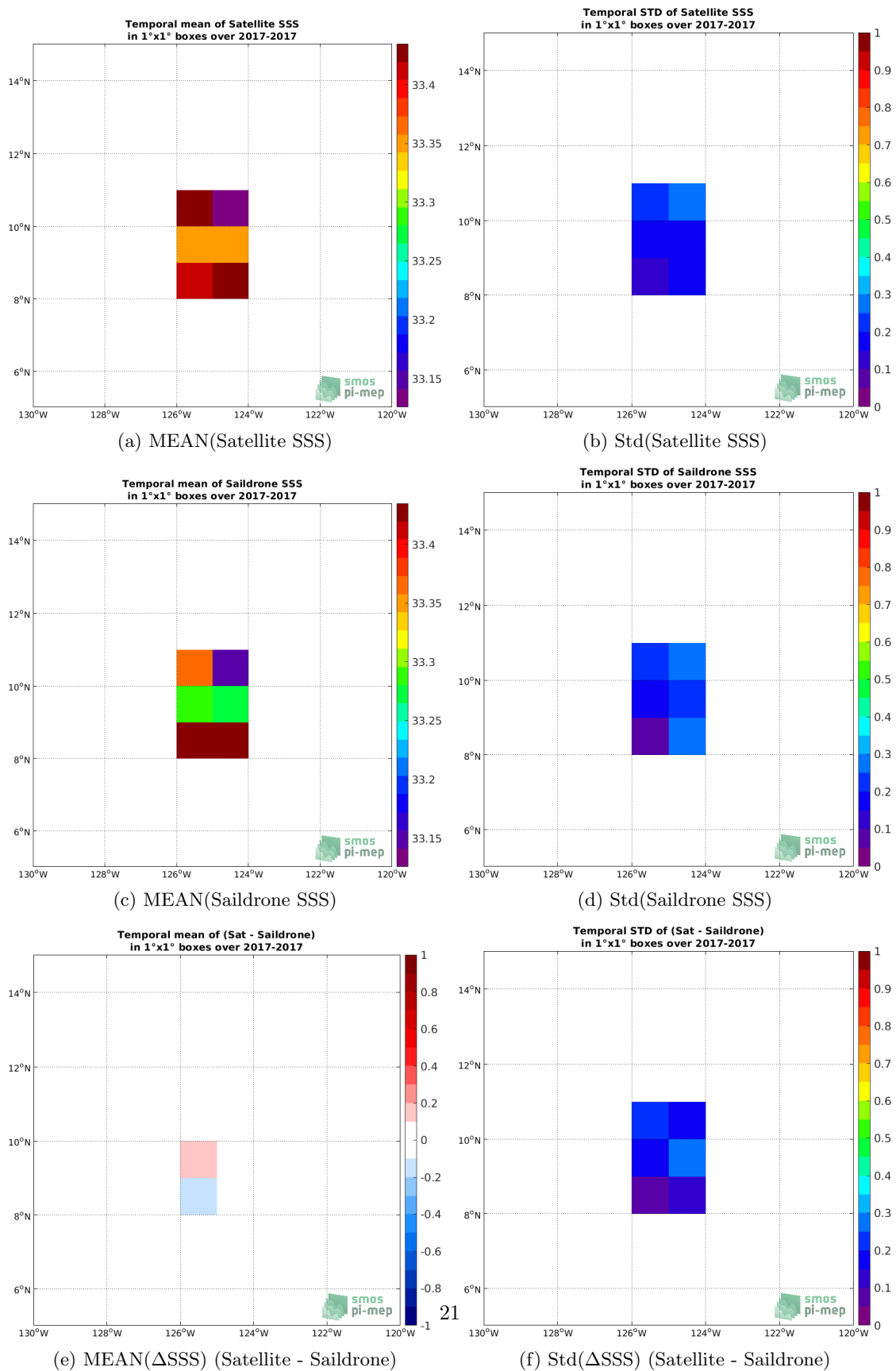
Figure 5: Temporal mean (left) and Std (right) of SSS from CCI SSS L4 Merged-OI v2.31 - 7-day running (ESA) (top), Saildrone (middle), and of \Delta SSS (Satellite - Saildrone). Only match-up pairs are used to generate these maps.
