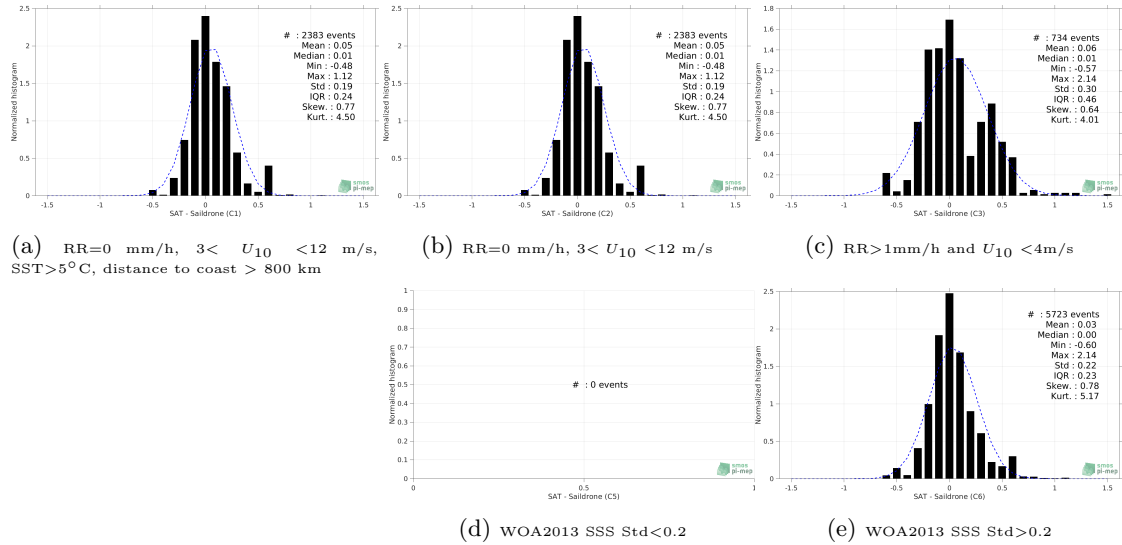
Figure 12: Normalized histogram of \Delta SSS (CCI SSS L4 Merged-OI v2.31 - 7-day running (ESA) - Saildrone) for 5 different subdatasets corresponding to: RR=0 mm/h, 3 < U_{10} < 12 m/s, SST > 5°C, distance to coast > 800 km (a), RR=0 mm/h, 3 < U_{10} < 12 m/s (b), RR > 1mm/h and U_{10} < 4 m/s (c), WOA2013 SSS Std < 0.2 (d), WOA2013 SSS Std > 0.2 (e).
