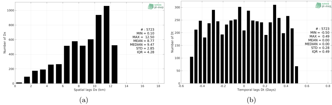
Figure 4: Histograms of the spatial (a) and temporal (b) lags between the location/time of the Saildrone measurement and the date of the corresponding CCI SSS L4 Merged-OI v2.31 - 7-day running (ESA) SSS pixel.
