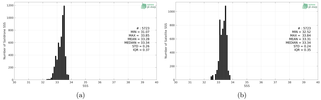
Figure 2: Histograms of SSS from Sairdrone (a) and CCI SSS L4 Merged-OI v2.31 - 7-day running (ESA) (b) considering all match-up pairs per bins of 0.1 over the SPURS 2 Pi-MEP region and for the full satellite product period.
