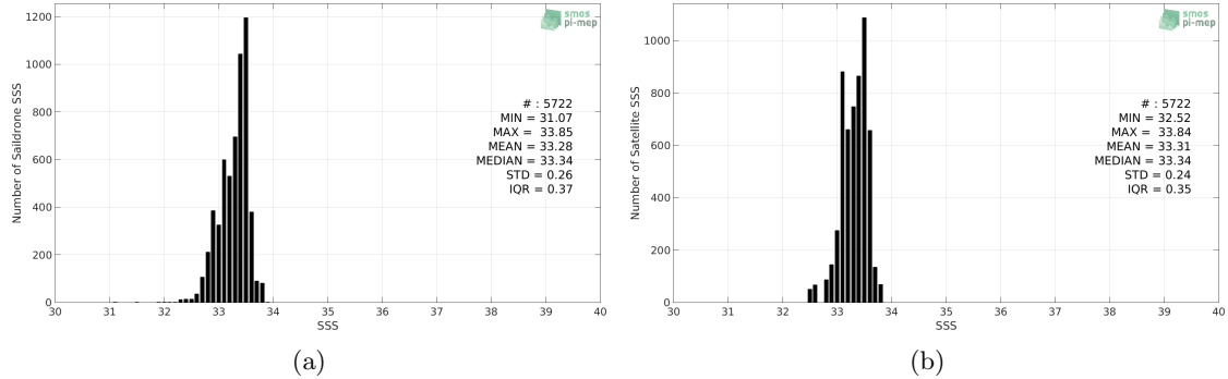
Figure 2: Histograms of SSS from Saildrone (a) and CCI SSS L4 Merged-OI v2.31 - 7-day running (ESA) (b) considering all match-up pairs per bins of 0.1 over the SPURS 2 Pi-MEP region and for the full satellite product period.
