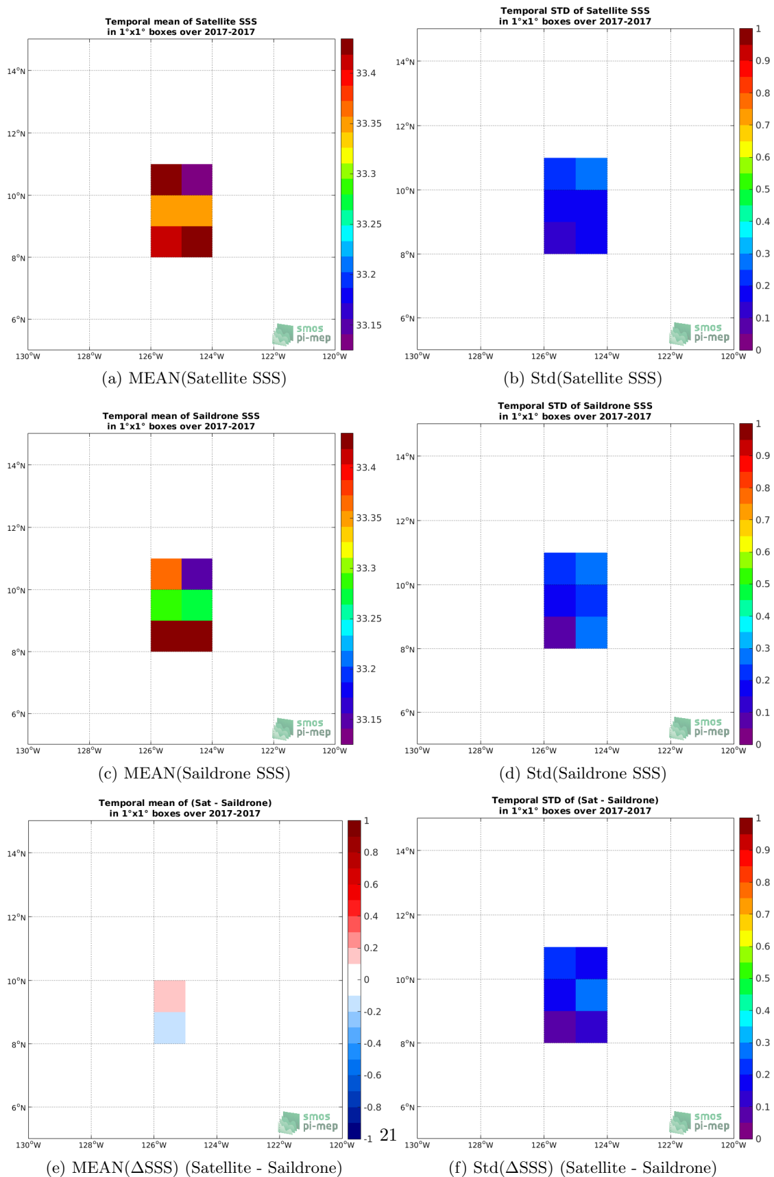
Figure 6: Temporal mean (left) and Std (right) of SSS from CCI SSS L4 Merged-OI v2.31 - 7-day running (ESA) (top), Saildrone (middle), and of \Delta SSS (Satellite - Saildrone). Only match-up pairs are used to generate these maps.
