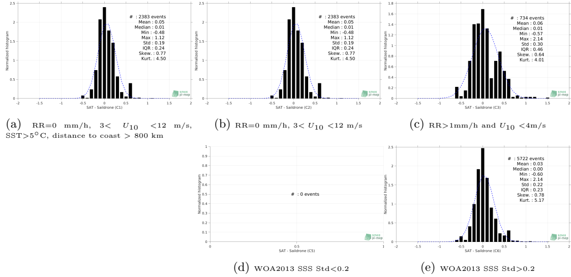
Figure 13: Normalized histogram of \Delta SSS (CCI SSS L4 Merged-OI v2.31 - 7-day running (ESA) - Saildrone) for 5 different subdatasets corresponding to: RR=0 mm/h, 3 < U_{10} < 12 m/s, SST > 5°C, distance to coast > 800 km (a), RR=0 mm/h, 3 < U_{10} < 12 m/s (b), RR > 1mm/h and U_{10} < 4 m/s (c), WOA2013 SSS Std < 0.2 (d), WOA2013 SSS Std > 0.2 (e).
