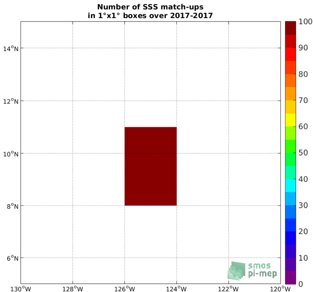
Figure 4: Number of SSS match-ups between Saildrone SSS and the CCI SSS L4 Merged-OI v2.31 - 7-day running (ESA) SSS product for the SPURS 2 Pi-MEP region over 1°x1° boxes and for the full satellite product period.
