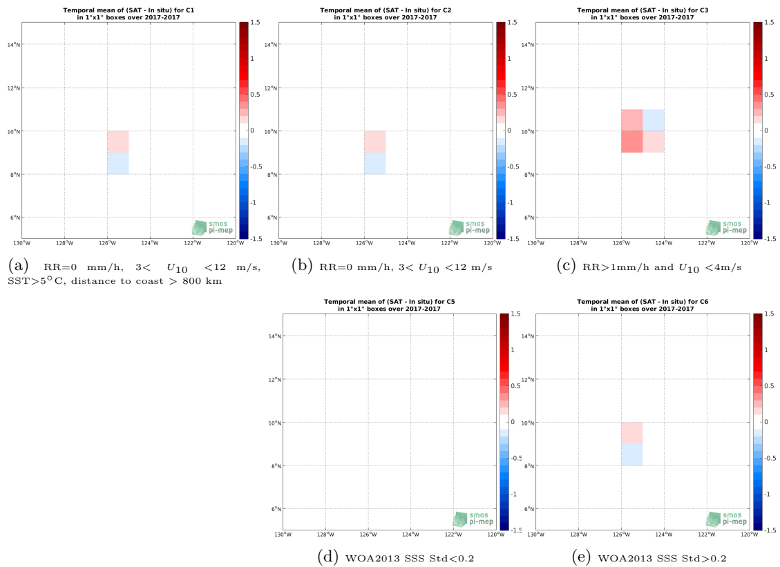
Figure 12: Temporal mean gridded over spatial boxes of size 1^\circ \times 1^\circ of \Delta SSS (CCI SSS L4 Merged-OI v2.31 - 7-day running (ESA) - Saildrone) for 5 different subdatasets corresponding to:RR=0 mm/h, 3 < U_{10} < 12 m/s, SST >5^\circ\text{C} , distance to coast > 800 km (a), RR=0 mm/h, 3 < U_{10} < 12 m/s (b), RR >1 mm/h and U_{10} < 4 m/s (c), WOA2013 SSS Std <0.2 (d), WOA2013 SSS Std >0.2 (e).
