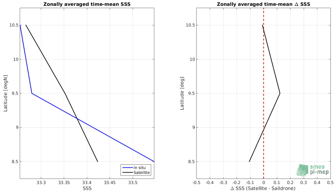
Figure 8: Left panel: Zonal mean SSS from CCI SSS L4 Merged-OI v2.31 - 7-day running (ESA) satellite product (black) and from Sairdrone (blue). Right panel: Zonal mean of \Delta SSS (Satellite - Sairdrone) for all the collected Pi-MEP match-up pairs estimated over the full satellite product period.
