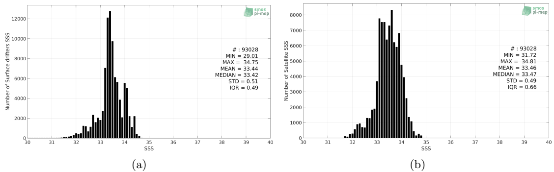
Figure 2: Histograms of SSS from Surface drifters (a) and CCI SSS L4 Merged-OI v2.31 - 7-day running (ESA) (b) considering all match-up pairs per bins of 0.1 over the SPURS 2 Pi-MEP region and for the full satellite product period.
