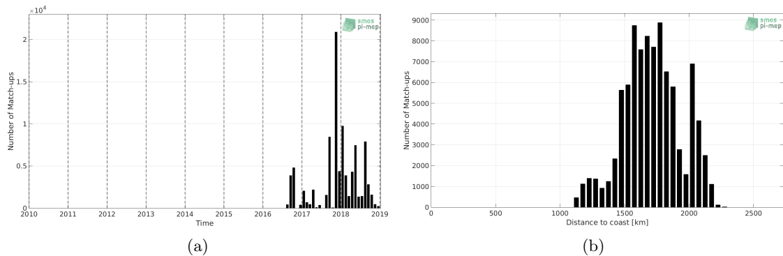
Figure 1: Number of match-ups between Surface drifters and CCI SSS L4 Merged-OI v2.31 - 7-day running (ESA) SSS as a function of time (a) and as function of the distance to coast (b) over the SPURS 2 Pi-MEP region and for the full satellite product period.
