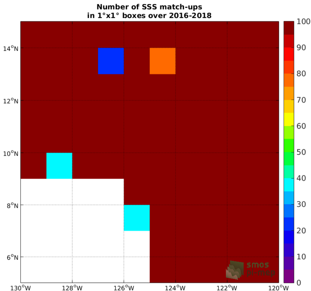
Figure 3: Number of SSS match-ups between Surface drifters SSS and the CCI SSS L4 Merged-OI v2.31 - 7-day running (ESA) SSS product for the SPURS 2 Pi-MEP region over 1°x1° boxes and for the full satellite product period.
