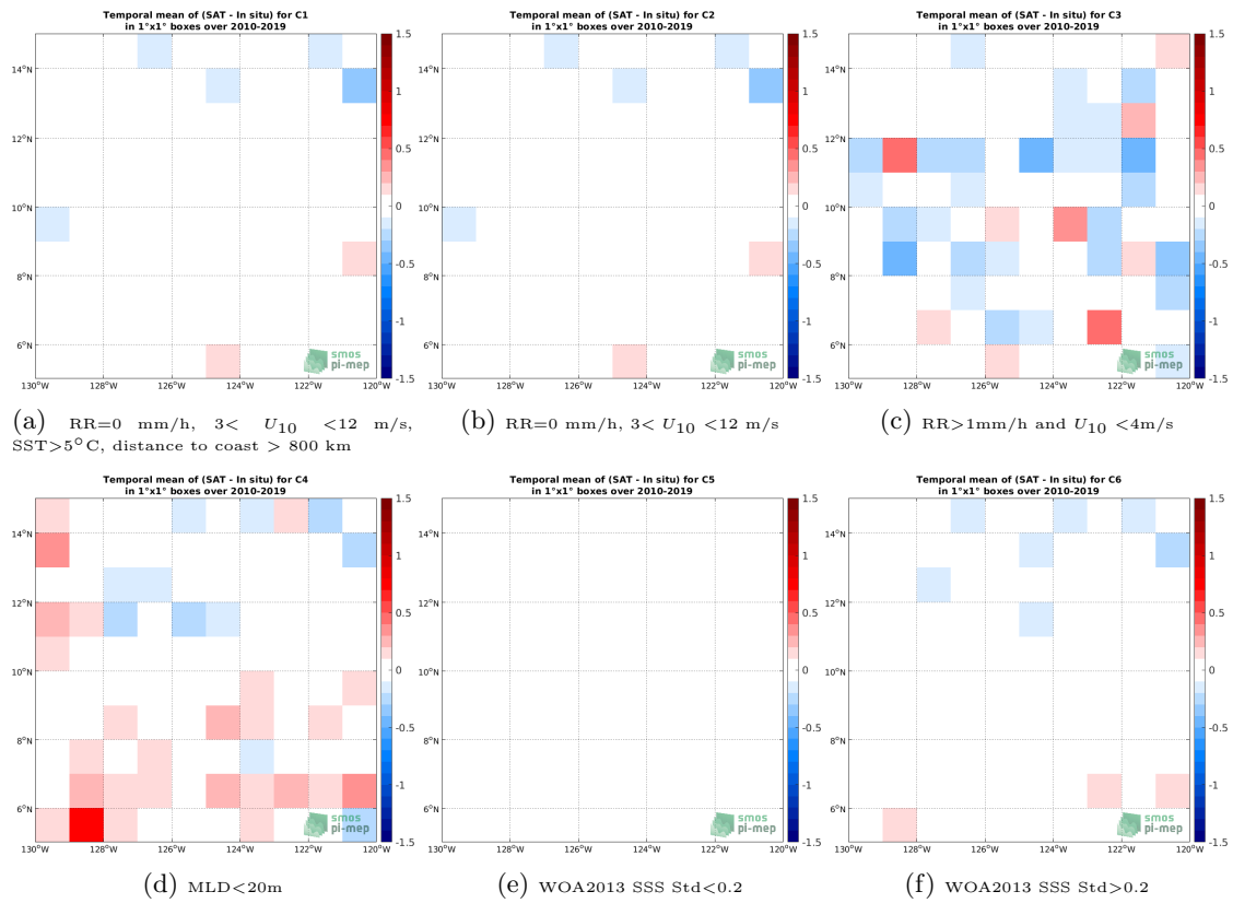
Figure 12: Temporal mean gridded over spatial boxes of size 1^\circ \times 1^\circ of \Delta SSS (CCI SSS L4 Merged-OI v2.31 - 7-day running (ESA) - Argo) for 6 different subdatasets corresponding to:RR=0 mm/h, 3 < U_{10} < 12 m/s, SST >5^\circ C, distance to coast > 800 km (a), RR=0 mm/h, 3 < U_{10} < 12 m/s (b), RR >1 mm/h and U_{10} < 4 m/s (c),MLD <20 m (d),WOA2013 SSS Std <0.2 (e),WOA2013 SSS Std >0.2 (f).
