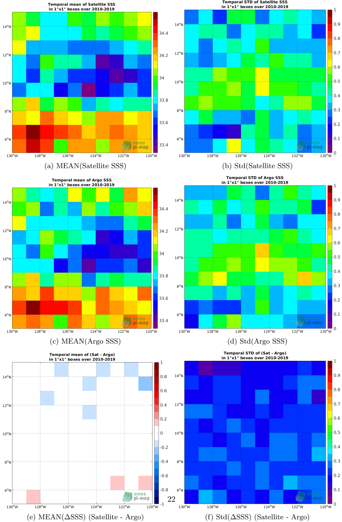
Figure 6: Temporal mean (left) and Std (right) of SSS from CCI SSS L4 Merged-OI v2.31 - 7-day running (ESA) (top), Argo (middle), and of \Delta SSS (Satellite - Argo). Only match-up pairs are used to generate these maps.
