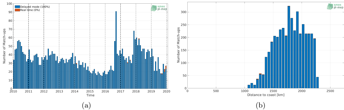
Figure 1: Number of match-ups between Argo and CCI SSS L4 Merged-OI v2.31 - 7-day running (ESA) SSS as a function of time (a) and as function of the distance to coast (b) over the SPURS 2 Pi-MEP region and for the full satellite product period.
