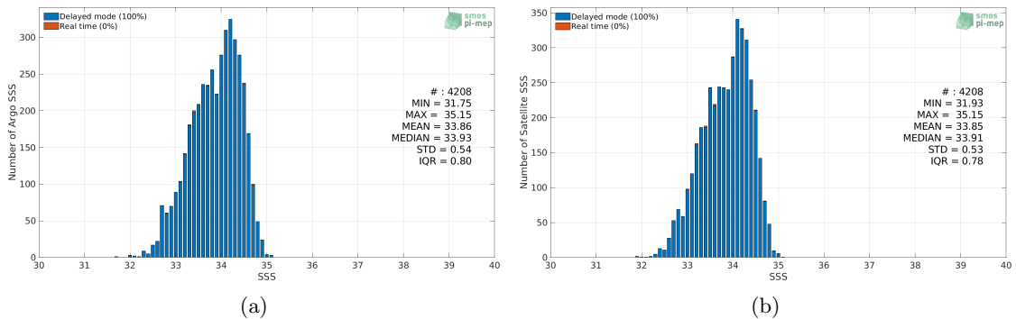
Figure 2: Histograms of SSS from Argo (a) and CCI SSS L4 Merged-OI v2.31 - 7-day running (ESA) (b) considering all match-up pairs per bins of 0.1 over the SPURS 2 Pi-MEP region and for the full satellite product period.
