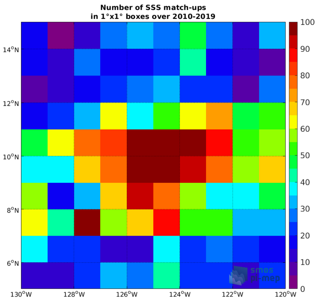
Figure 4: Number of SSS match-ups between Argo SSS and the CCI SSS L4 Merged-OI v2.31 - 7-day running (ESA) SSS product for the SPURS 2 Pi-MEP region over 1°x1° boxes and for the full satellite product period.
