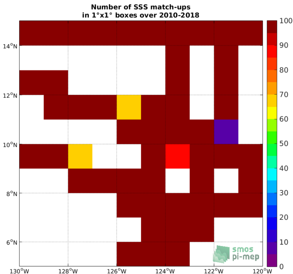
Figure 4: Number of SSS match-ups between TSG (SAMOS) SSS and the CCI L4 Merged-OI v2.31 - 30-day running (ESA) SSS product for the SPURS 2 Pi-MEP region over 1°x1° boxes and for the full satellite product period.
