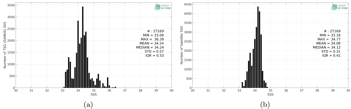
Figure 2: Histograms of SSS from TSG (SAMOS) (a) and CCI L4 Merged-OI v2.31 - 30-day running (ESA) (b) considering all match-up pairs per bins of 0.1 over the SPURS 2 Pi-MEP region and for the full satellite product period.
