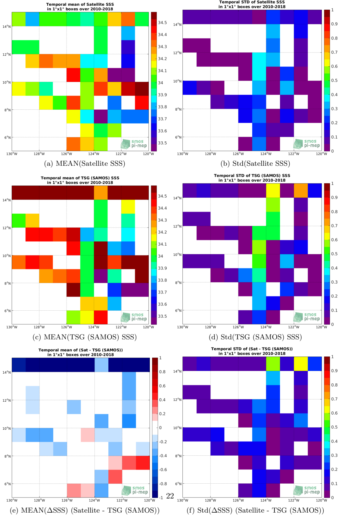
Figure 6: Temporal mean (left) and Std (right) of SSS from CCI L4 Merged-OI v2.31 - 30-day running (ESA) (top), TSG (SAMOS) (middle), and of \Delta SSS (Satellite - TSG (SAMOS)). Only match-up pairs are used to generate these maps.
