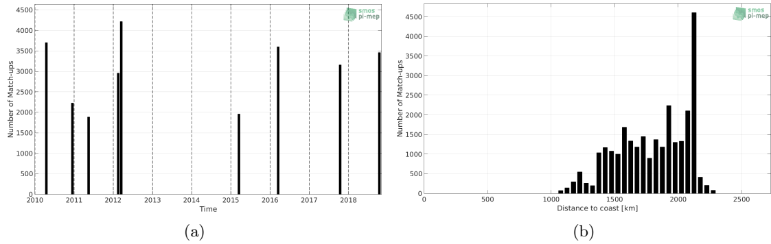
Figure 1: Number of match-ups between TSG (SAMOS) and CCI L4 Merged-OI v2.31 - 30-day running (ESA) SSS as a function of time (a) and as function of the distance to coast (b) over the SPURS 2 Pi-MEP region and for the full satellite product period.
