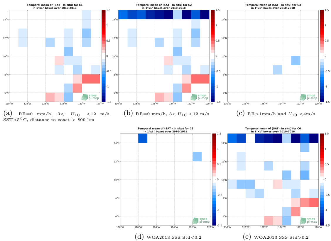
Figure 12: Temporal mean gridded over spatial boxes of size 1^\circ \times 1^\circ of \Delta SSS (CCI L4 Merged-OI v2.31 - 30-day running (ESA) - TSG (SAMOS)) for 5 different subdatasets corresponding to:RR=0 mm/h, 3 < U_{10} < 12 m/s, SST >5^\circ\text{C} , distance to coast > 800 km (a), RR=0 mm/h, 3 < U_{10} < 12 m/s (b), RR >1 mm/h and U_{10} < 4 m/s (c), WOA2013 SSS Std <0.2 (d), WOA2013 SSS Std >0.2 (e).
