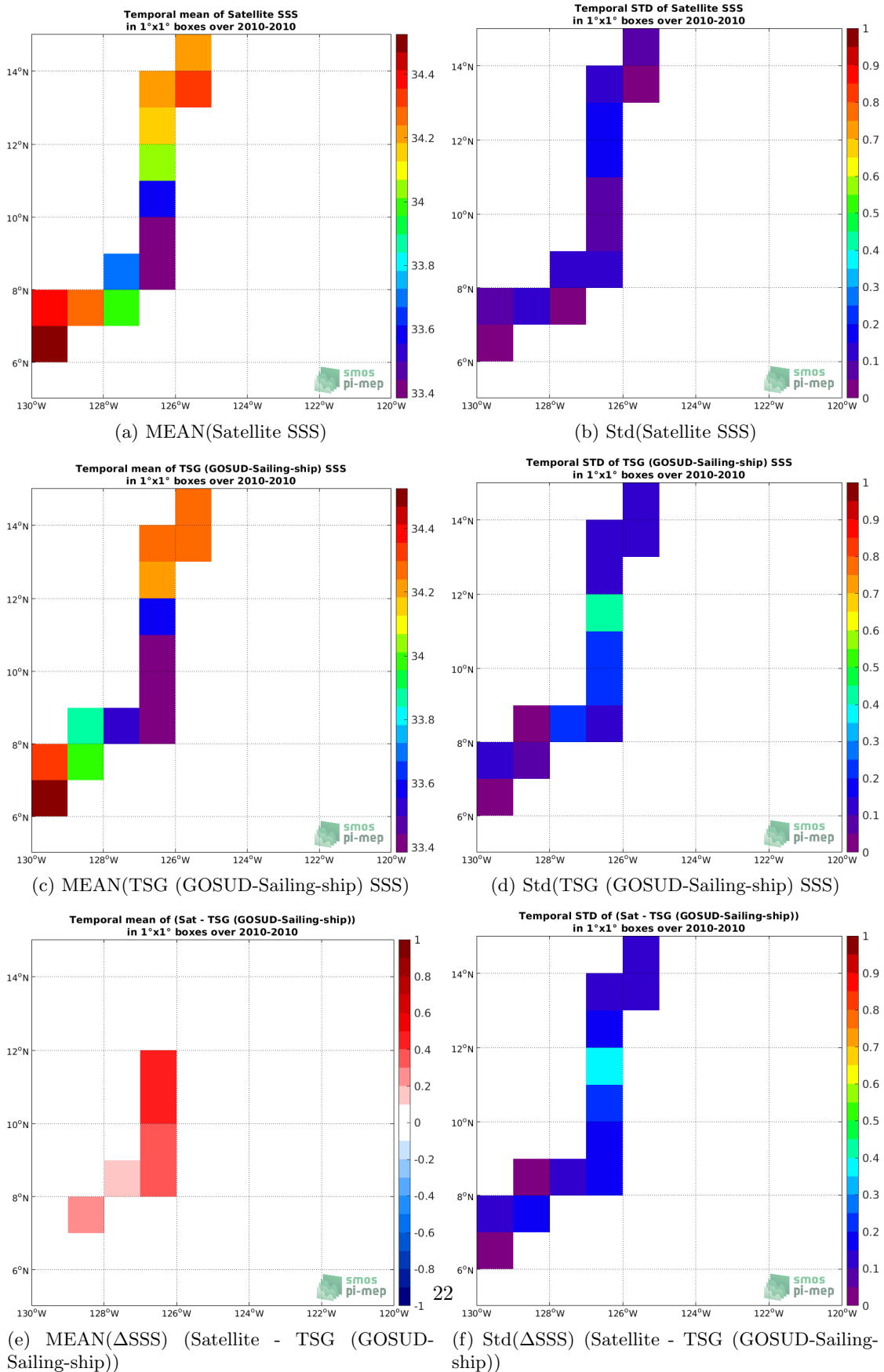
Figure 6: Temporal mean (left) and Std (right) of SSS from CCI SSS L4 Merged-OI v2.31 - 30-day running (ESA) (top), TSG (GOSUD-Sailing-ship) (middle), and of \Delta SSS (Satellite - TSG (GOSUD-Sailing-ship)). Only match-up pairs are used to generate these maps.
