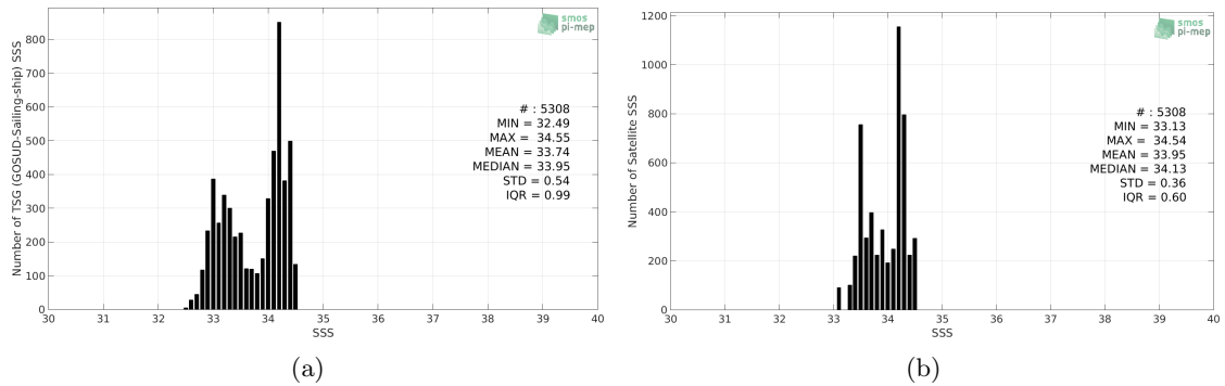
Figure 2: Histograms of SSS from TSG (GOSUD-Sailing-ship) (a) and CCI SSS L4 Merged-OI v2.31 - 30-day running (ESA) (b) considering all match-up pairs per bins of 0.1 over the SPURS 2 Pi-MEP region and for the full satellite product period.
