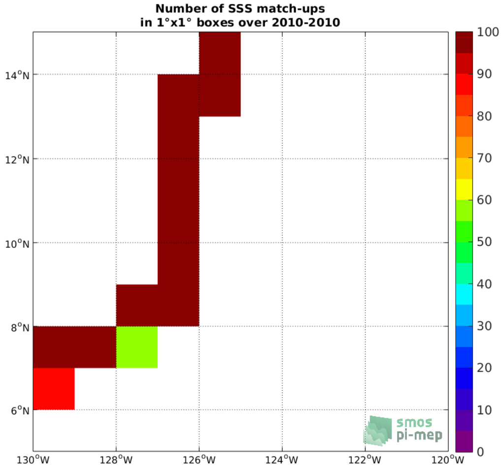
Figure 4: Number of SSS match-ups between TSG (GOSUD-Sailing-ship) SSS and the CCI SSS L4 Merged-OI v2.31 - 30-day running (ESA) SSS product for the SPURS 2 Pi-MEP region over 1°x1° boxes and for the full satellite product period.
