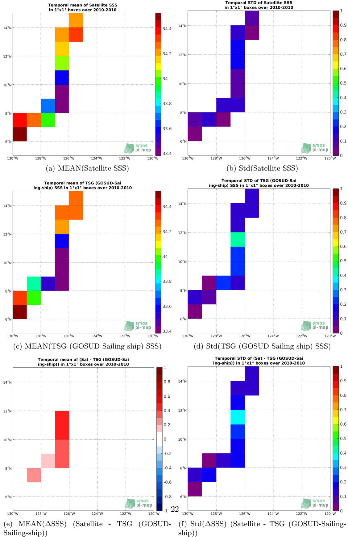
Figure 6: Temporal mean (left) and Std (right) of SSS from CCI L4 Merged-OI v2.31 - 30-day running (ESA) (top), TSG (GOSUD-Sailing-ship) (middle), and of \Delta SSS (Satellite - TSG (GOSUD-Sailing-ship)). Only match-up pairs are used to generate these maps.
