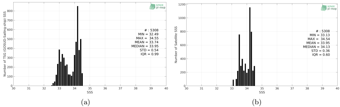
Figure 2: Histograms of SSS from TSG (GOSUD-Sailing-ship) (a) and CCI L4 Merged-OI v2.31 - 30-day running (ESA) (b) considering all match-up pairs per bins of 0.1 over the SPURS 2 Pi-MEP region and for the full satellite product period.
