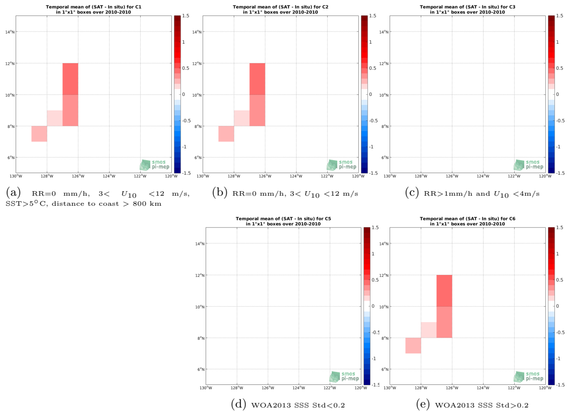
Figure 12: Temporal mean gridded over spatial boxes of size 1^\circ \times 1^\circ of \Delta SSS (CCI L4 Merged-OI v2.31 - 30-day running (ESA) - TSG (GOSUD-Sailing-ship)) for 5 different subdatasets corresponding to:RR=0 mm/h, 3 < U_{10} < 12 m/s, SST>5°C, distance to coast > 800 km (a), RR=0 mm/h, 3 < U_{10} < 12 m/s (b), RR>1mm/h and U_{10} < 4 m/s (c), WOA2013 SSS Std<0.2 (d), WOA2013 SSS Std>0.2 (e).
