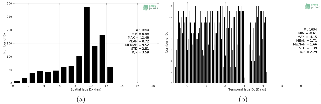
Figure 5: Histograms of the spatial (a) and temporal (b) lags between the location/time of the TSG (GOSUD-Research-vessel) measurement and the date of the corresponding CCI SSS L4 Merged-OI v2.31 - 30-day running (ESA) SSS pixel.
