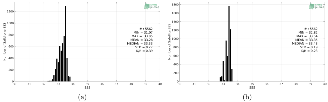
Figure 2: Histograms of SSS from Sairdrone (a) and CCI SSS L4 Merged-OI v2.31 - 30-day running (ESA) (b) considering all match-up pairs per bins of 0.1 over the SPURS 2 Pi-MEP region and for the full satellite product period.
