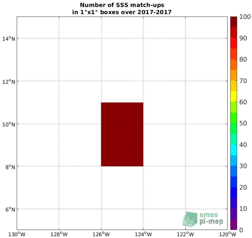
Figure 3: Number of SSS match-ups between Saildrone SSS and the CCI SSS L4 Merged-OI v2.31 - 30-day running (ESA) SSS product for the SPURS 2 Pi-MEP region over 1°x1° boxes and for the full satellite product period.
