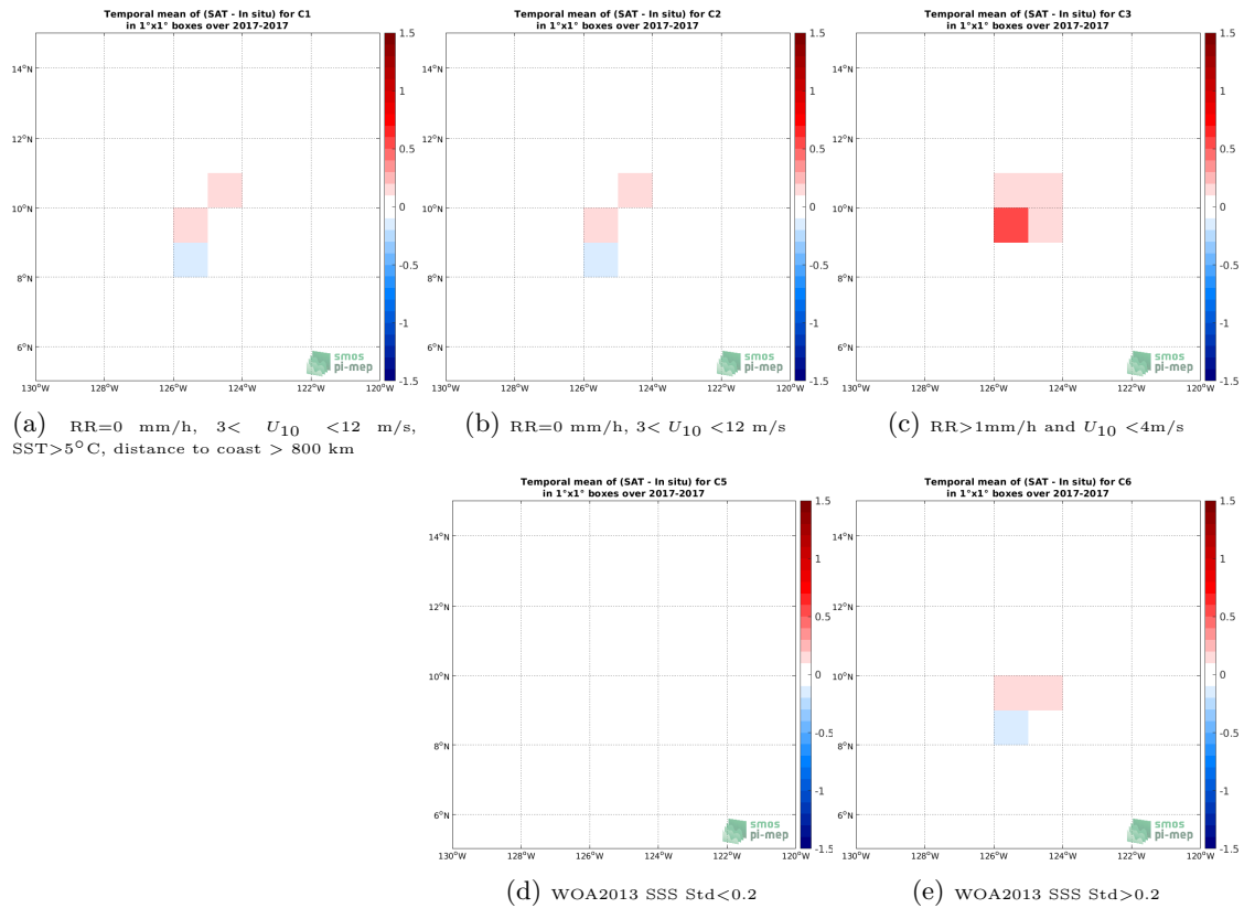
Figure 11: Temporal mean gridded over spatial boxes of size 1^\circ \times 1^\circ of \Delta SSS (CCI SSS L4 Merged-OI v2.31 - 30-day running (ESA) - Saildrone) for 5 different subdatasets corresponding to:RR=0 mm/h, 3 < U_{10} < 12 m/s, SST >5^\circ\text{C} , distance to coast > 800 km (a), RR=0 mm/h, 3 < U_{10} < 12 m/s (b), RR >1 mm/h and U_{10} < 4 m/s (c), WOA2013 SSS Std <0.2 (d), WOA2013 SSS Std >0.2 (e).
