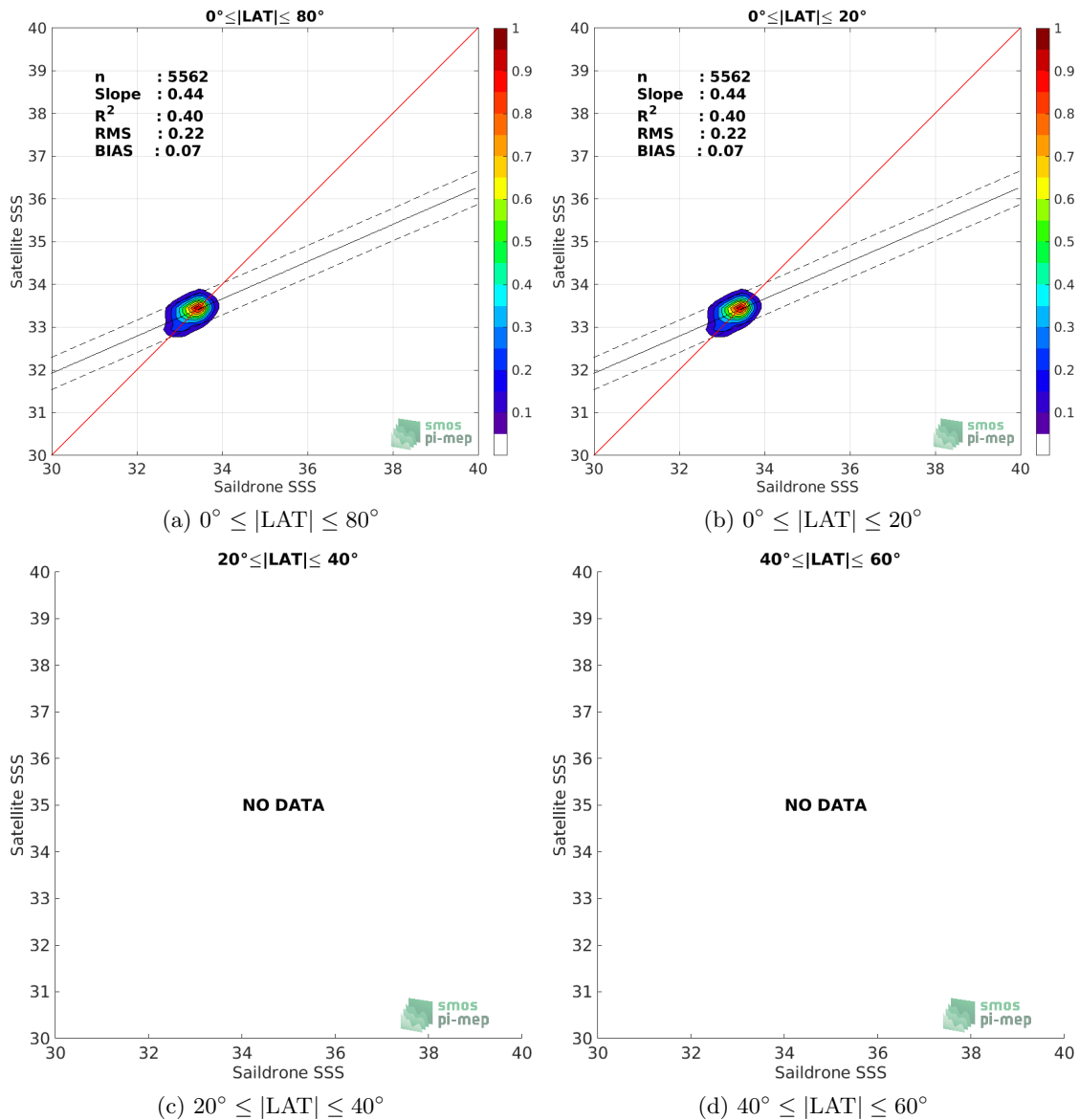
Figure 8: Contour maps of the concentration of CCI SSS L4 Merged-OI v2.31 - 30-day running (ESA) SSS (y-axis) versus Saildrone SSS (x-axis) at match-up pairs for different latitude bands. For each plot, the red line shows x=y . The black thin and dashed lines indicate a linear fit through the data cloud and the \pm 95\% confidence levels, respectively. The number match-up pairs n , the slope and R^2 coefficient of the linear fit, the root mean square (RMS) and the mean bias between satellite and in situ data are indicated for each latitude band in each plots.
