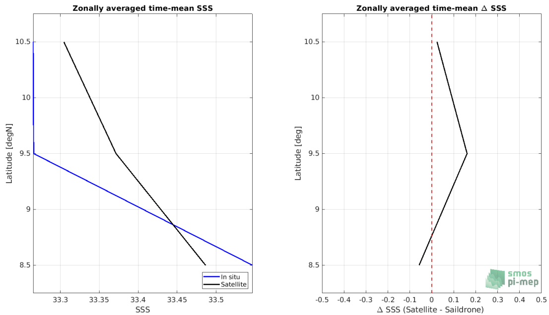
Figure 7: Left panel: Zonal mean SSS from CCI SSS L4 Merged-OI v2.31 - 30-day running (ESA) satellite product (black) and from Sairdron (blue). Right panel: Zonal mean of \Delta SSS (Satellite - Sairdron) for all the collected Pi-MEP match-up pairs estimated over the full satellite product period.
