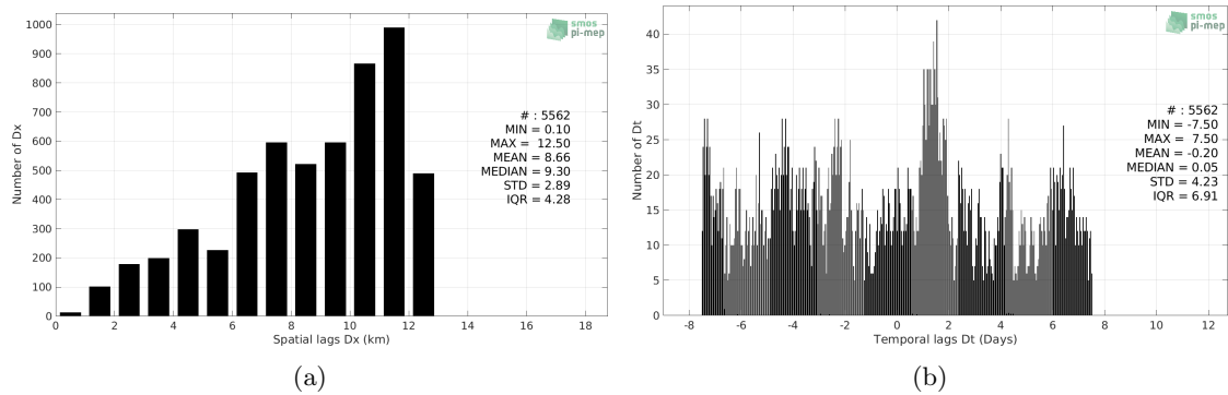
Figure 4: Histograms of the spatial (a) and temporal (b) lags between the location/time of the Saildrone measurement and the date of the corresponding CCI SSS L4 Merged-OI v2.31 - 30-day running (ESA) SSS pixel.
