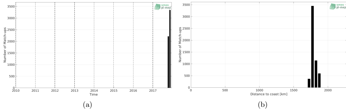
Figure 1: Number of match-ups between Saildrone and CCI SSS L4 Merged-OI v2.31 - 30-day running (ESA) SSS as a function of time (a) and as function of the distance to coast (b) over the SPURS 2 Pi-MEP region and for the full satellite product period.
