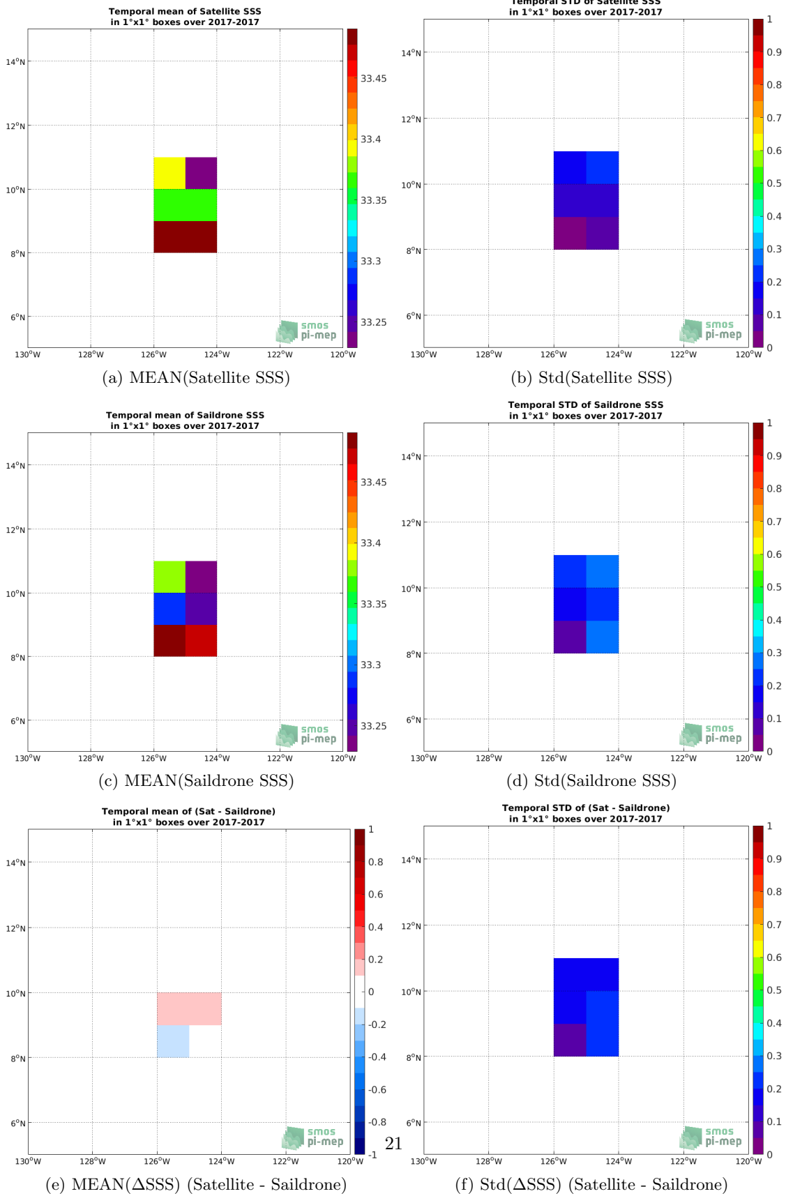
Figure 5: Temporal mean (left) and Std (right) of SSS from CCI SSS L4 Merged-OI v2.31 - 30-day running (ESA) (top), Saildrone (middle), and of \Delta SSS (Satellite - Saildrone). Only match-up pairs are used to generate these maps.
