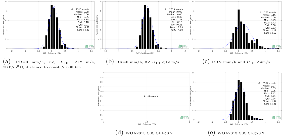
Figure 12: Normalized histogram of \Delta SSS (CCI SSS L4 Merged-OI v2.31 - 30-day running (ESA) - Saildrone) for 5 different subdatasets corresponding to: RR=0 mm/h, 3 < U_{10} < 12 m/s, SST > 5°C, distance to coast > 800 km (a), RR=0 mm/h, 3 < U_{10} < 12 m/s (b), RR > 1mm/h and U_{10} < 4 m/s (c), WOA2013 SSS Std < 0.2 (d), WOA2013 SSS Std > 0.2 (e).
