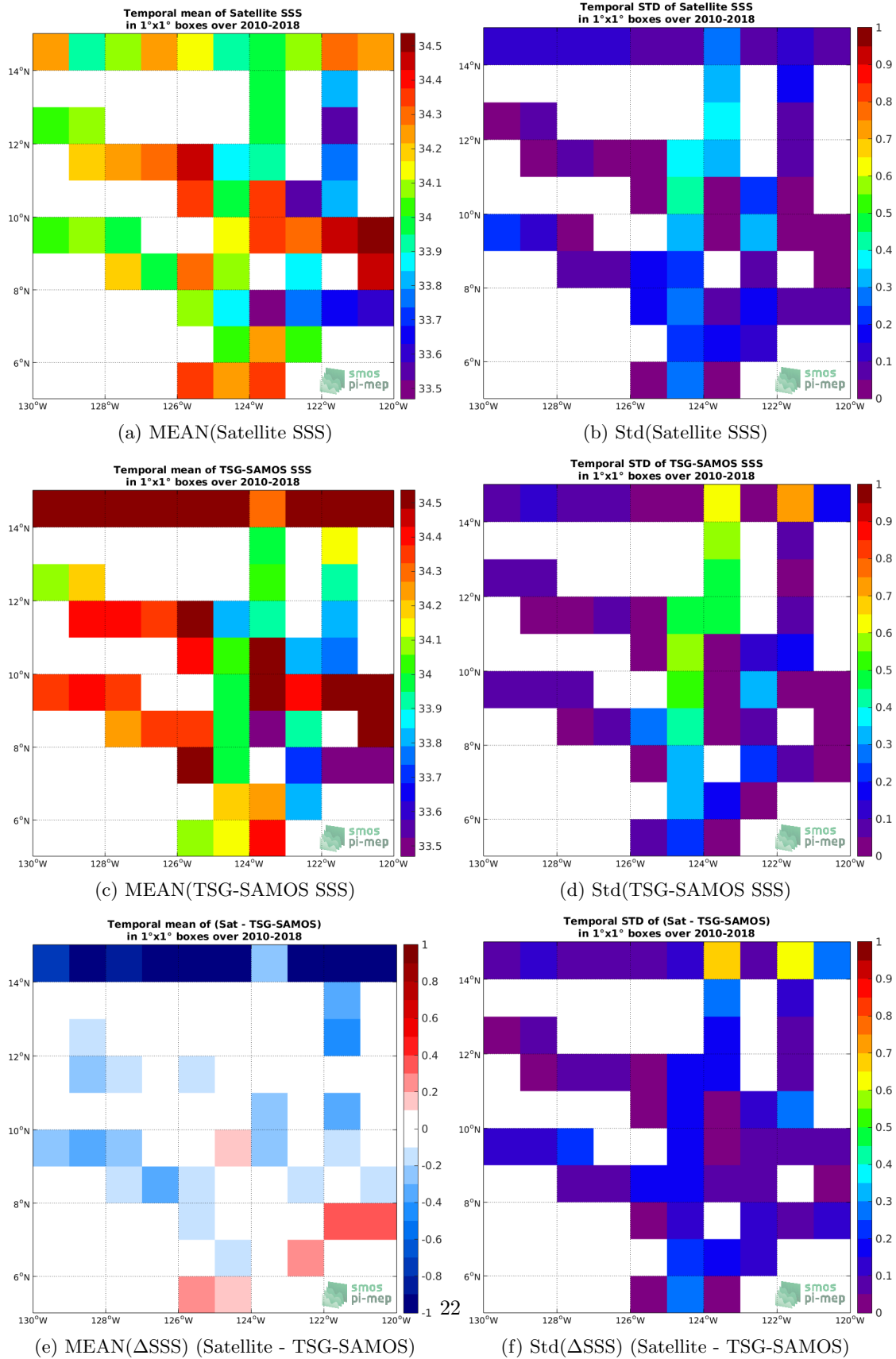
Figure 6: Temporal mean (left) and Std (right) of SSS from CCI L4 Merged-OI v1.8 - 7-day running (ESA) (top), TSG-SAMOS (middle), and of \Delta SSS (Satellite - TSG-SAMOS). Only match-up pairs are used to generate these maps.
