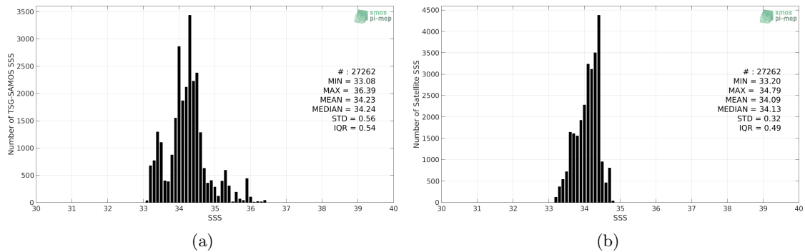
Figure 2: Histograms of SSS from TSG-SAMOS (a) and CCI L4 Merged-OI v1.8 - 7-day running (ESA) (b) considering all match-up pairs per bins of 0.1 over the SPURS 2 Pi-MEP region and for the full satellite product period.
