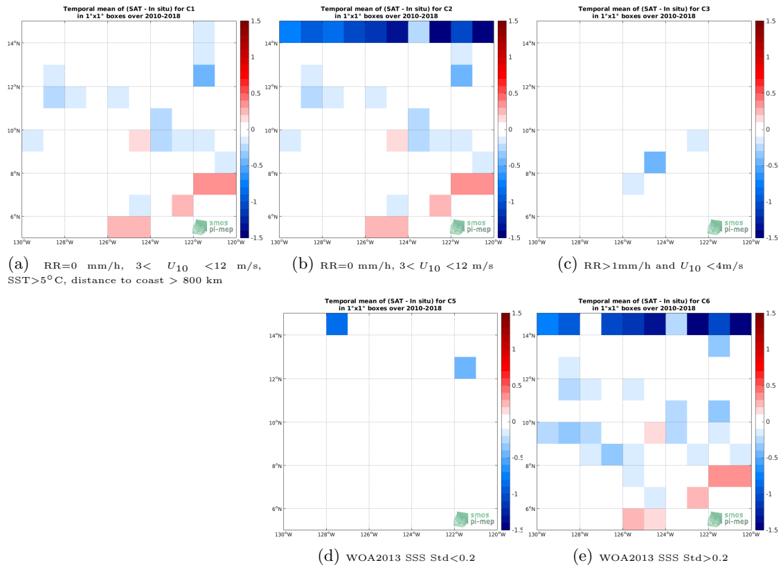
Figure 12: Temporal mean gridded over spatial boxes of size 1^\circ \times 1^\circ of \Delta SSS (CCI L4 Merged-OI v1.8 - 7-day running (ESA) - TSG-SAMOS) for 5 different subdatasets corresponding to: RR=0 mm/h, 3 < U_{10} < 12 m/s, SST > 5^\circ C , distance to coast > 800 km (a), RR=0 mm/h, 3 < U_{10} < 12 m/s (b), RR > 1 mm/h and U_{10} < 4 m/s (c), WOA2013 SSS Std < 0.2 (d), WOA2013 SSS Std > 0.2 (e).
