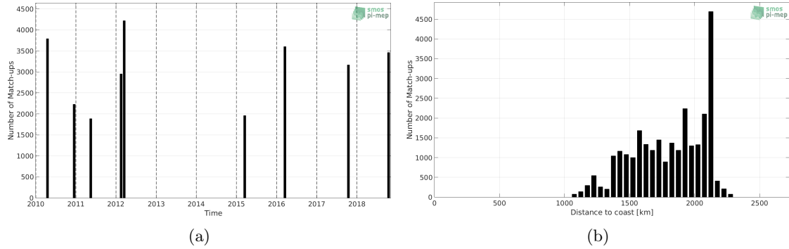
Figure 1: Number of match-ups between TSG-SAMOS and CCI L4 Merged-OI v1.8 - 7-day running (ESA) SSS as a function of time (a) and as function of the distance to coast (b) over the SPURS 2 Pi-MEP region and for the full satellite product period.
