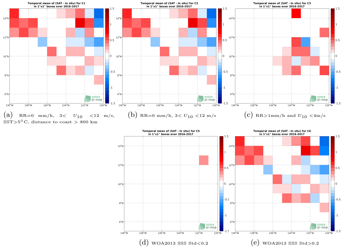
Figure 11: Temporal mean gridded over spatial boxes of size 1^\circ \times 1^\circ of \Delta SSS (CCI-L4-ESA-MERGED-OI-V1.8-7DAY-RUNNING - Surface drifters) for 5 different subdatasets corresponding to: RR=0 mm/h, 3 < U_{10} < 12 m/s, SST > 5^\circ C , distance to coast > 800 km (a), RR=0 mm/h, 3 < U_{10} < 12 m/s (b), RR > 1 mm/h and U_{10} < 4 m/s (c), WOA2013 SSS Std < 0.2 (d), WOA2013 SSS Std > 0.2 (e).
