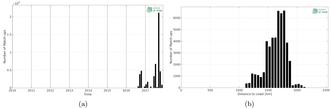
Figure 1: Number of match-ups between Surface drifters and CCI-L4-ESA-MERGED-OI-V1.8-7DAY-RUNNING SSS as a function of time (a) and as function of the distance to coast (b) over the SPURS 2 Pi-MEP region and for the full satellite product period.
