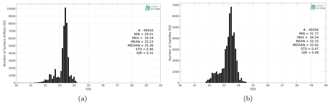
Figure 2: Histograms of SSS from Surface drifters (a) and CCI-L4-ESA-MERGED-OI-V1.8-7DAY-RUNNING (b) considering all match-up pairs per bins of 0.1 over the SPURS 2 Pi-MEP region and for the full satellite product period.
