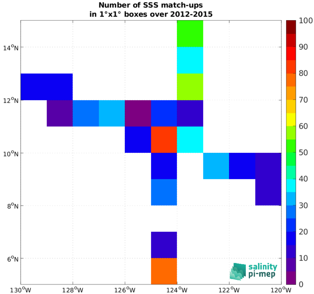
Figure 5: Number of SSS match-ups between TSG (SAMOS) SSS and the Aquarius SSS L4 OI v5 - Weekly (IPRC) SSS product for the SPURS 2 Pi-MEP region over 1^\circ \times 1^\circ boxes and for the full satellite product period.
