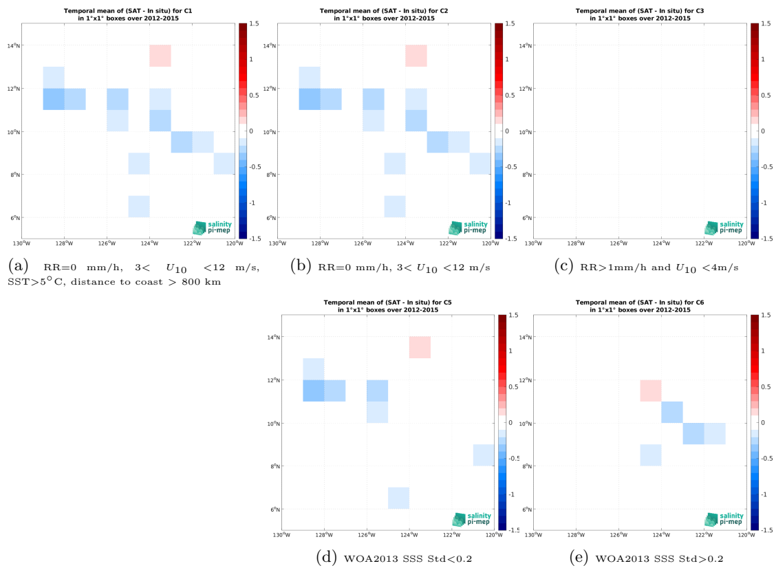
Figure 14: Temporal mean gridded over spatial boxes of size 1^\circ \times 1^\circ of \Delta SSS (Aquarius SSS L4 OI v5 - Weekly (IPRC) - TSG (SAMOS)) for 5 different subdatasets corresponding to:RR=0 mm/h, 3 < U_{10} < 12 m/s, SST >5^\circ\text{C} , distance to coast > 800 km (a), RR=0 mm/h, 3 < U_{10} < 12 m/s (b), RR >1 mm/h and U_{10} < 4 m/s (c), WOA2013 SSS Std <0.2 (d), WOA2013 SSS Std >0.2 (e).
