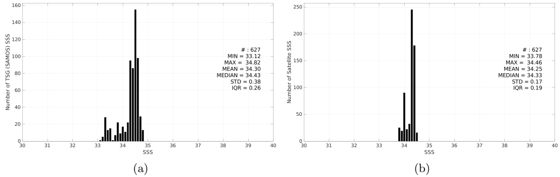
Figure 3: Histograms of SSS from TSG (SAMOS) (a) and Aquarius SSS L4 OI v5 - Weekly (IPRC) (b) considering all match-up pairs per bins of 0.1 over the SPURS 2 Pi-MEP region and for the full satellite product period.
