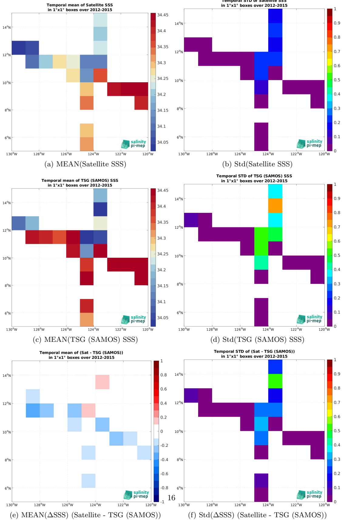
Figure 7: Temporal mean (left) and Std (right) of SSS from Aquarius SSS L4 OI v5 - Weekly (IPRC) (top), TSG (SAMOS) (middle), and of \Delta SSS (Satellite - TSG (SAMOS)). Only match-up pairs are used to generate these maps.
