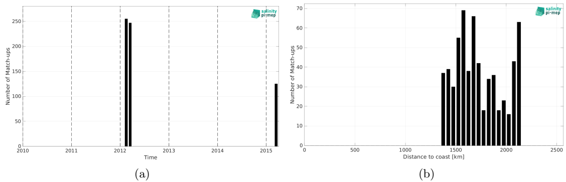
Figure 2: Number of match-ups between TSG (SAMOS) and Aquarius SSS L4 OI v5 - Weekly (IPRC) SSS as a function of time (a) and as function of the distance to coast (b) over the SPURS 2 Pi-MEP region and for the full satellite product period.
