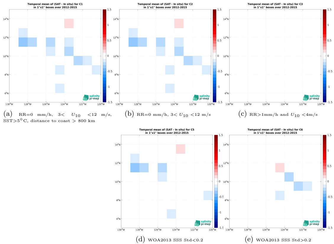
Figure 14: Temporal mean salinity gridded over spatial boxes of size 1^\circ \times 1^\circ of \Delta SSS (Aquarius SSS L4 OI v5 - Weekly (IPRC) - TSG (SAMOS)) for 5 different subdatasets corresponding to:RR=0 mm/h, 3 < U_{10} < 12 m/s, SST>5°C, distance to coast > 800 km (a), RR=0 mm/h, 3 < U_{10} < 12 m/s (b), RR>1mm/h and U_{10} < 4 m/s (c), WOA2013 SSS Std<0.2 (d), WOA2013 SSS Std>0.2 (e).
