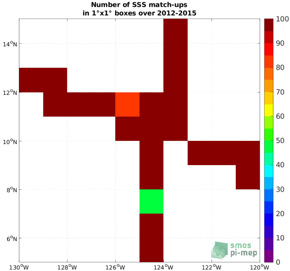
Figure 4: Number of SSS match-ups between TSG (SAMOS) SSS and the Aquarius SSS L4 OI v5 - Weekly (IPRC) SSS product for the SPURS 2 Pi-MEP region over 1^\circ \times 1^\circ boxes and for the full satellite product period.
