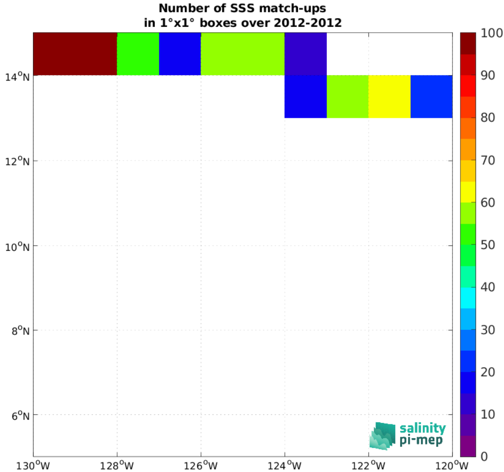
Figure 5: Number of SSS match-ups between TSG (GOSUD-Research-vessel) SSS and the Aquarius SSS L4 OI v5 - Weekly (IPRC) SSS product for the SPURS 2 Pi-MEP region over 1^\circ \times 1^\circ boxes and for the full satellite product period.
