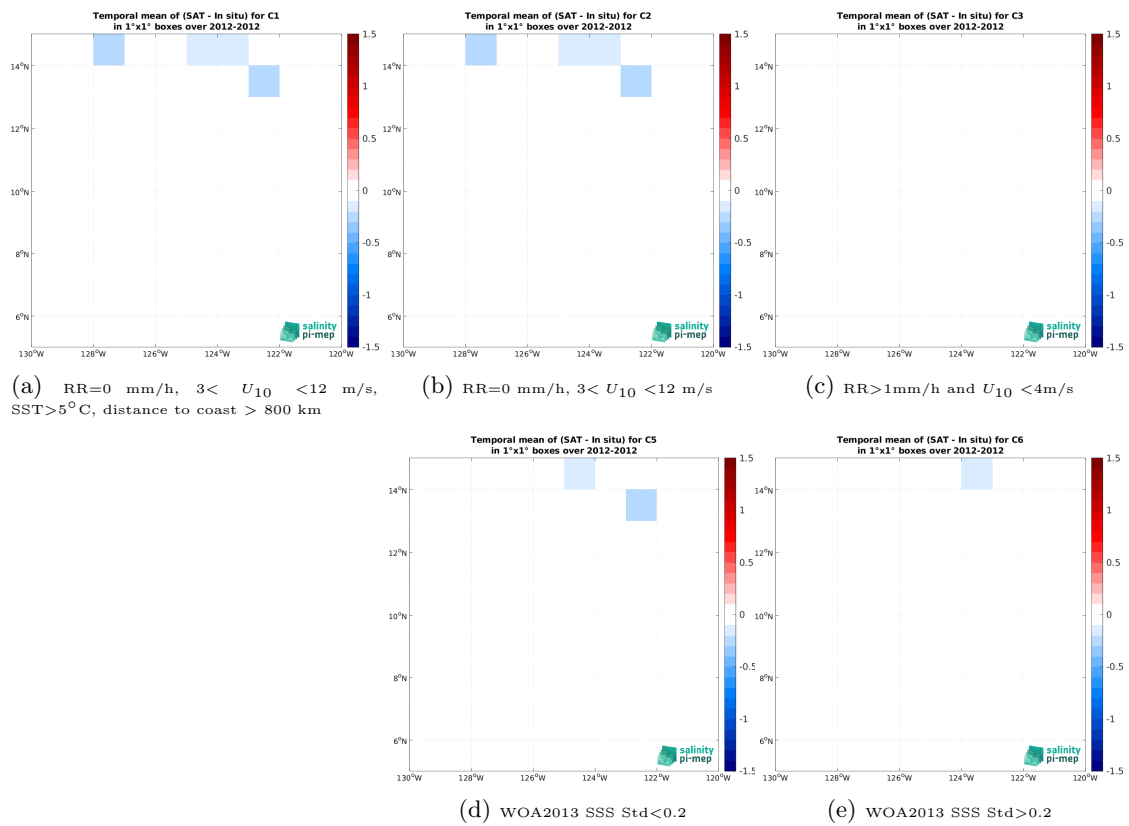
Figure 14: Temporal mean gridded over spatial boxes of size 1^\circ \times 1^\circ of \Delta SSS (Aquarius SSS L4 OI v5 - Weekly (IPRC) - TSG (GOSUD-Research-vessel)) for 5 different subdatasets corresponding to:RR=0 mm/h, 3 < U_{10} < 12 m/s, SST >5^\circ\text{C} , distance to coast > 800 km (a), RR=0 mm/h, 3 < U_{10} < 12 m/s (b), RR >1 mm/h and U_{10} < 4 m/s (c), WOA2013 SSS Std <0.2 (d), WOA2013 SSS Std >0.2 (e).
