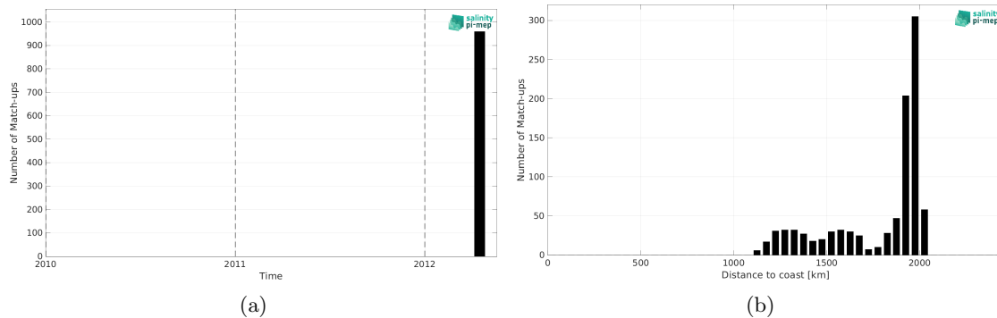
Figure 2: Number of match-ups between TSG (GOSUD-Research-vessel) and Aquarius SSS L4 OI v5 - Weekly (IPRC) SSS as a function of time (a) and as function of the distance to coast (b) over the SPURS 2 Pi-MEP region and for the full satellite product period.
