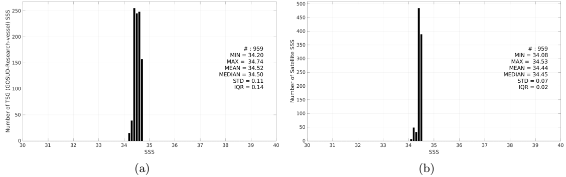
Figure 3: Histograms of SSS from TSG (GOSUD-Research-vessel) (a) and Aquarius SSS L4 OI v5 - Weekly (IPRC) (b) considering all match-up pairs per bins of 0.1 over the SPURS 2 Pi-MEP region and for the full satellite product period.
