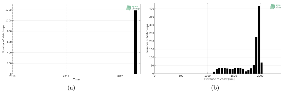
Figure 1: Number of match-ups between TSG-GOSUD-Research-vessel and Aquarius-L4-IPRC-V5-WEEKLY SSS as a function of time (a) and as function of the distance to coast (b) over the SPURS 2 Pi-MEP region and for the full satellite product period.
