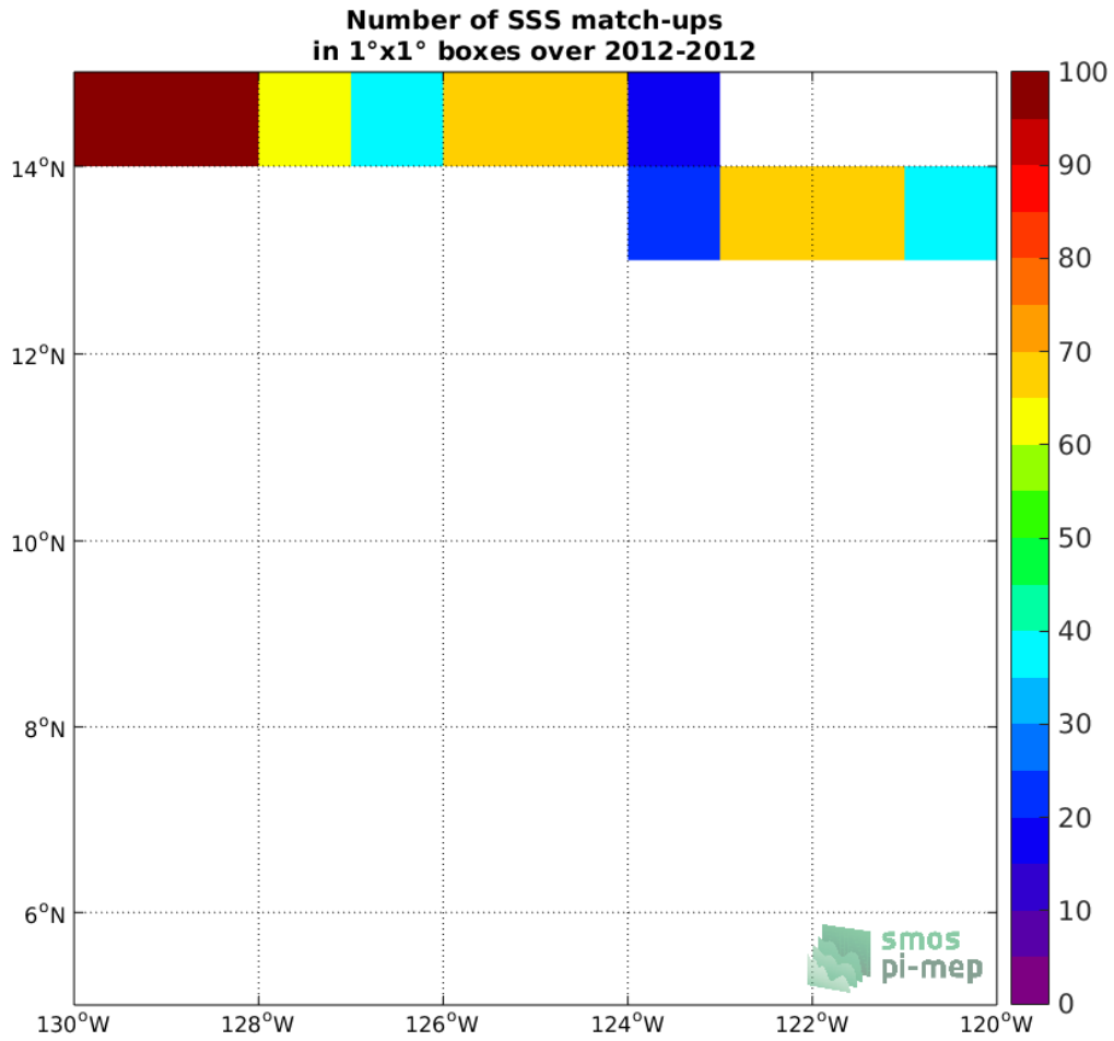
Figure 4: Number of SSS match-ups between TSG-GOSUD-Research-vessel SSS and the Aquarius-L4-IPRC-V5-WEEKLY SSS product for the SPURS 2 Pi-MEP region over 1°x1° boxes and for the full satellite product period.
