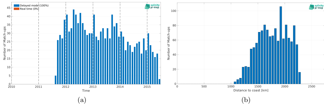
Figure 2: Number of match-ups between Argo and Aquarius SSS L4 OI v5 - Weekly (IPRC) SSS as a function of time (a) and as function of the distance to coast (b) over the SPURS 2 Pi-MEP region and for the full satellite product period.
