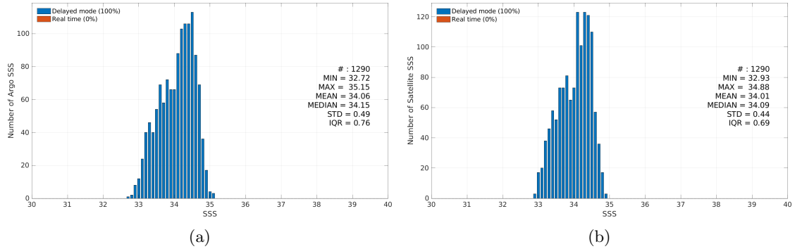
Figure 3: Histograms of SSS from Argo (a) and Aquarius SSS L4 OI v5 - Monthly (IPRC) (b) considering all match-up pairs per bins of 0.1 over the SPURS 2 Pi-MEP region and for the full satellite product period.
