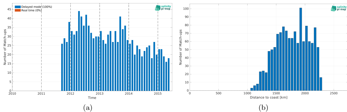
Figure 2: Number of match-ups between Argo and Aquarius SSS L4 OI v5 - Monthly (IPRC) SSS as a function of time (a) and as function of the distance to coast (b) over the SPURS 2 Pi-MEP region and for the full satellite product period.
