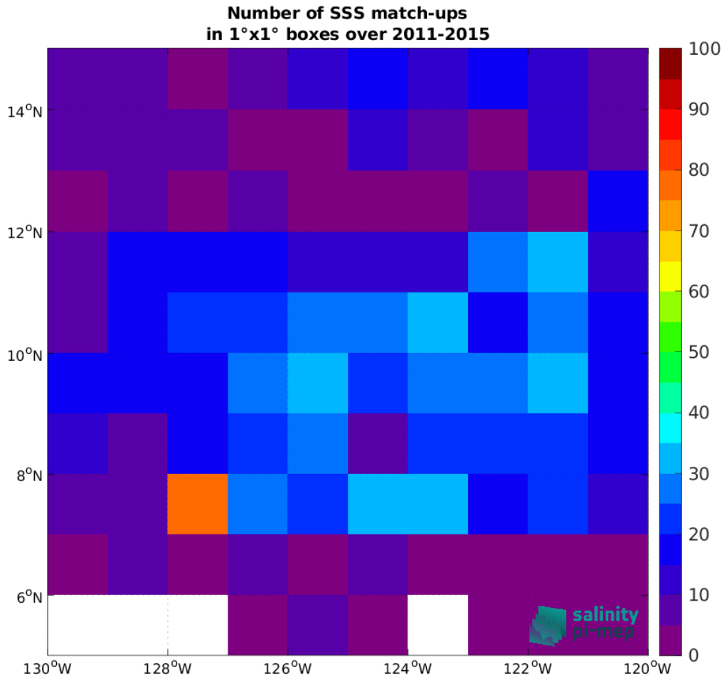
Figure 5: Number of SSS match-ups between Argo SSS and the Aquarius SSS L4 OI v5 - Monthly (IPRC) SSS product for the SPURS 2 Pi-MEP region over 1^\circ \times 1^\circ boxes and for the full satellite product period.
