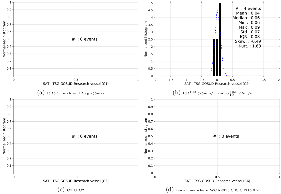
Figure 13: Normalized histogram of \Delta\text{SSS} (Aquarius-L4-IPRC-V4-WEEKLY - TSG-GOSUD-Research-vessel) for 6 different subdatasets corresponding to: RR > 1\text{mm/h} and U_{10} < 5\text{m/s} (a), RR^{10d} > 5\text{mm/h} and U_{10}^{10d} < 5\text{m/s} (b), C1 \cup C2 (c), Locations where WOA2013 SSS STD > 0.2 (d).
