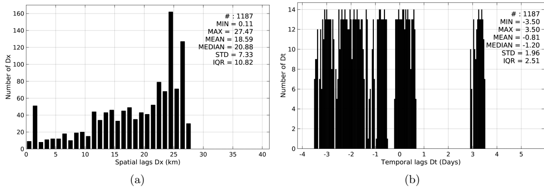
Figure 5: Histograms of the spatial (a) and temporal (b) lags between the time of the TSG-GOSUD-Research-vessel measurements and the date of the corresponding Aquarius-L4-IPRC-V4-WEEKLY SSS product.
