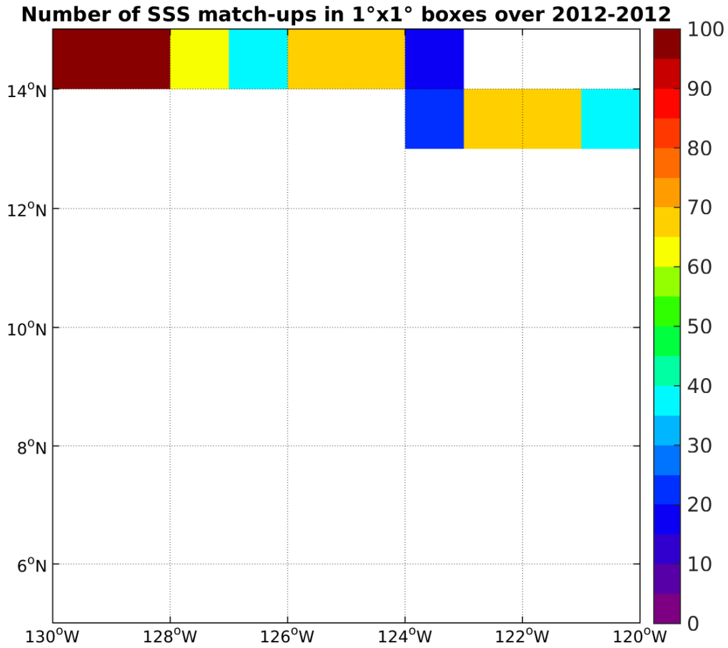
Figure 4: Number of SSS match-ups between TSG-GOSUD-Research-vessel SSS and the Aquarius-L4-IPRC-V4-WEEKLY SSS product for the SPURS 2 Pi-MEP region over 1°x1° boxes and for the full satellite product period.
