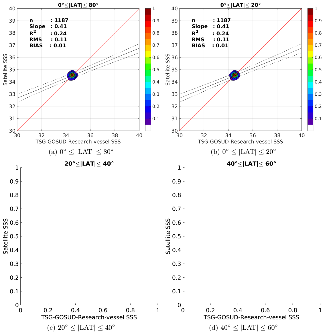
Figure 9: Contour maps of the concentration of Aquarius-L4-IPRC-V4-WEEKLY SSS (y-axis) versus TSG-GOSUD-Research-vessel SSS (x-axis) at match-up pairs for different latitude bands. For each plot, the red line shows x=y . The black thin and dashed lines indicate a linear fit through the data cloud and the \pm 95\% confidence levels, respectively. The number match-up pairs n , the slope and R^2 coefficient of the linear fit, the root mean square (RMS) and the mean bias between satellite and in situ data are indicated for each latitude band in each plots.
