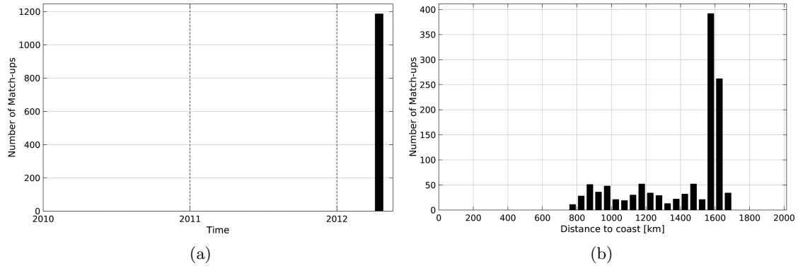
Figure 1: Number of match-ups between TSG-GOSUD-Research-vessel and Aquarius-L4-IPRC-V4-WEEKLY SSS as a function of time (a) and as function of the distance to coast (b) over the SPURS 2 Pi-MEP region and for the full satellite product period.
