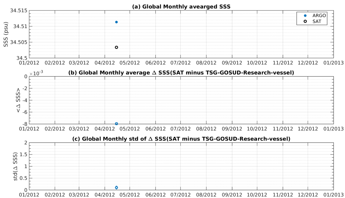
Figure 7: Time series of the monthly averaged mean SSS (top), mean \Delta SSS (Satellite - TSG-GOSUD-Research-vessel) and STD of \Delta SSS (Satellite - TSG-GOSUD-Research-vessel) over the SPURS 2 Pi-MEP region considering all match-ups collected by the Pi-MEP platform.
