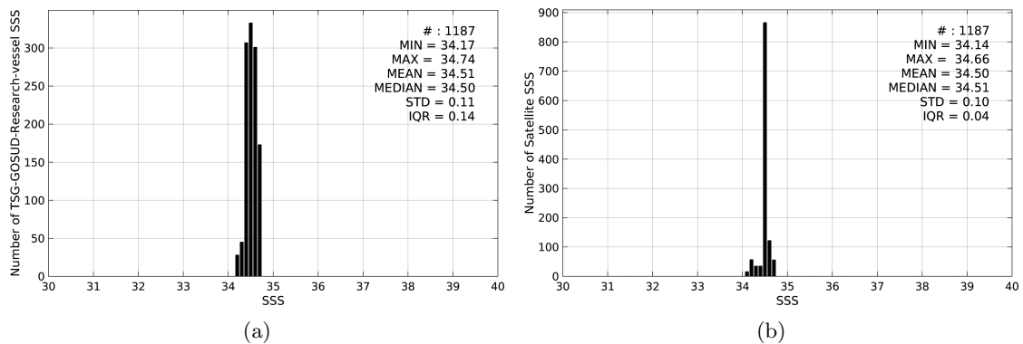
Figure 2: Histograms of SSS from TSG-GOSUD-Research-vessel (a) and Aquarius-L4-IPRC-V4-WEEKLY (b) considering all match-up pairs per bins of 0.1 over the SPURS 2 Pi-MEP region and for the full satellite product period.
