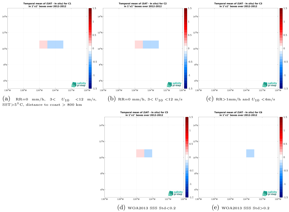
Figure 14: Temporal mean gridded over spatial boxes of size 1^\circ \times 1^\circ of \Delta SSS (Aquarius SSS L3 OR v5 - 7-Day running (NASA-GSFC) - TSG (SAMOS)) for 5 different subdatasets corresponding to:RR=0 mm/h, 3 < U_{10} < 12 m/s, SST>5°C, distance to coast > 800 km (a), RR=0 mm/h, 3 < U_{10} < 12 m/s (b), RR>1mm/h and U_{10} < 4 m/s (c), WOA2013 SSS Std<0.2 (d), WOA2013 SSS Std>0.2 (e).
