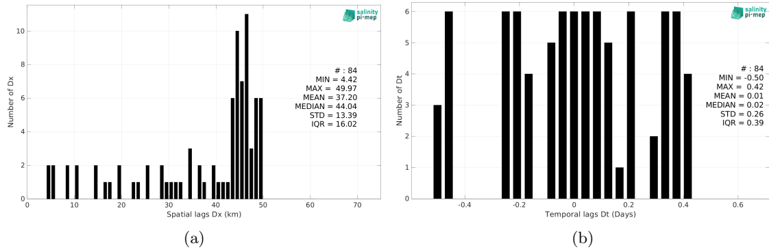
Figure 6: Histograms of the spatial (a) and temporal (b) lags between the location/time of the TSG (SAMOS) measurement and the date of the corresponding Aquarius SSS L3 OR v5 - 7-Day running (NASA-GSFC) SSS pixel.
