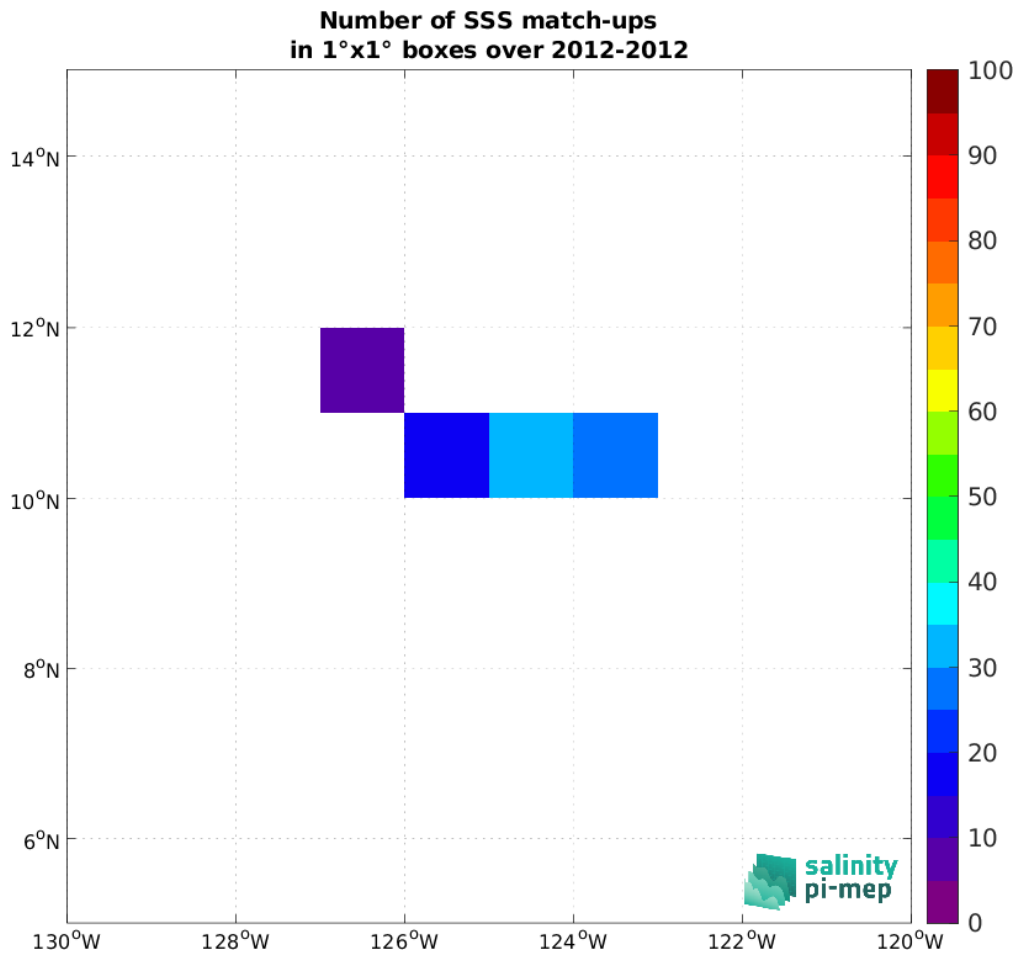
Figure 5: Number of SSS match-ups between TSG (SAMOS) SSS and the Aquarius SSS L3 OR v5 - 7-Day running (NASA-GSFC) SSS product for the SPURS 2 Pi-MEP region over 1°x1° boxes and for the full satellite product period.
