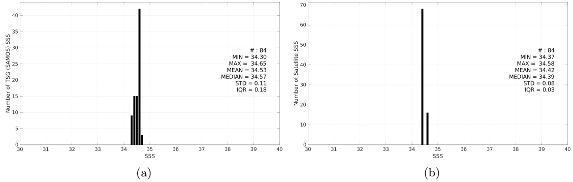
Figure 3: Histograms of SSS from TSG (SAMOS) (a) and Aquarius SSS L3 OR v5 - 7-Day running (NASA-GSFC) (b) considering all match-up pairs per bins of 0.1 over the SPURS 2 Pi-MEP region and for the full satellite product period.
