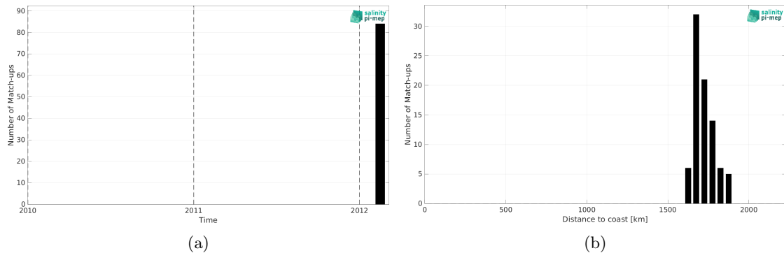
Figure 2: Number of match-ups between TSG (SAMOS) and Aquarius SSS L3 OR v5 - 7-Day running (NASA-GSFC) SSS as a function of time (a) and as function of the distance to coast (b) over the SPURS 2 Pi-MEP region and for the full satellite product period.
