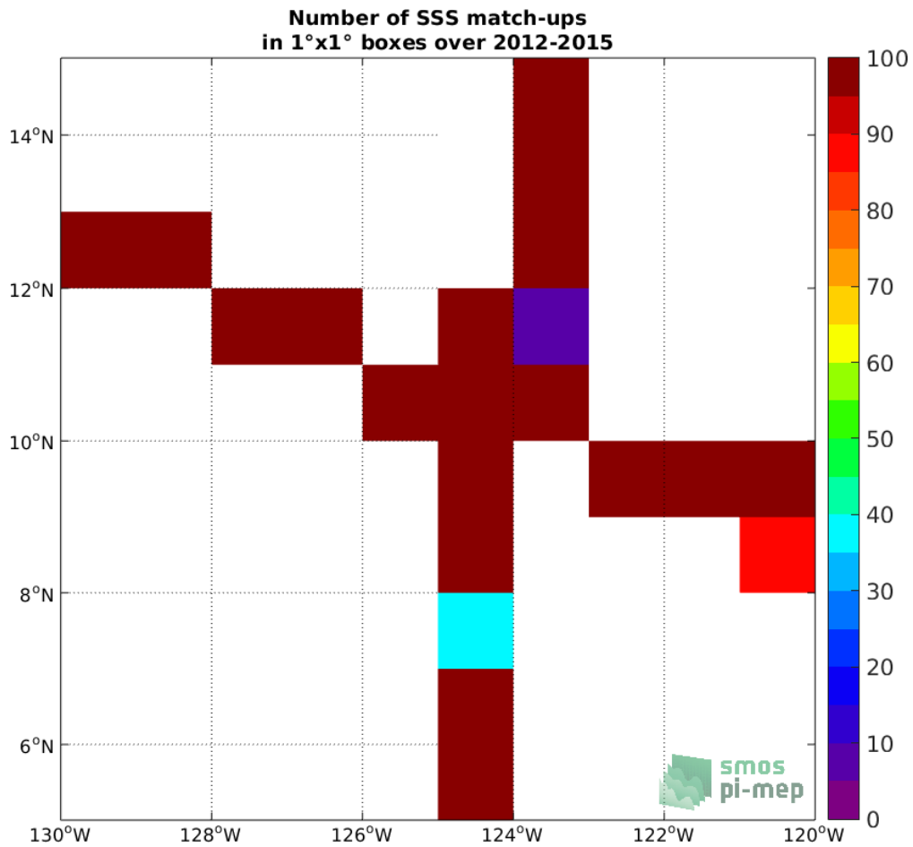
Figure 4: Number of SSS match-ups between TSG (SAMOS) SSS and the Aquarius SSS L3 OR v5 - 7-Day running (NASA-GSFC) SSS product for the SPURS 2 Pi-MEP region over 1°x1° boxes and for the full satellite product period.
