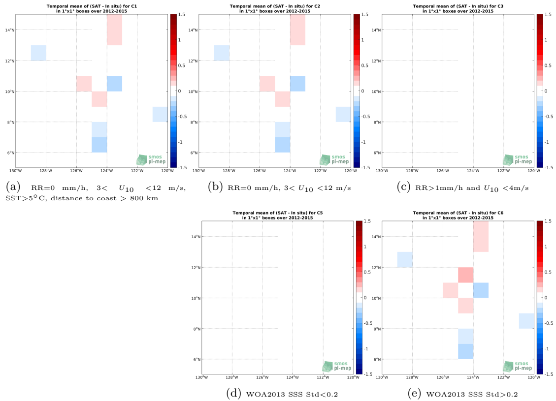
Figure 12: Temporal mean gridded over spatial boxes of size 1^\circ \times 1^\circ of \Delta\text{SSS} (Aquarius SSS L3 OR v5 - 7-Day running (NASA-GSFC) - TSG (SAMOS)) for 5 different subdatasets corresponding to:RR=0 mm/h, 3 < U_{10} < 12 m/s, SST >5^\circ\text{C} , distance to coast > 800 km (a), RR=0 mm/h, 3 < U_{10} < 12 m/s (b), RR >1 mm/h and U_{10} < 4 m/s (c), WOA2013 SSS Std <0.2 (d), WOA2013 SSS Std >0.2 (e).
