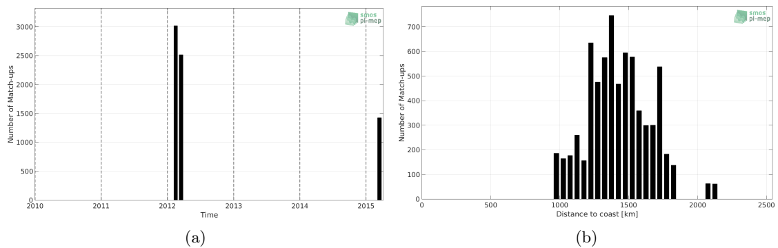
Figure 1: Number of match-ups between TSG-SAMOS and Aquarius-L3-OR-V5-7DAY-RUNNING-1DEG SSS as a function of time (a) and as function of the distance to coast (b) over the SPURS 2 Pi-MEP region and for the full satellite product period.
