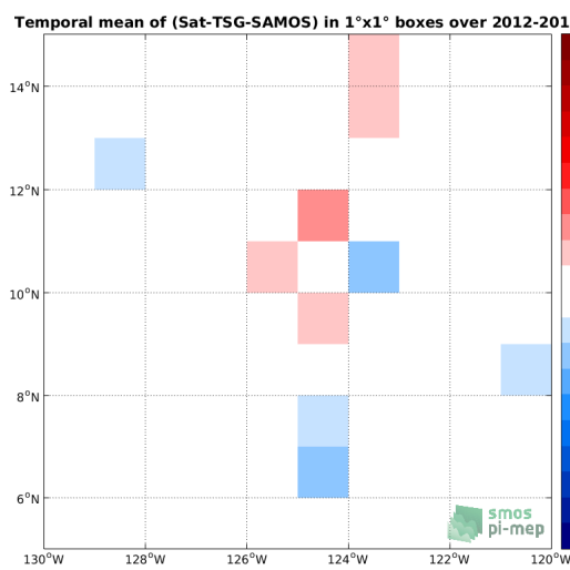
(e) MEAN( \Delta SSS) (Satellite - TSG-SAMOS) 21
