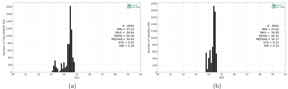
Figure 2: Histograms of SSS from TSG-SAMOS (a) and Aquarius-L3-OR-V5-7DAY-RUNNING-1DEG (b) considering all match-up pairs per bins of 0.1 over the SPURS 2 Pi-MEP region and for the full satellite product period.
