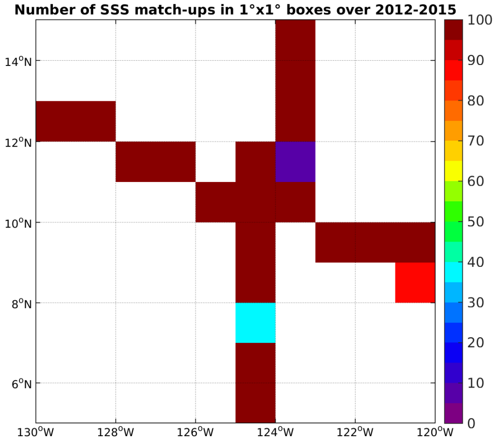
Figure 4: Number of SSS match-ups between TSG-SAMOS SSS and the Aquarius-L3-OR-V5-7DAY-RUNNING-1DEG SSS product for the SPURS 2 Pi-MEP region over 1°x1° boxes and for the full satellite product period.
