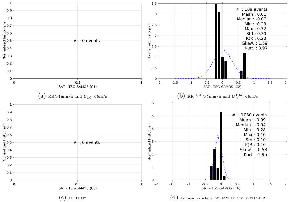
Figure 13: Normalized histogram of \Delta\text{SSS} (Aquarius-L3-OR-V5-7DAY-RUNNING-1DEG - TSG-SAMOS) for 6 different subdatasets corresponding to: RR > 1\text{mm/h} and U_{10} < 5\text{m/s} (a), RR^{10d} > 5\text{mm/h} and U_{10}^{10d} < 5\text{m/s} (b), C1 U C2 (c), Locations where WOA2013 SSS STD > 0.2 (d).
