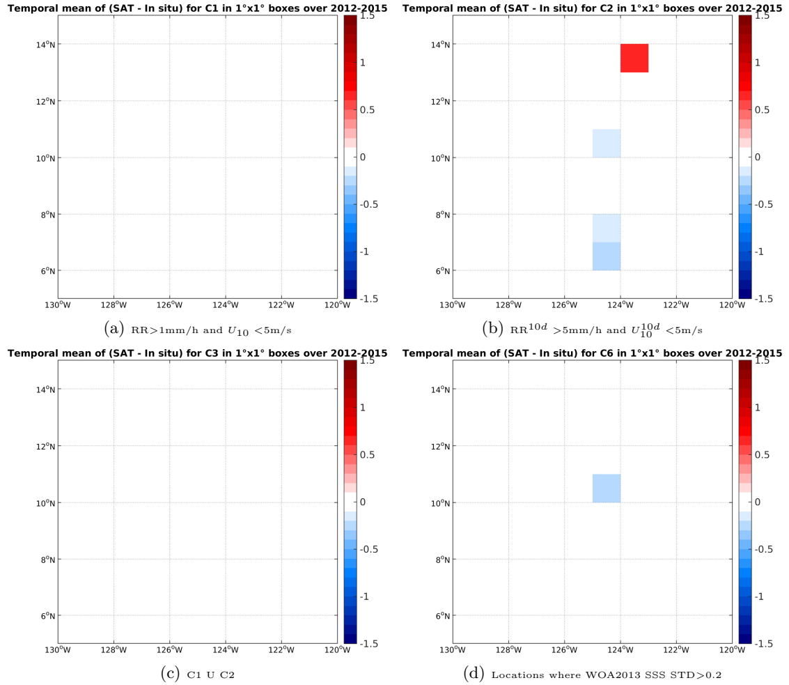
Figure 12: Temporal mean gridded over spatial boxes of size 1^\circ \times 1^\circ of \Delta SSS (Aquarius-L3-OR-V5-7DAY-RUNNING-1DEG - TSG-SAMOS) for 4 different subdatasets corresponding to: RR > 1\text{mm/h} and U_{10} < 5\text{m/s} (a), RR^{10d} > 5\text{mm/h} and U_{10}^{10d} < 5\text{m/s} (b), C1 U C2 (c), Locations where WOA2013 SSS STD > 0.2 (d).
