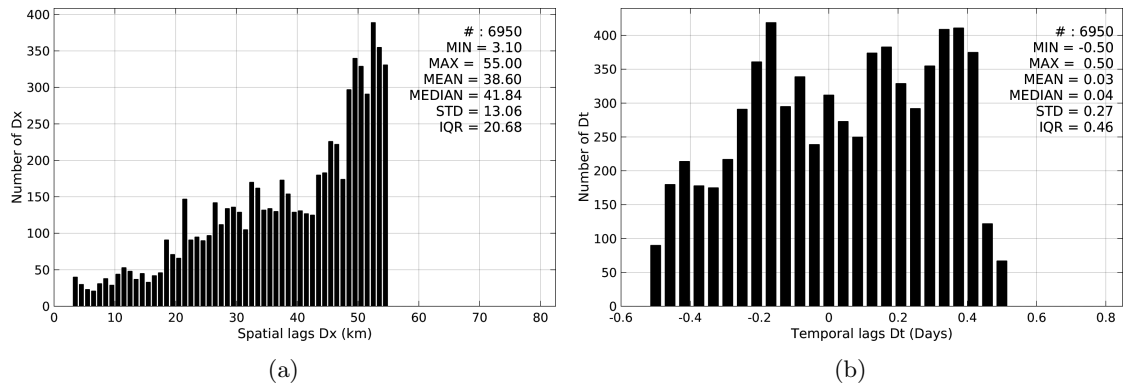
Figure 5: Histograms of the spatial (a) and temporal (b) lags between the time of the TSG-SAMOS measurements and the date of the corresponding Aquarius-L3-OR-V5-7DAY-RUNNING-1DEG SSS product.
