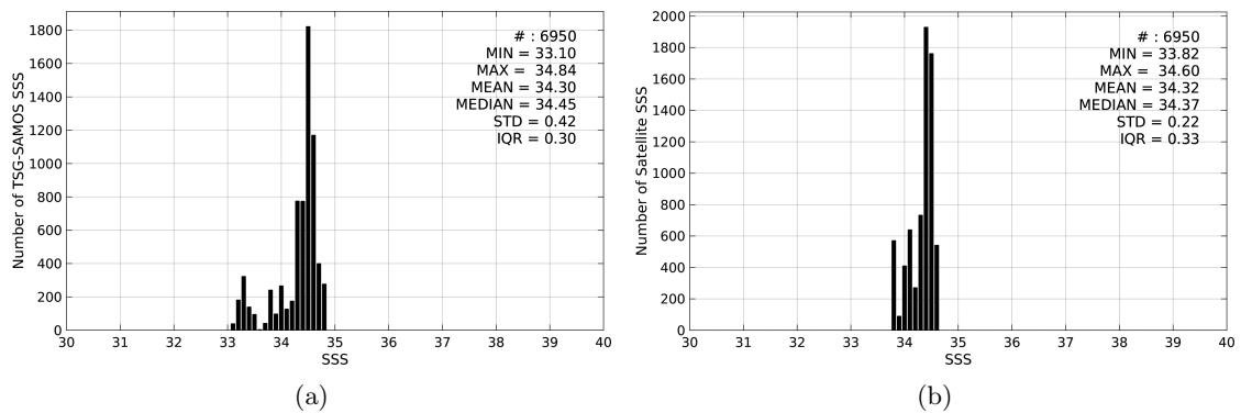
Figure 2: Histograms of SSS from TSG-SAMOS (a) and Aquarius-L3-OR-V5-7DAY-RUNNING-1DEG (b) considering all match-up pairs per bins of 0.1 over the SPURS 2 Pi-MEP region and for the full satellite product period.
