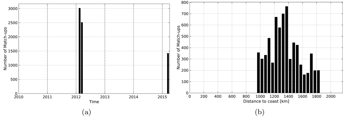
Figure 1: Number of match-ups between TSG-SAMOS and Aquarius-L3-OR-V5-7DAY-RUNNING-1DEG SSS as a function of time (a) and as function of the distance to coast (b) over the SPURS 2 Pi-MEP region and for the full satellite product period.
